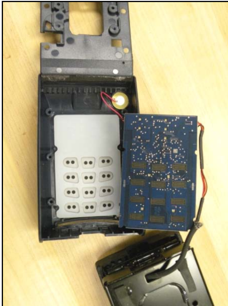
Photograph 13: Board Removed
