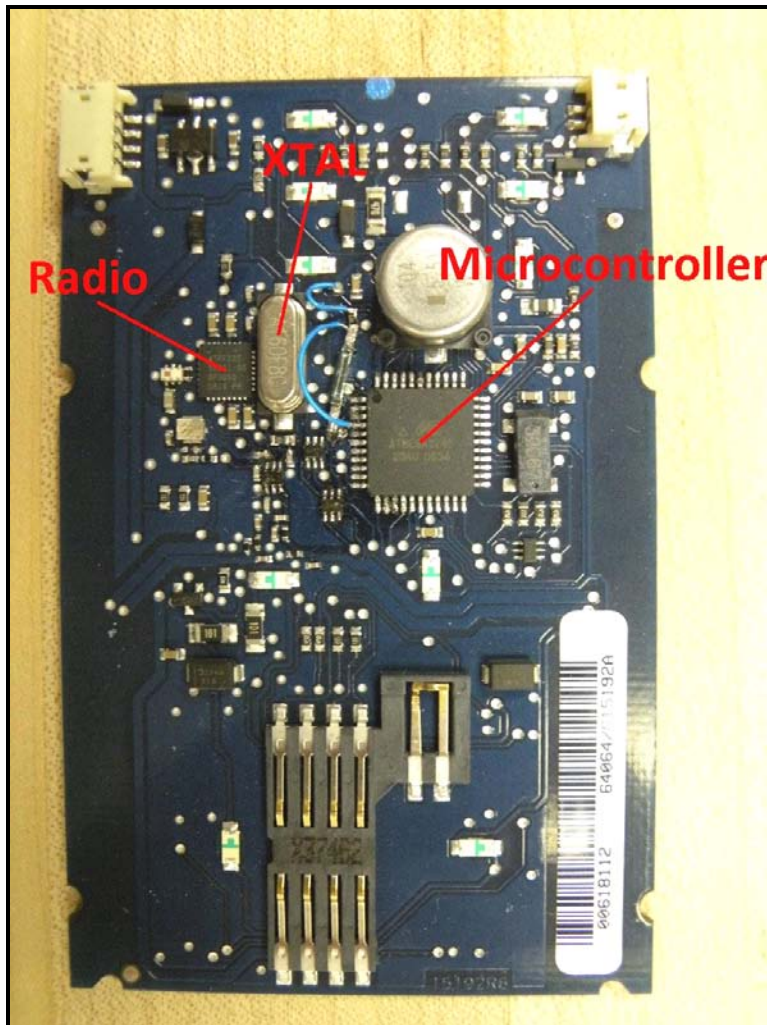
Photograph 15: PCB Back View
