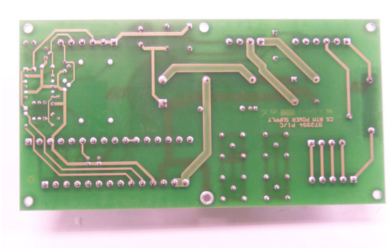
Figure 6.1 CS RTM POWER SUPPLY 972911A1 Bottom View
