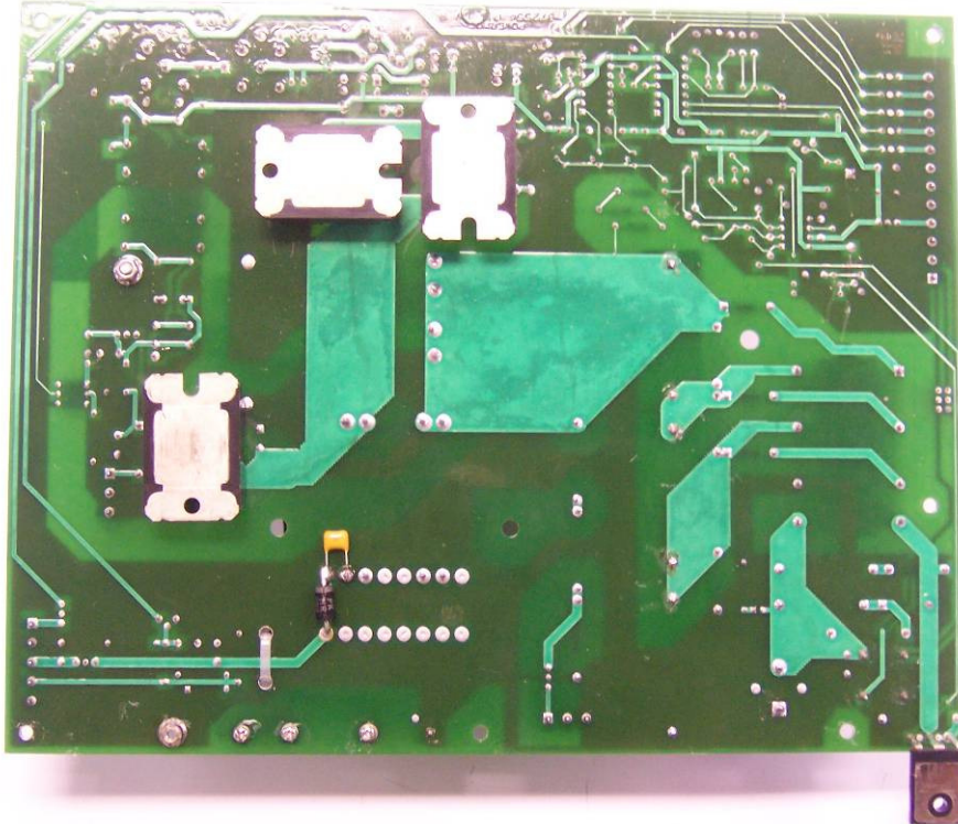
Figure 2.1 POWER MOS 972551A3 Bottom View
