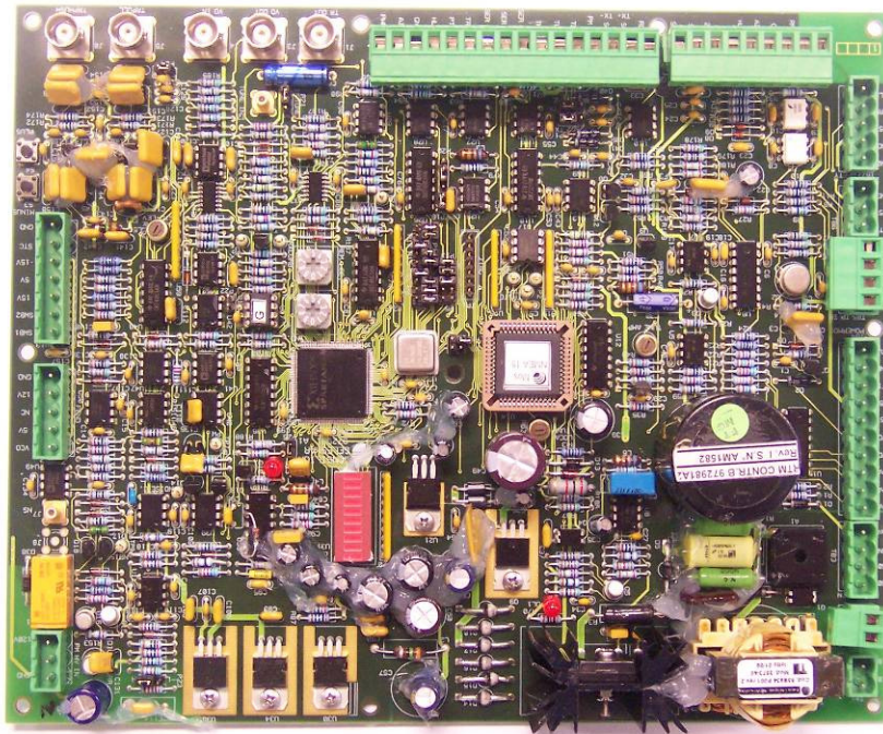
Figure 3.0 RTM CONTROL B 972981A2 Top View
