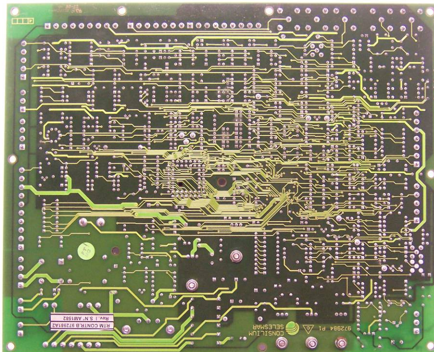
Figure 3.1 RTM CONTROL B 972981A2 Bottom View
