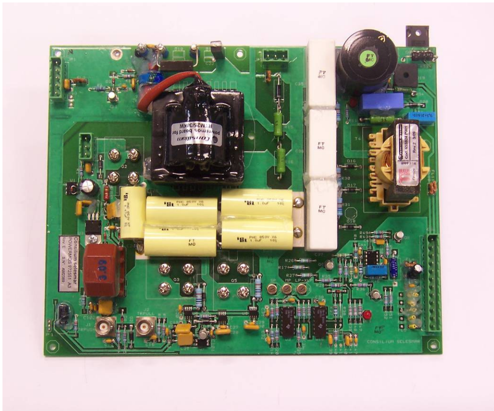
Figure 2.0 POWER MOS 972551A3 Top View
