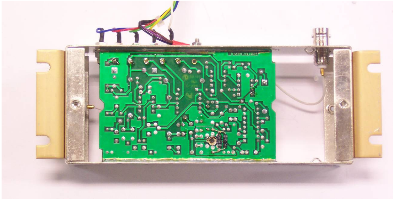
Figure 2.1 NIFB Assy 303186A2 Bottom View
