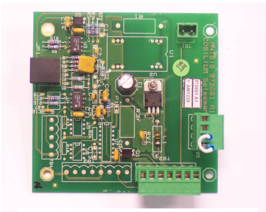
Figure 4.0 ANTSIG 972661A1 Top View
