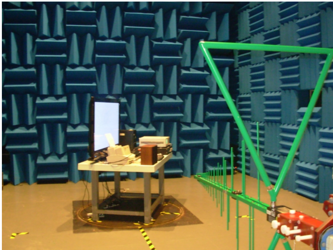
SETUP WITH MAXIMUM DETECTED EMISSION AT VERTICAL POLARIZATION (HDMI 800*600@60Hz)
