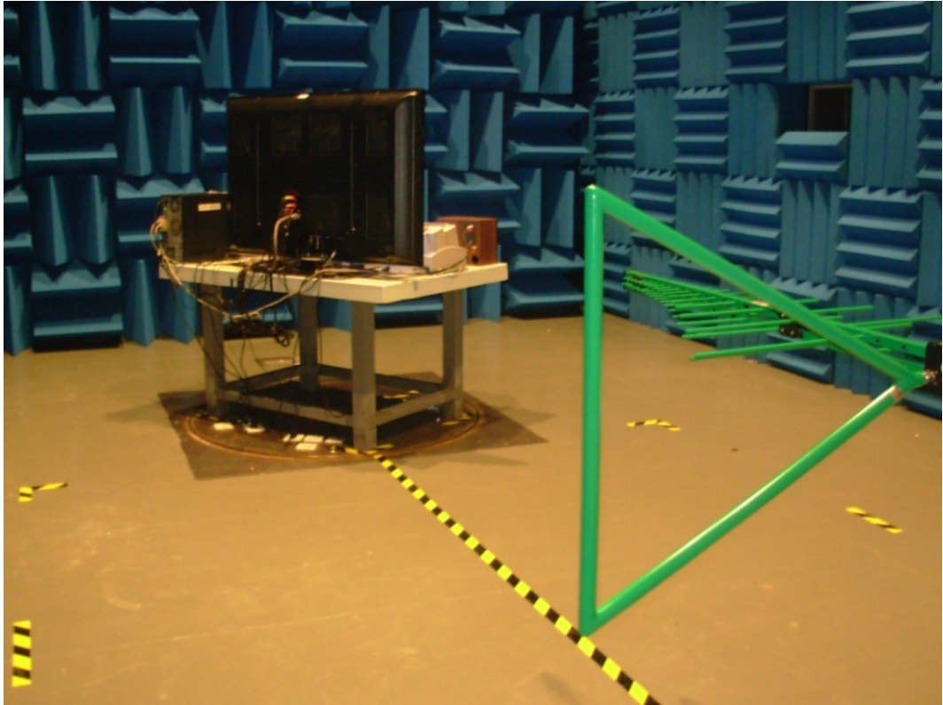
SETUP WITH MAXIMUM DETECTED EMISSION AT HORIZONTAL POLARIZATION (HDMI 800*600@60Hz)
