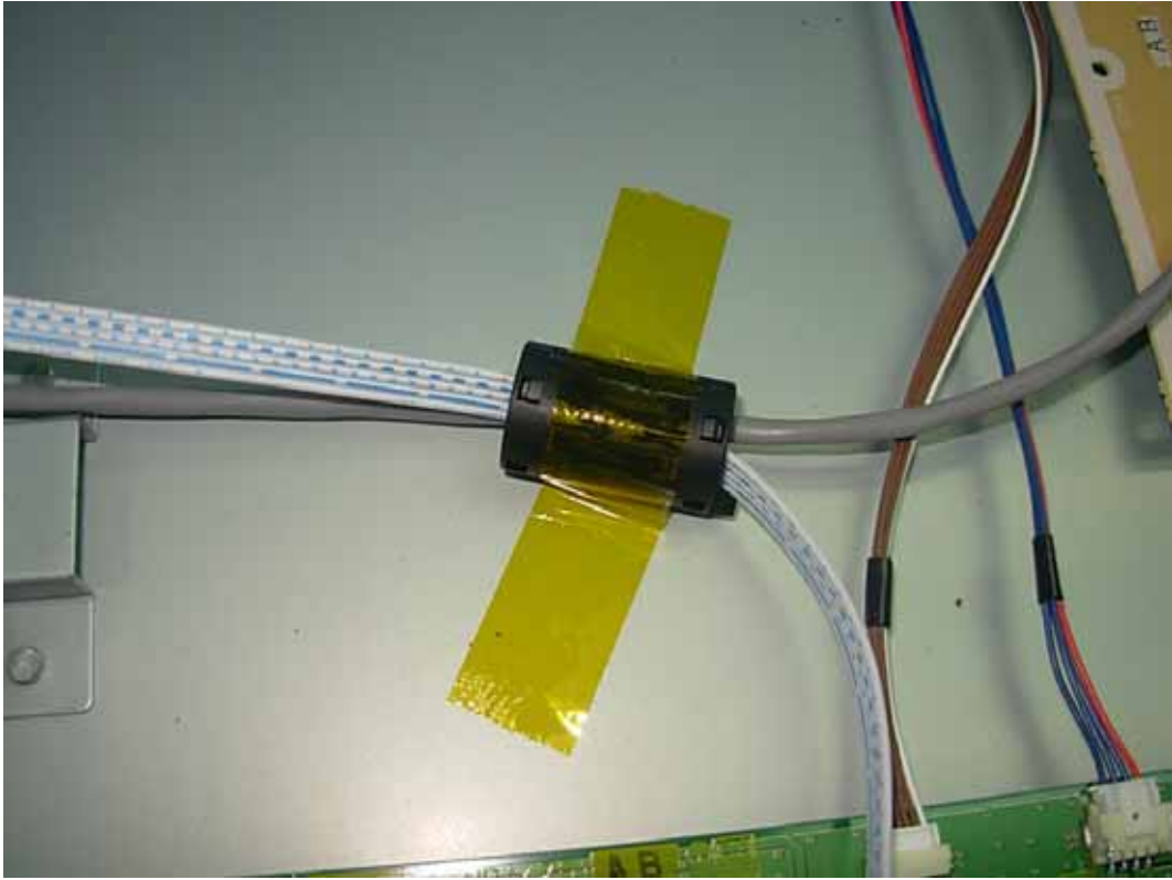
FIGURE 31 PDP TV (M/N: ELPCFT501) DEBUG#2
