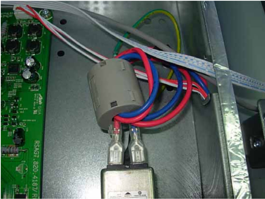
FIGURE 30 PDP TV (M/N: ELPCFT501) DEBUG#1
