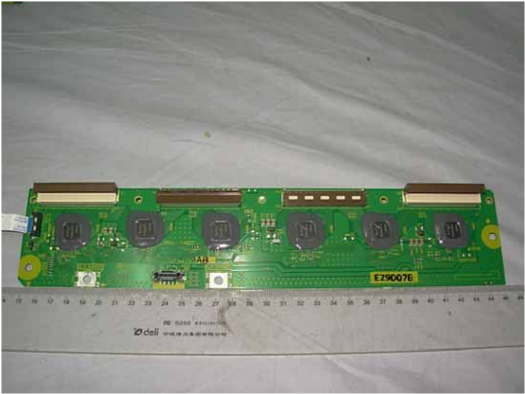
FIGURE 22 PDP TV (M/N: ELPCFT501) H.V. BOARD#2 (COMPONENT SIDE)
