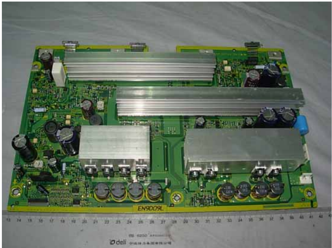
FIGURE 16 PDP TV (M/N: ELPCFT501) TPVSUS BOARD#1 (COMPONENT SIDE)
