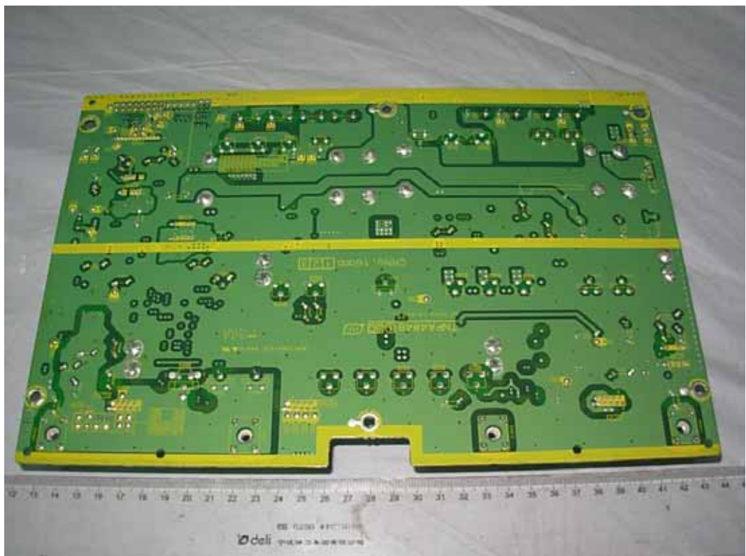
FIGURE 17 PDP TV (M/N: ELPCFT501) TPVSUS BOARD#1 (SOLDERED SIDE)
