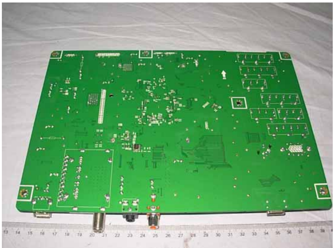
FIGURE 6 PDP TV (M/N: ELPCFT501) MAIN BOARD (SOLDERED SIDE)
