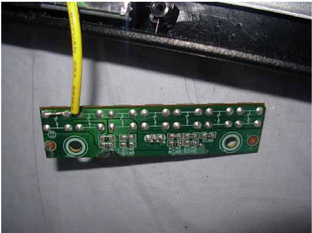
FIGURE 12 PDP TV (M/N: ELPCFT501) KEY BOARD (SOLDERED SIDE)
