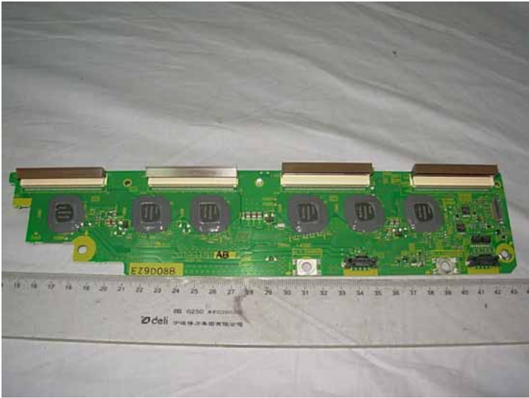
FIGURE 20 PDP TV (M/N: ELPCFT501) H.V. BOARD#1 (COMPONENT SIDE)
