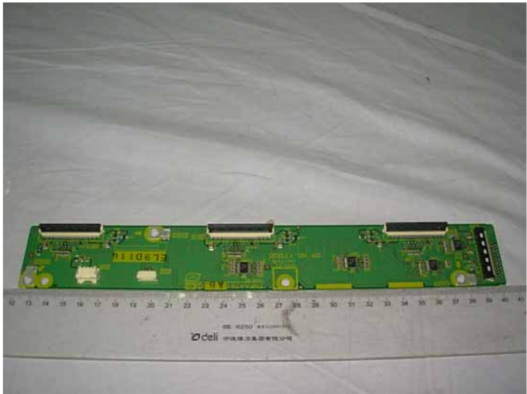
FIGURE 26 PDP TV (M/N: ELPCFT501) RT CONTROL BOARD#2 (COMPONENT SIDE)
