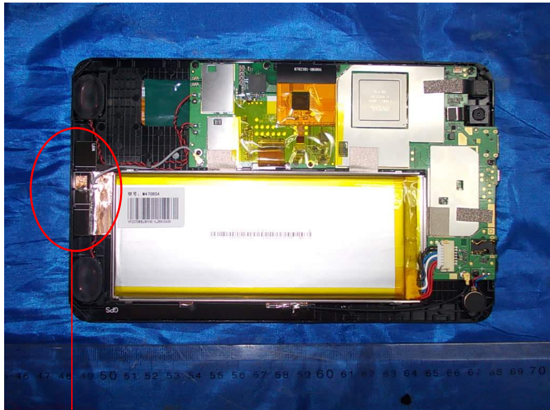
FIGURE 5 SERO 7 PRO (M/N: M470BSA) COVER REMOVED (INSIDE VIEW)
