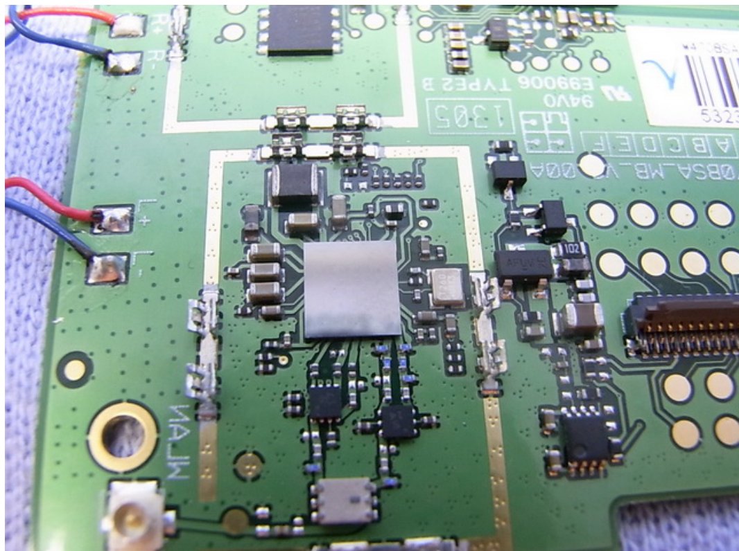
FIGURE 12 SERO 7 PRO (M/N: M470BSA) RF MODULE ON MAIN BOARD
