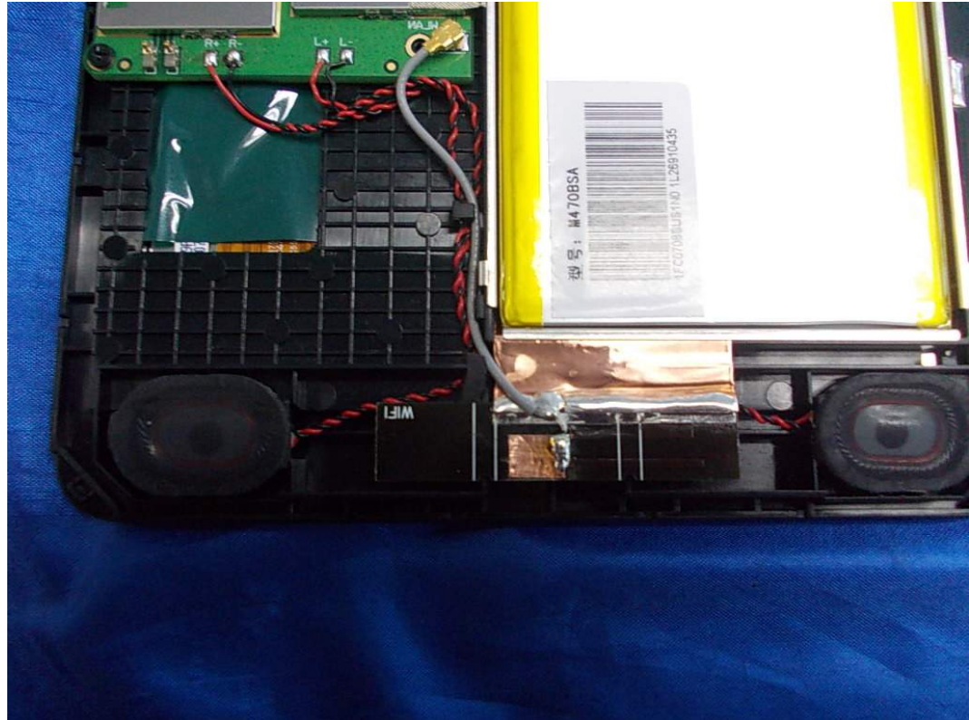
FIGURE 13 SERO 7 PRO (M/N: M470BSA) RF ANTENNA
