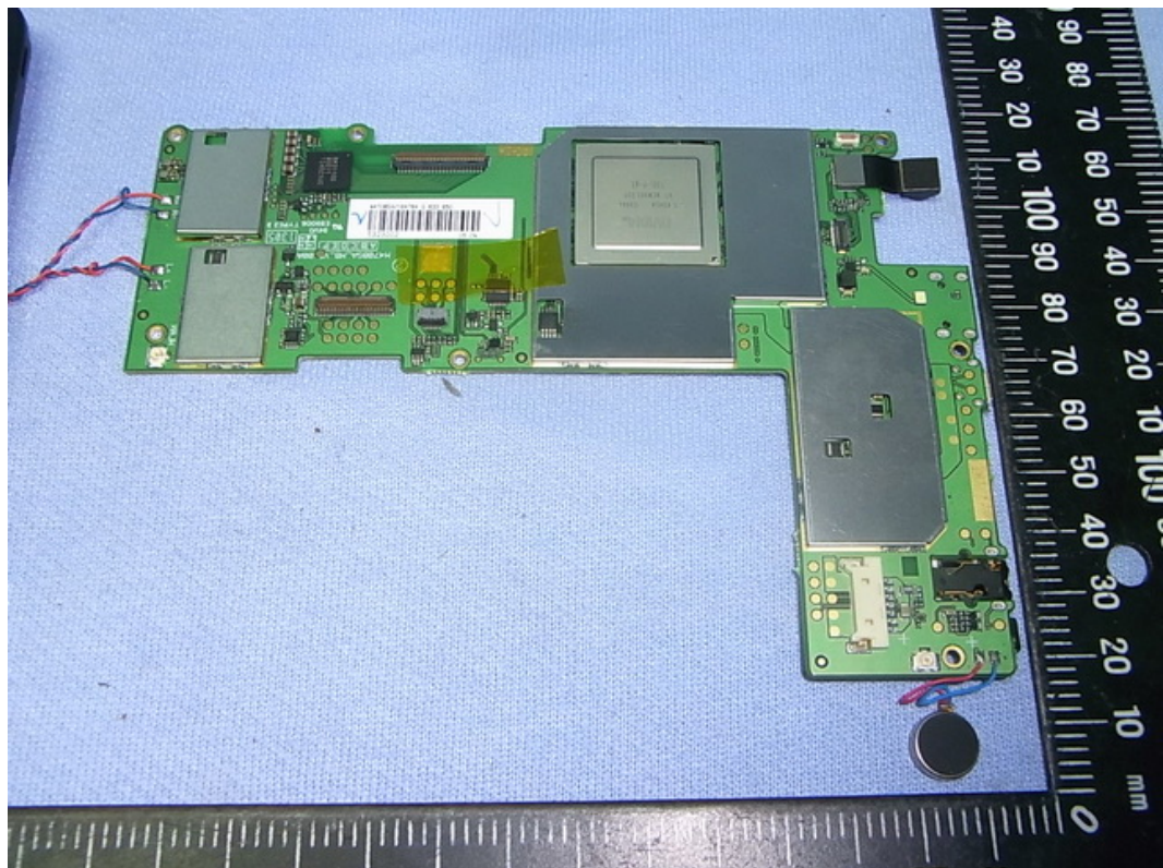
FIGURE 8 SERO 7 PRO (M/N: M470BSA) MAIN BOARD (COMPONENT SIDE)
