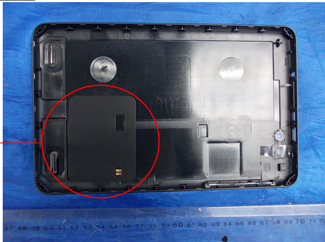
FIGURE 6 SERO 7 PRO (M/N: M470BSA) COVER REMOVED (INSIDE VIEW)
