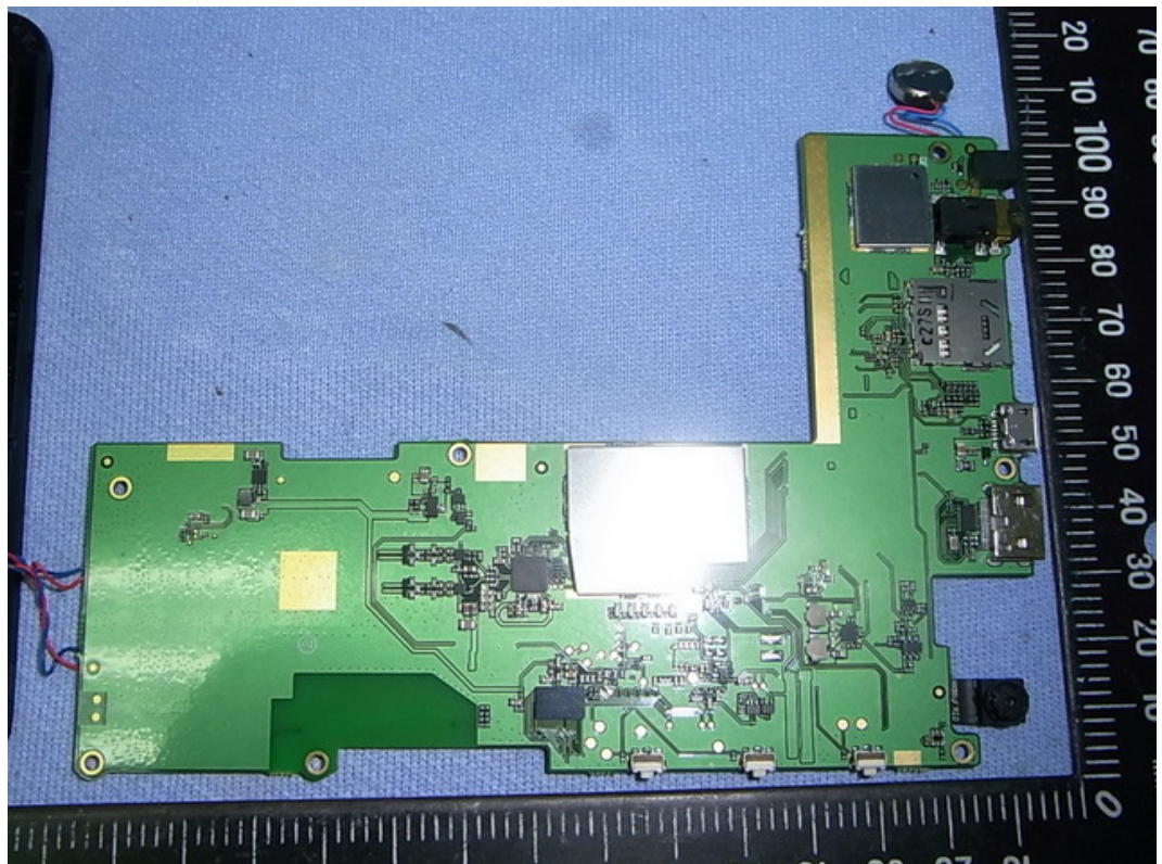
FIGURE 10 SERO 7 PRO (M/N: M470BSA) MAIN BOARD (SOLDERED SIDE)
