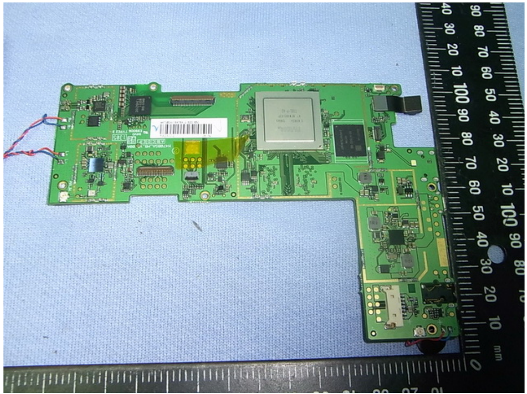
FIGURE 9 SERO 7 PRO (M/N: M470BSA) MAIN BOARD (COMPONENT SIDE – SHIELDED SHELL REMOVED)
