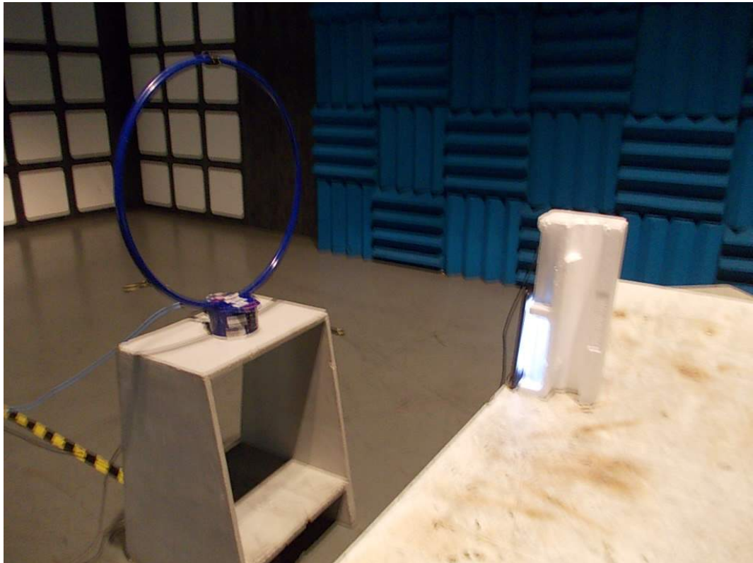
FRONT VIEW OF RADIATED EMISSION TEST ( < 30\text{MHz} )
