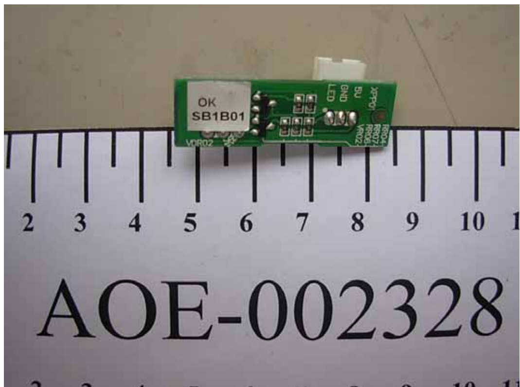
FIGURE 22 LCD MONITOR (M/N: NVU52FX5) LED BOARD 2 (SOLDERED SIDE)
