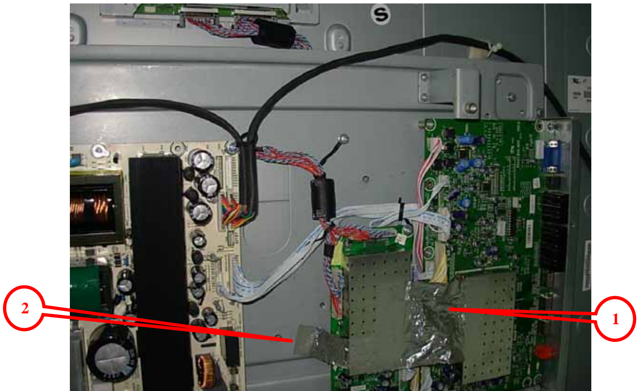
FIGURE 30 LCD MONITOR (M/N: NVU52FX5) DEBUG #2
