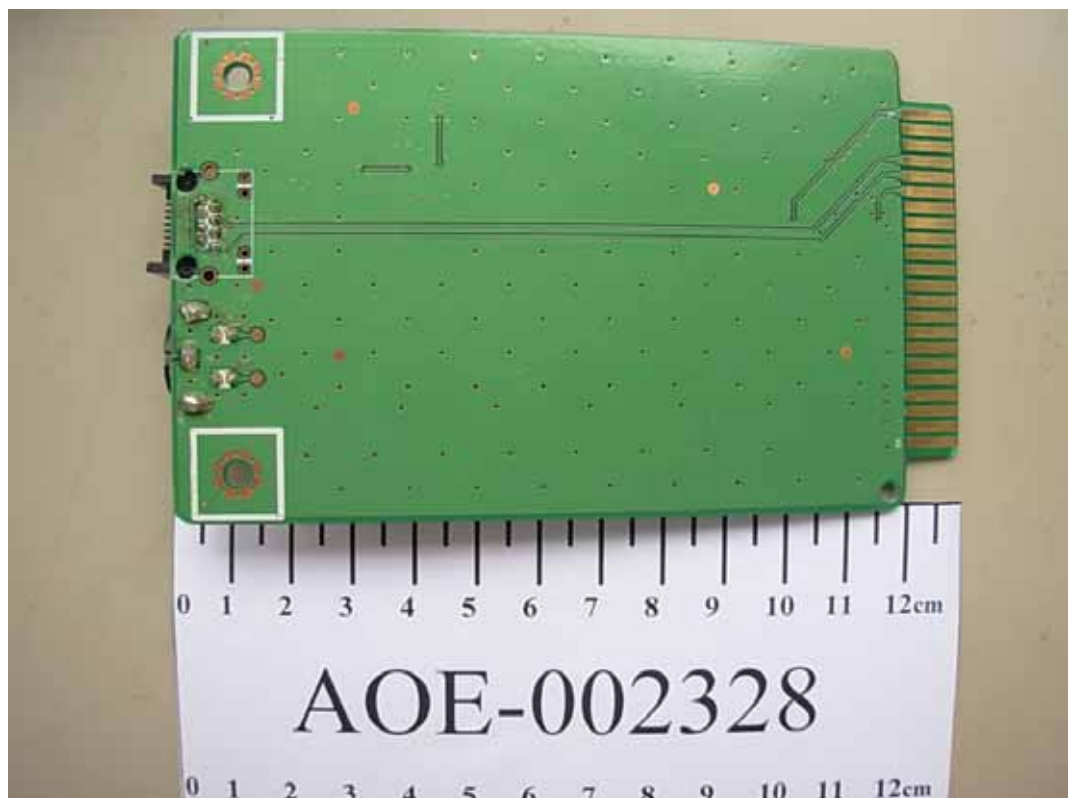
FIGURE 17 LCD MONITOR (M/N: NVU52FX5) LAN BOX (SOLDERED SIDE)
