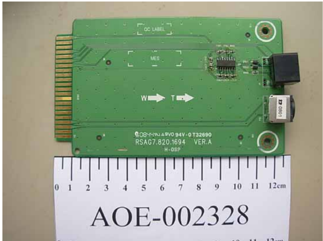
FIGURE 16 LCD MONITOR (M/N: NVU52FX5) LAN BOX (COMPONENT SIDE)
