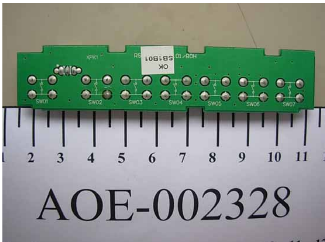
FIGURE 24 LCD MONITOR (M/N: NVU52FX5) BUTTON BOARD (SOLDERED SIDE)
