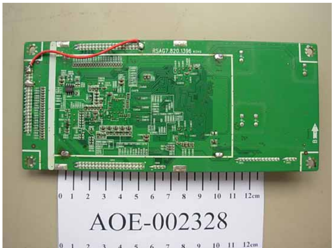
FIGURE 10 LCD MONITOR (M/N: NVU52FX5) MAIN BOARD 2 (SOLDERED SIDE)
