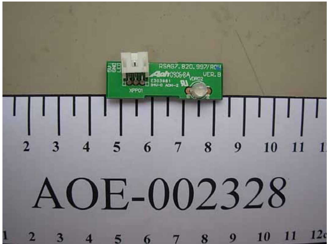
FIGURE 21 LCD MONITOR (M/N: NVU52FX5) LED BOARD 2 (COMPONENT SIDE)
