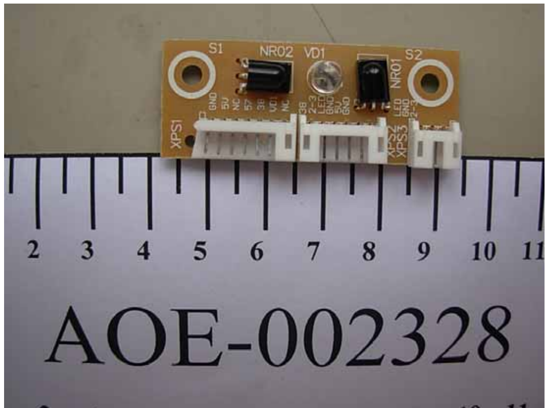
FIGURE 19 LCD MONITOR (M/N: NVU52FX5) LED BOARD 1 (COMPONENT SIDE)
