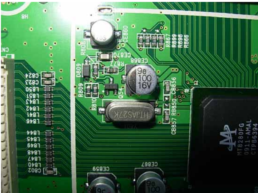
FIGURE 11 LCD MONITOR (M/N: NVU47FX5) CRYSTAL ON CONTROL BOARD
