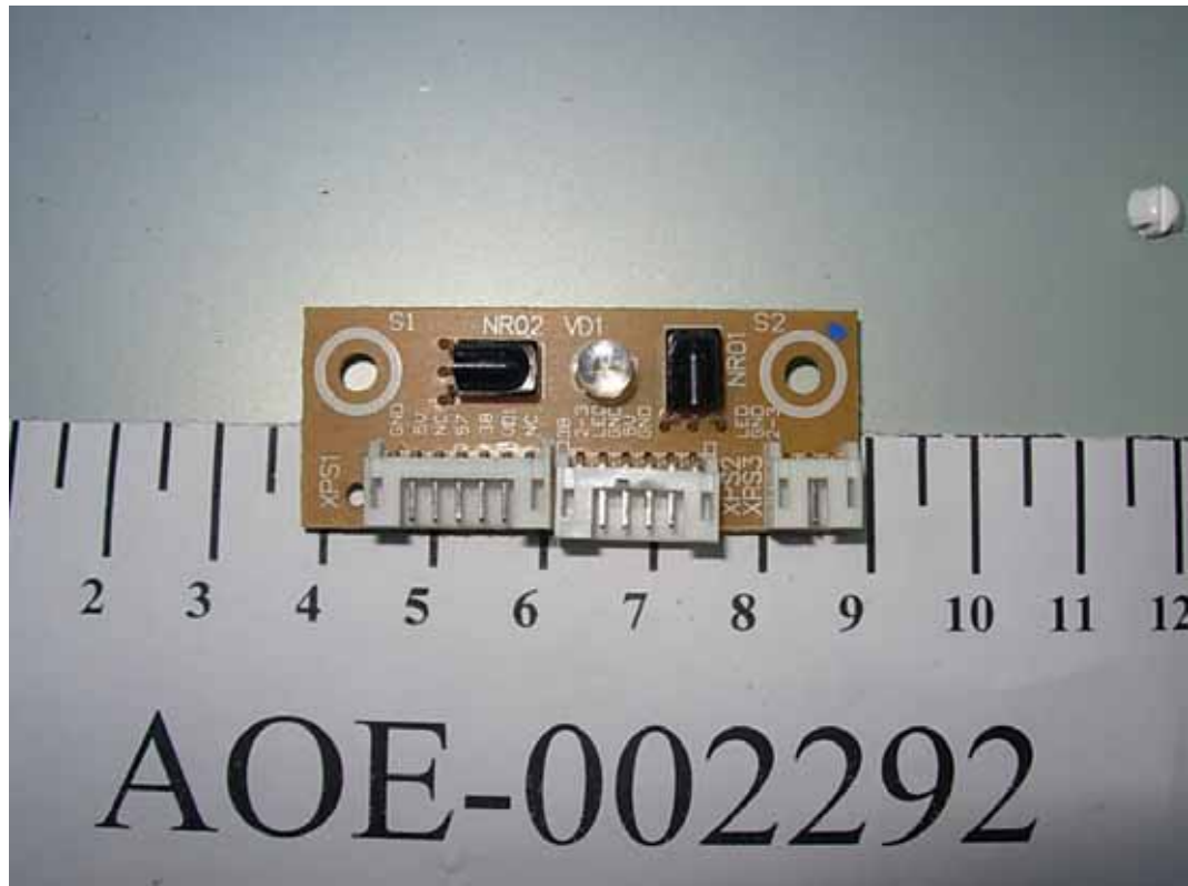
FIGURE 18 LCD MONITOR (M/N: NVU47FX5) LED PORT BOARD (COMPONENT SIDE)
