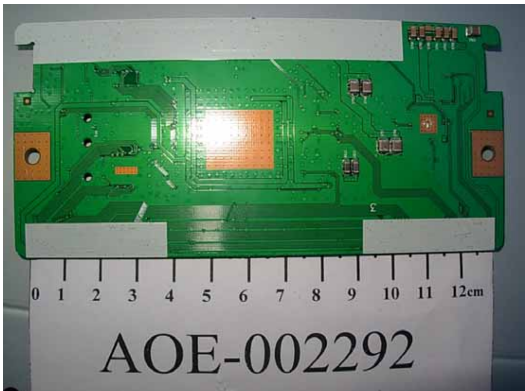
FIGURE 23 LCD MONITOR (M/N: NVU47FX5) LED BOARD (SOLDERED SIDE)
