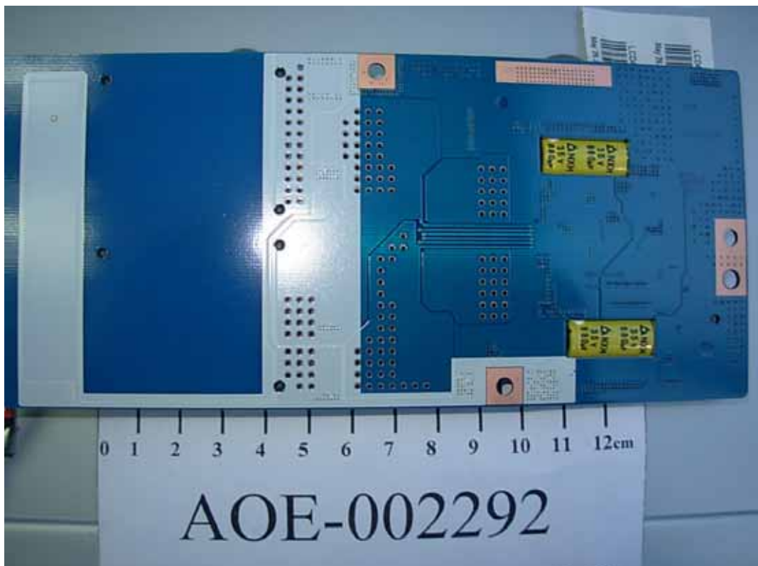
FIGURE 3 LCD MONITOR (M/N: NVU47FX5) INVERTER BOARD (SOLDERED SIDE)
