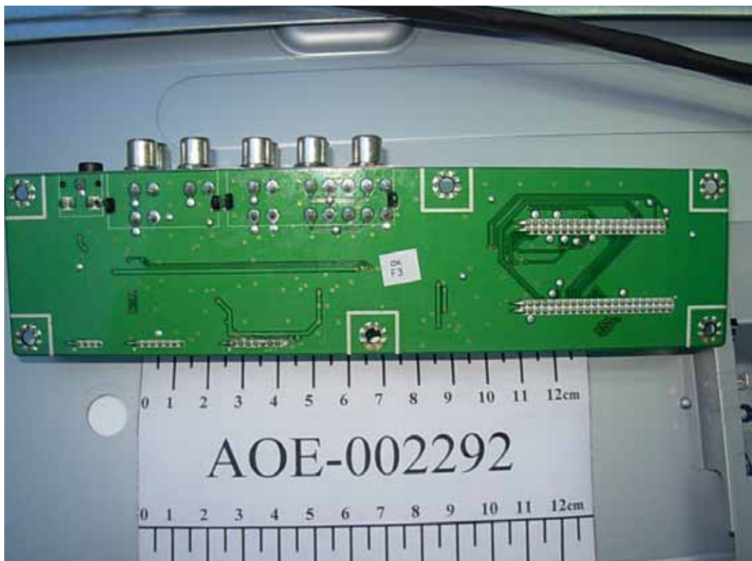
FIGURE 17 LCD MONITOR (M/N: NVU47FX5) SIGNAL BOARD (SOLDERED SIDE)
