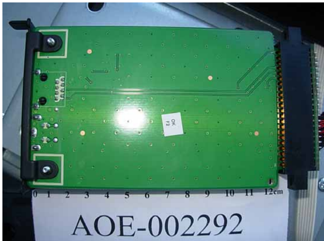
FIGURE 7 LCD MONITOR (M/N: NVU47FX5) LAN BOARD (SOLDERED SIDE)
