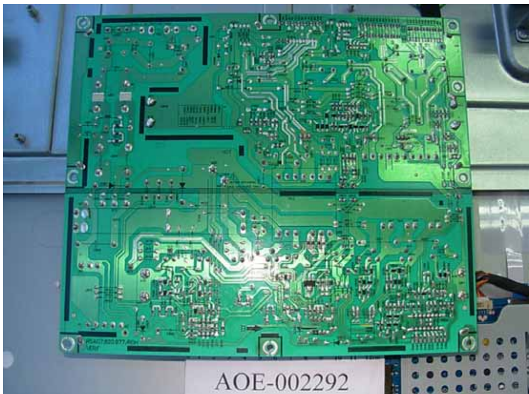
FIGURE 5 LCD MONITOR (M/N: NVU47FX5) POWER BOARD (SOLDERED SIDE)
