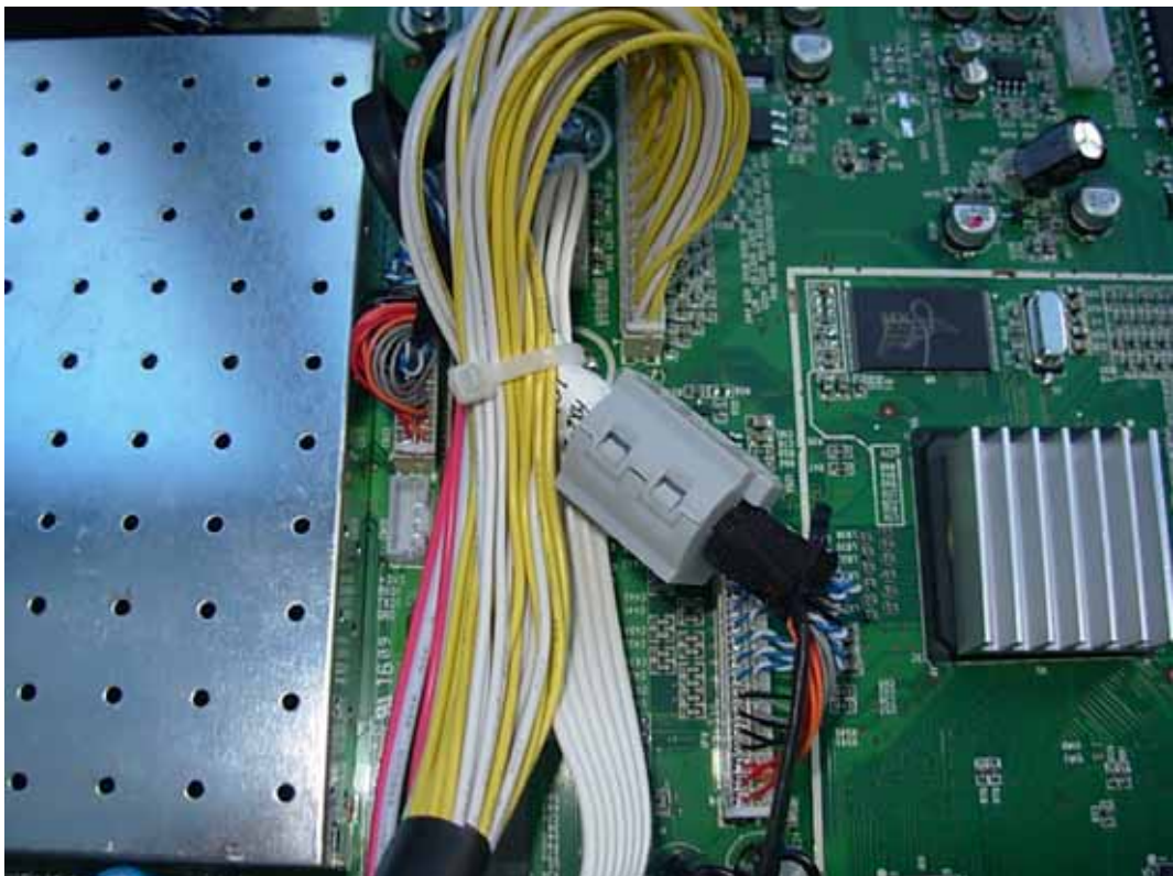
FIGURE 27 LCD MONITOR (M/N: NVU47FX5) DEBUG #2
