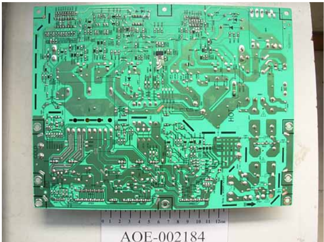
FIGURE 3 LCD MONITOR (M/N: LCD42B29GPUS) POWER BOARD (SOLDERED SIDE)
