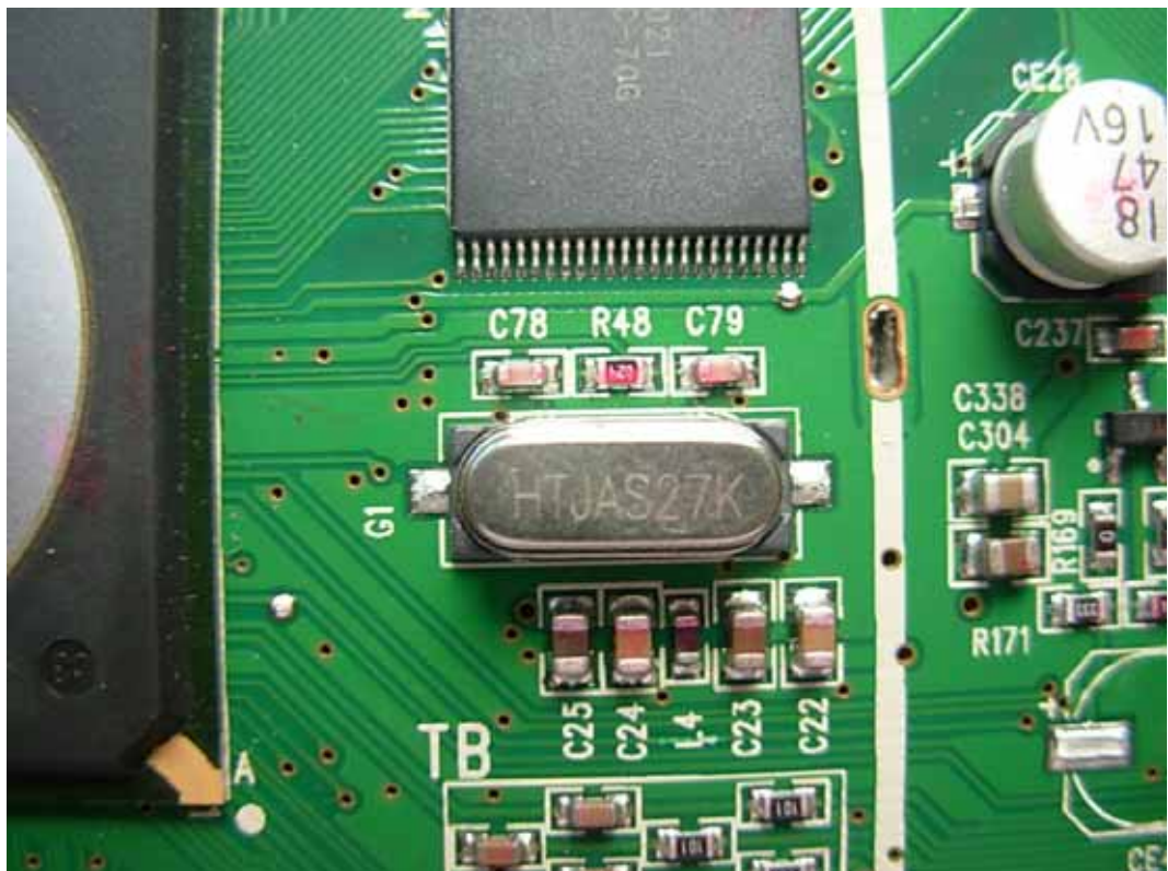
FIGURE 13 LCD MONITOR (M/N: LCD42B29GPUS) CRYSTAL #1
