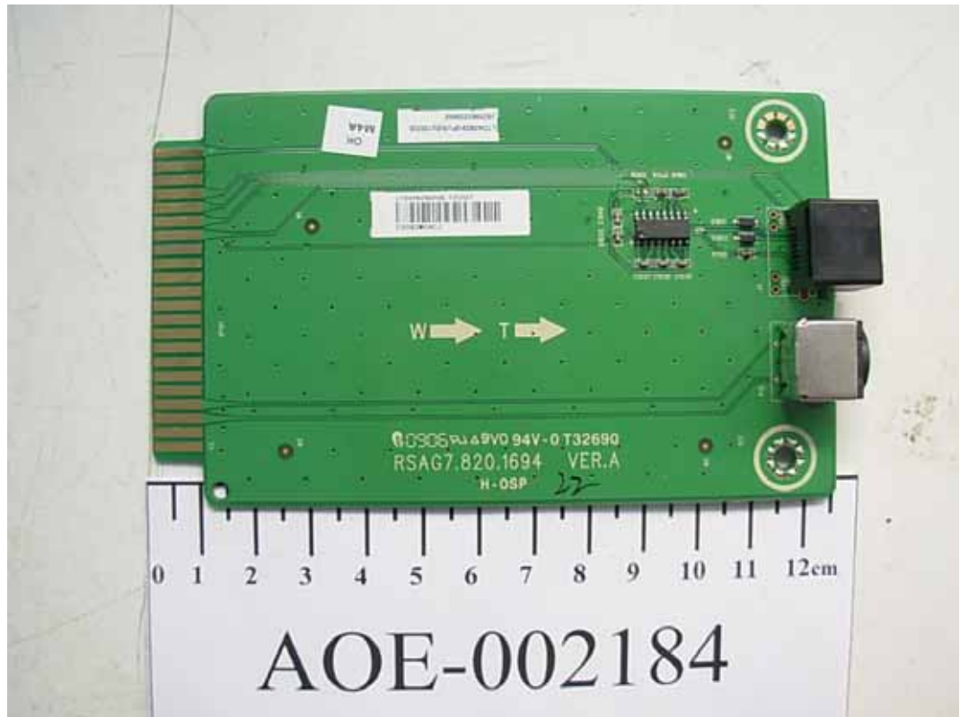
FIGURE 7 LCD MONITOR (M/N: LCD42B29GPUS) SIGNAL BOARD #2 (COMPONENT SIDE)
