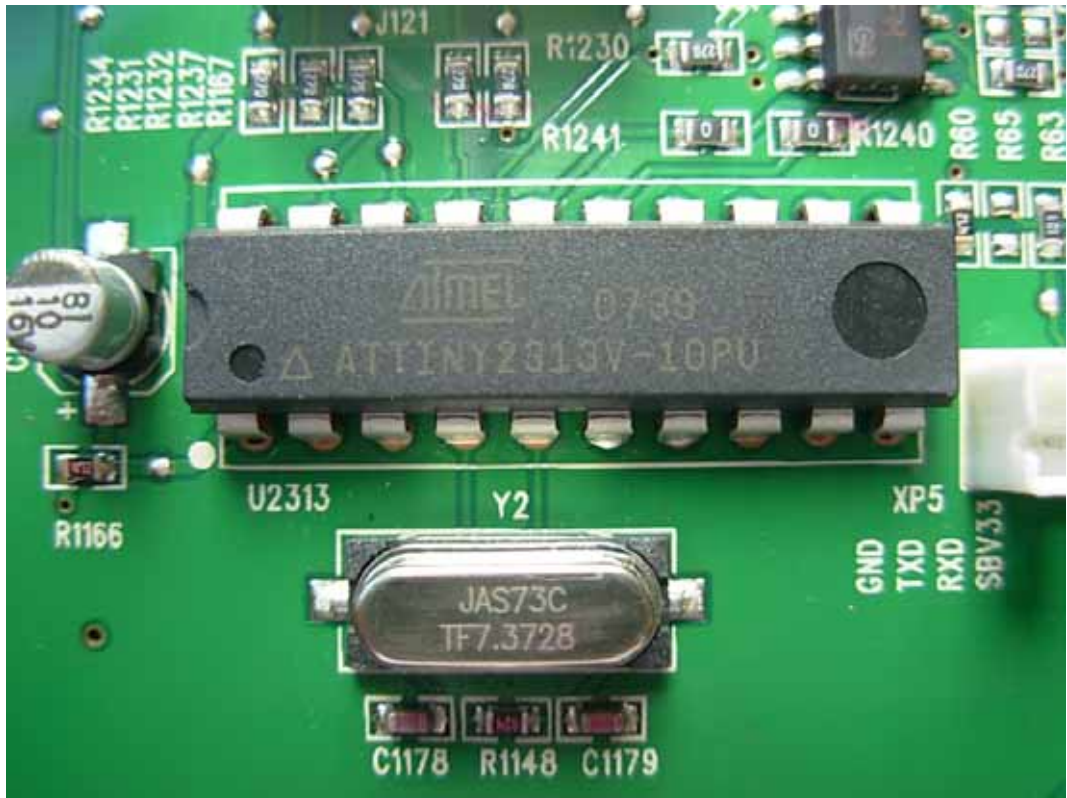
FIGURE 14 LCD MONITOR (M/N: LCD42B29GPUS) CHIP #2 & CRYSTAL #2
