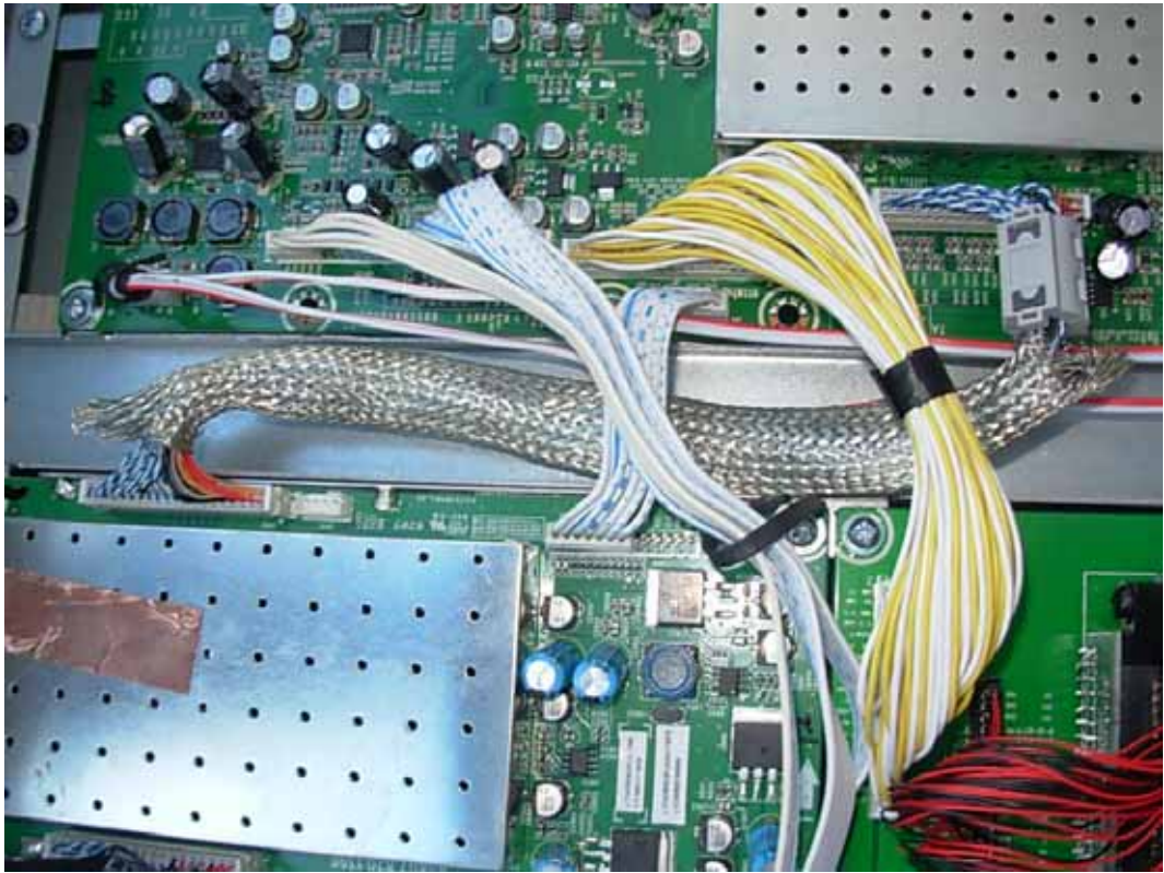
FIGURE 26 LCD MONITOR (M/N: LCD42B29GPUS) DEBUG 2
