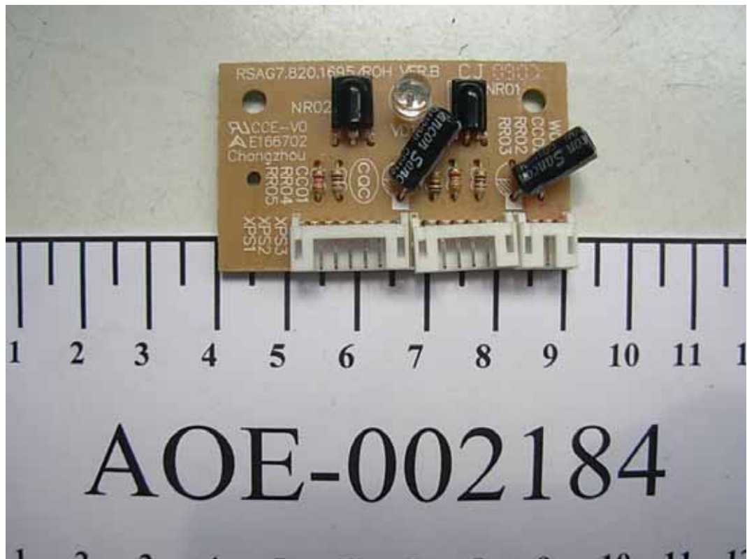
FIGURE 18 LCD MONITOR (M/N: LCD42B29GPUS) LED BOARD (COMPONENT SIDE)
