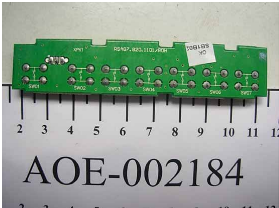
FIGURE 21 LCD MONITOR (M/N: LCD42B29GPUS) BUTTON BOARD (SOLDERED SIDE)
