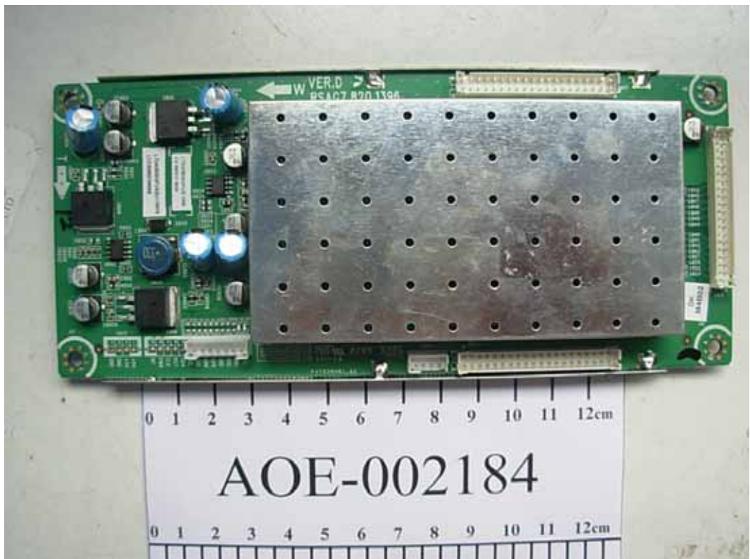
FIGURE 15 LCD MONITOR (M/N: LCD42B29GPUS) MAIN BOARD
