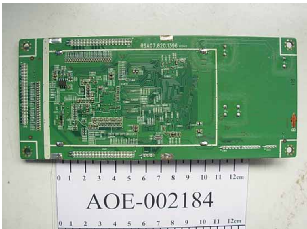
FIGURE 17 LCD MONITOR (M/N: LCD42B29GPUS) MAIN BOARD (SOLDERED SIDE)
