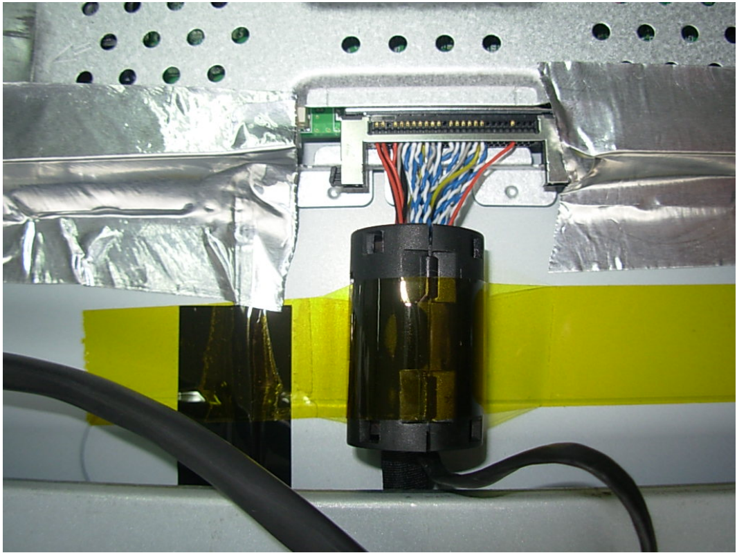
FIGURE 19 LCD TV (M/N: LTDN40W07US) DEBUG 3
