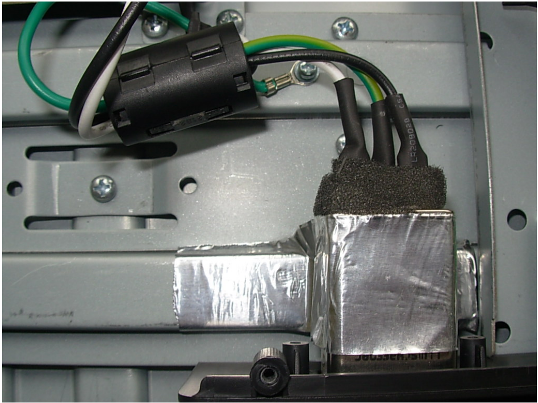
FIGURE 17 LCD TV (M/N: LTDN40W07US) DEBUG 1
