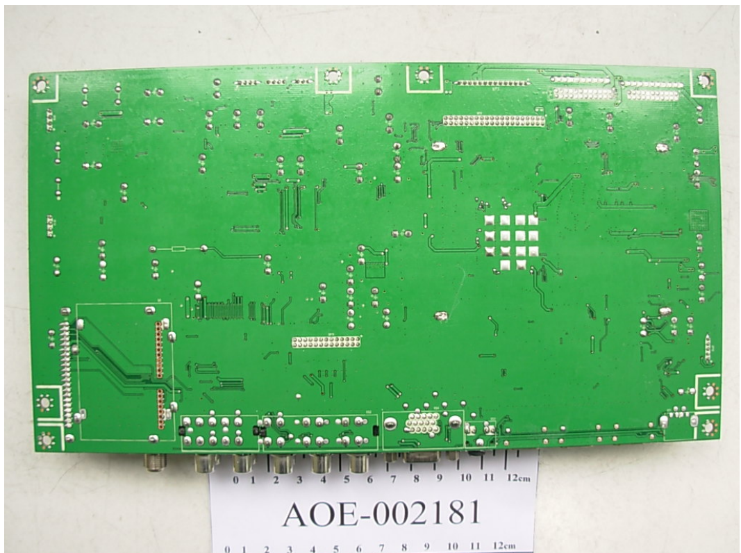
FIGURE 6 LCD TV (M/N: LTDN40W07US) MAIN BOARD (SOLDERED SIDE)
