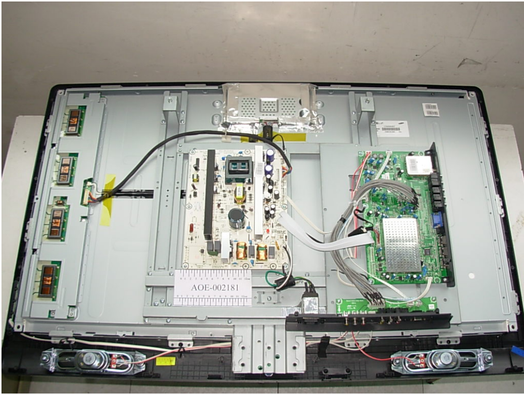
FIGURE 1 LCD TV (M/N: LTDN40W07US) COVER REMOVED
