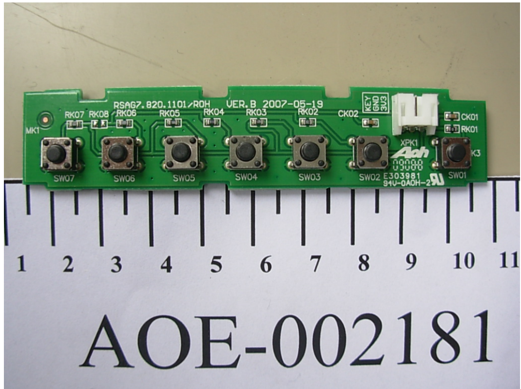
FIGURE 15 LCD TV (M/N: LTDN40W07US) BUTTON BOARD (COMPONENT SIDE)
