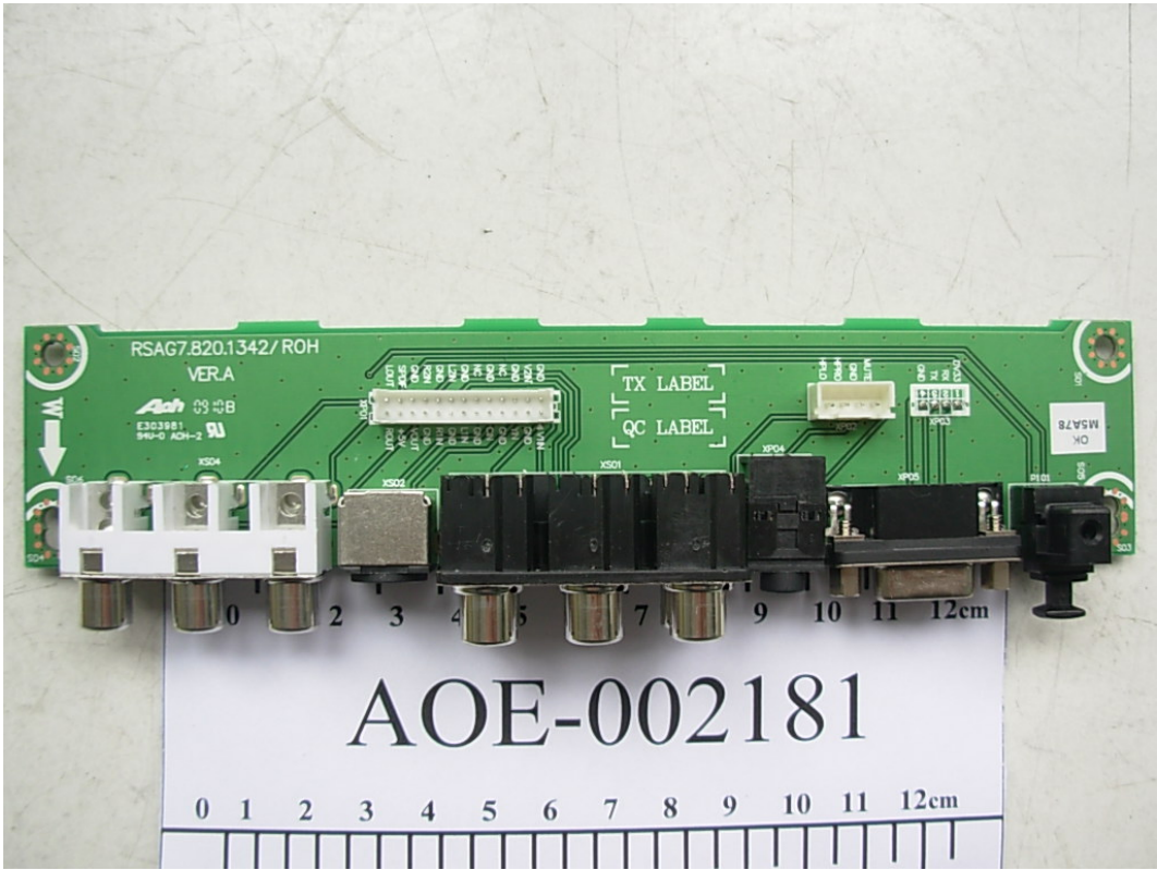
FIGURE 10 LCD TV (M/N: LTDN40W07US) SIGNAL BOARD (COMPONENT SIDE)
