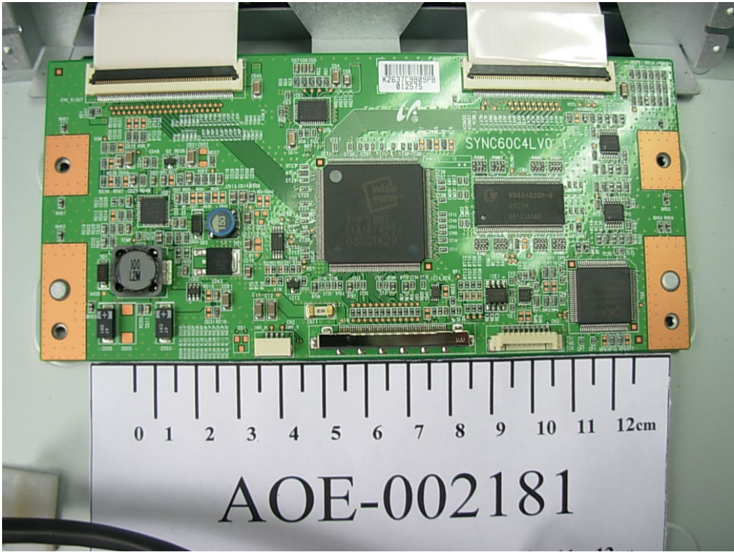
FIGURE 14 LCD TV (M/N: LTDN40W07US) LCD PANEL MAIN BOARD
