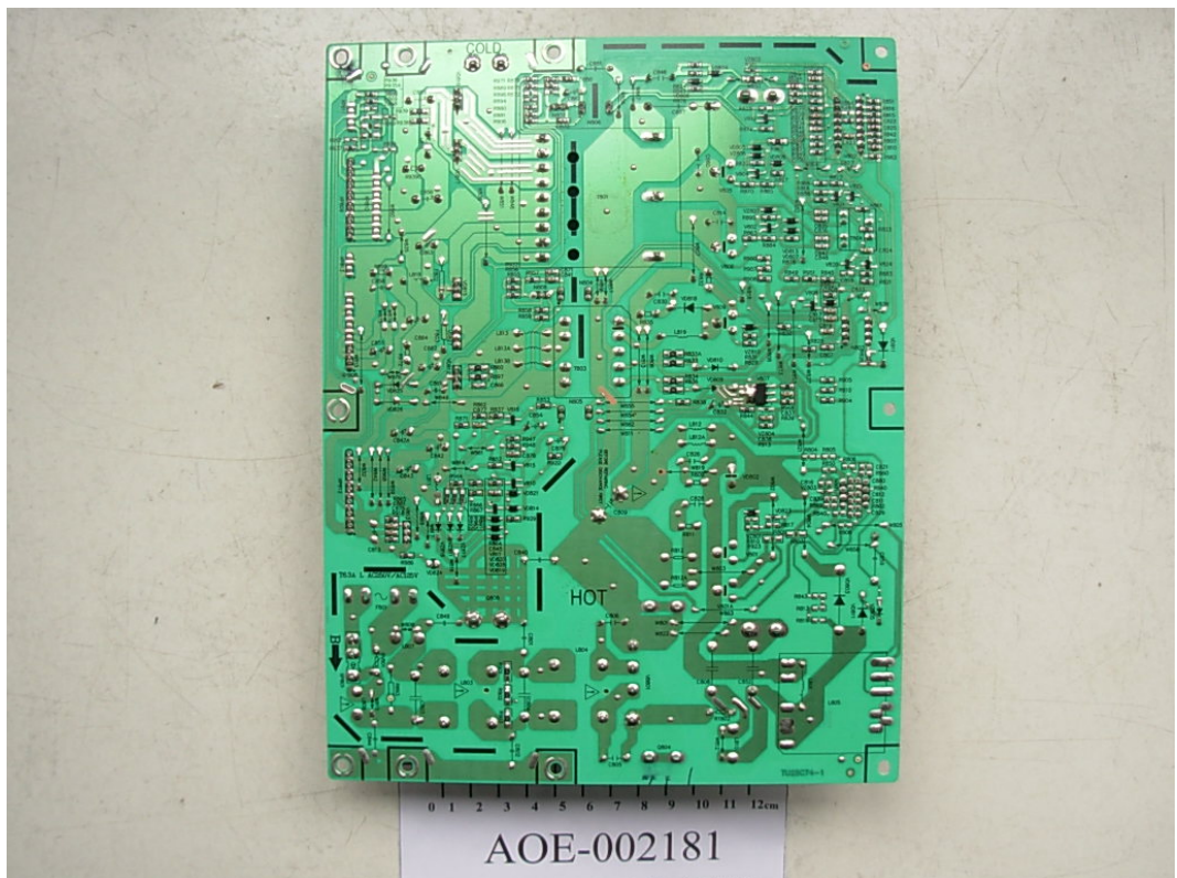
FIGURE 4 LCD TV (M/N: LTDN40W07US) POWER BOARD (SOLDERED SIDE)
