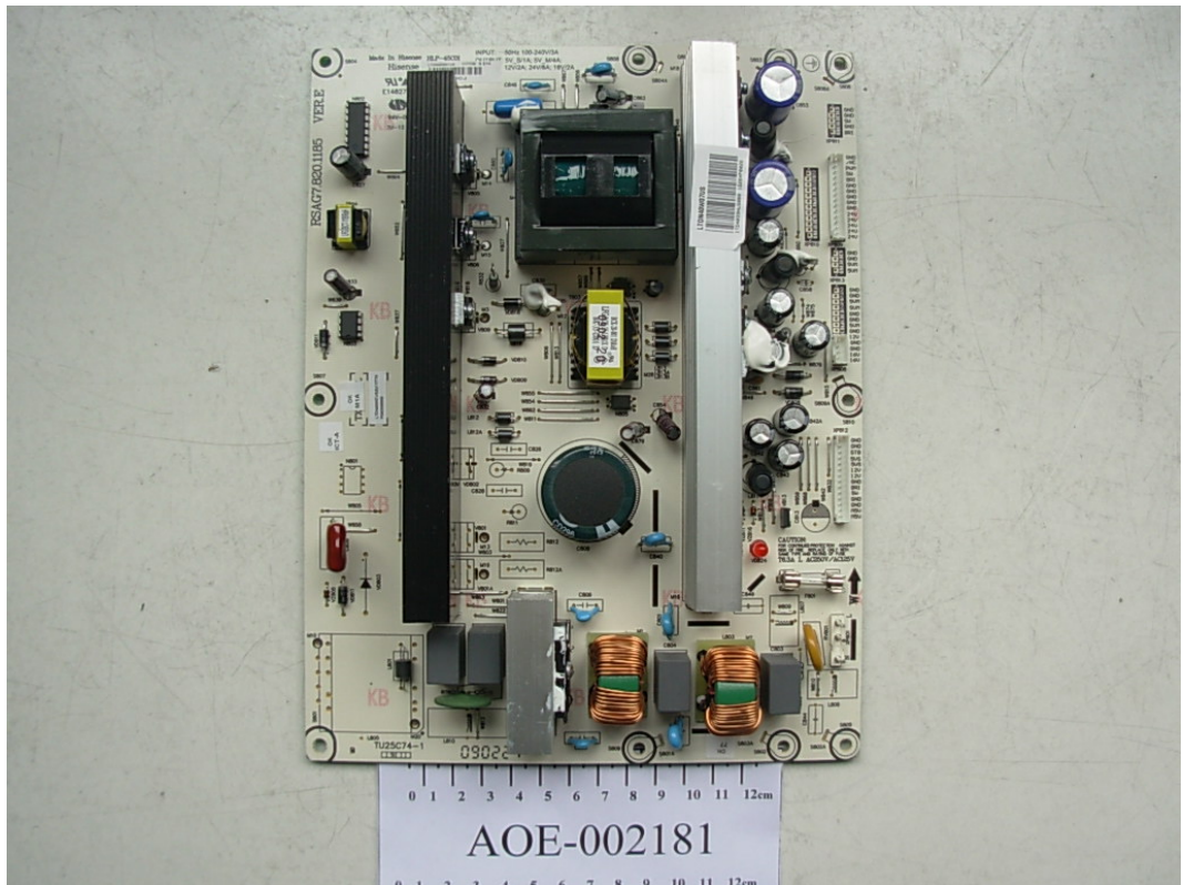
FIGURE 3 LCD TV (M/N: LTDN40W07US) POWER BOARD (COMPONENT SIDE)
