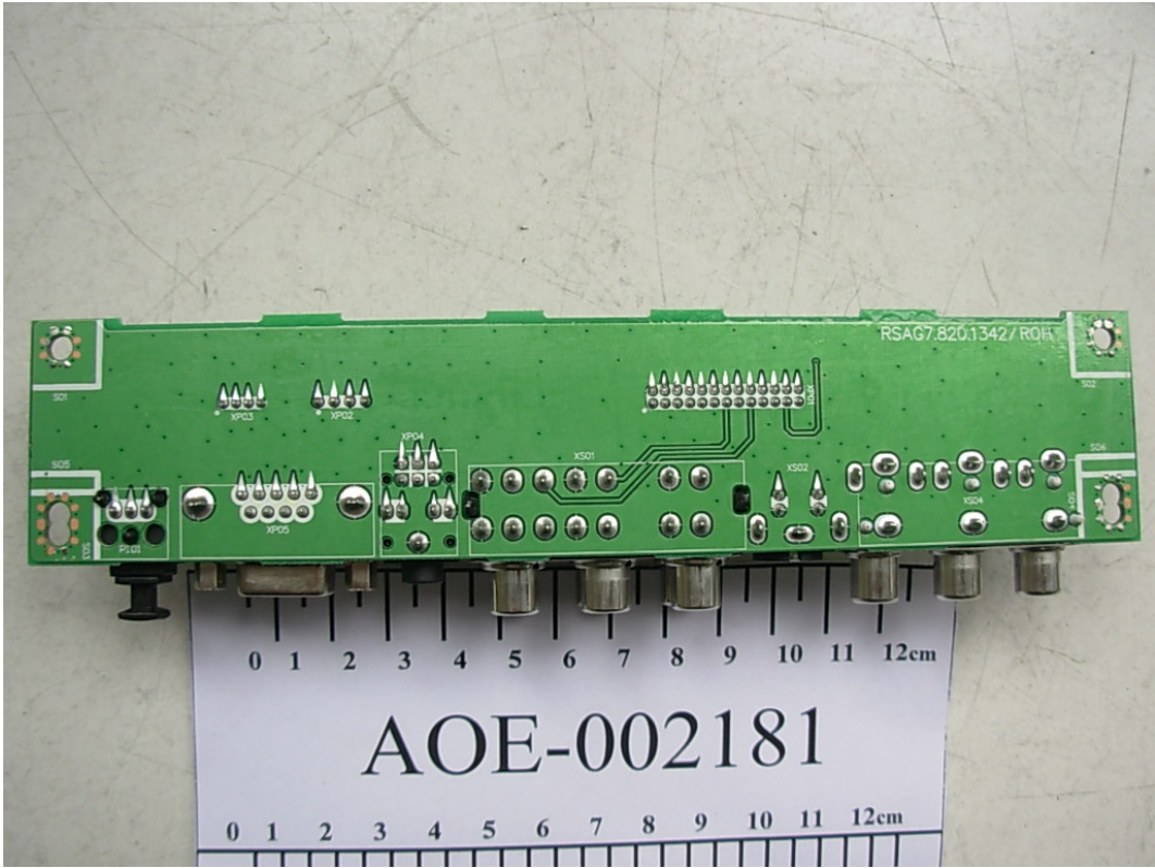
FIGURE 11 LCD TV (M/N: LTDN40W07US) SIGNAL BOARD (SOLDERED SIDE)
