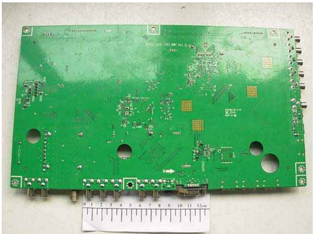
FIGURE 3 LCD TV (M/N: 55LED55SA) MAIN BOARD (SOLDERED SIDE)
