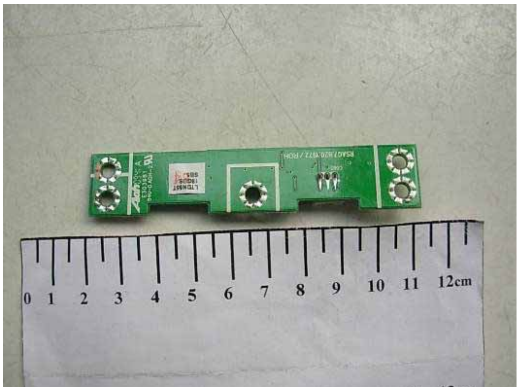
FIGURE 14 LCD TV (M/N: 55LED55SA) LED BOARD (SOLDERED SIDE)
