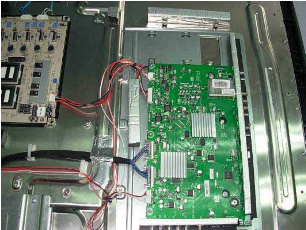
FIGURE 20 LCD TV (M/N: 55LED55SA) DEBUG #1
