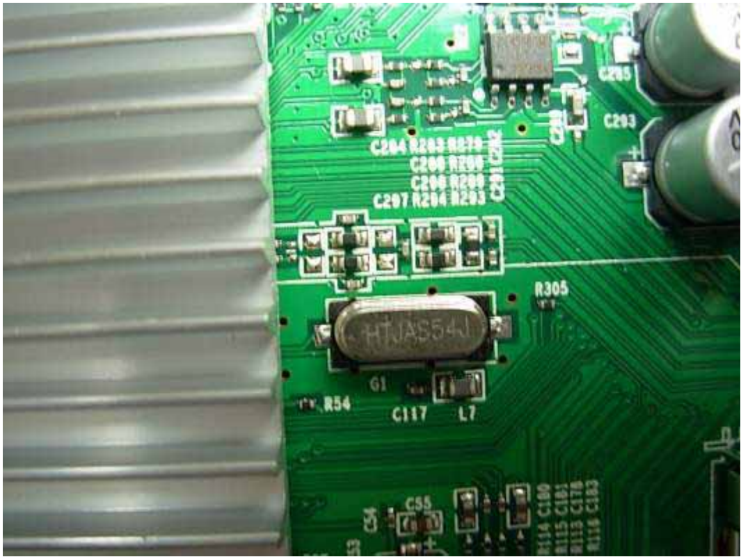
FIGURE 4 LCD TV (M/N: 55LED55SA) CRYSTAL #1 ON MAIN BOARD
