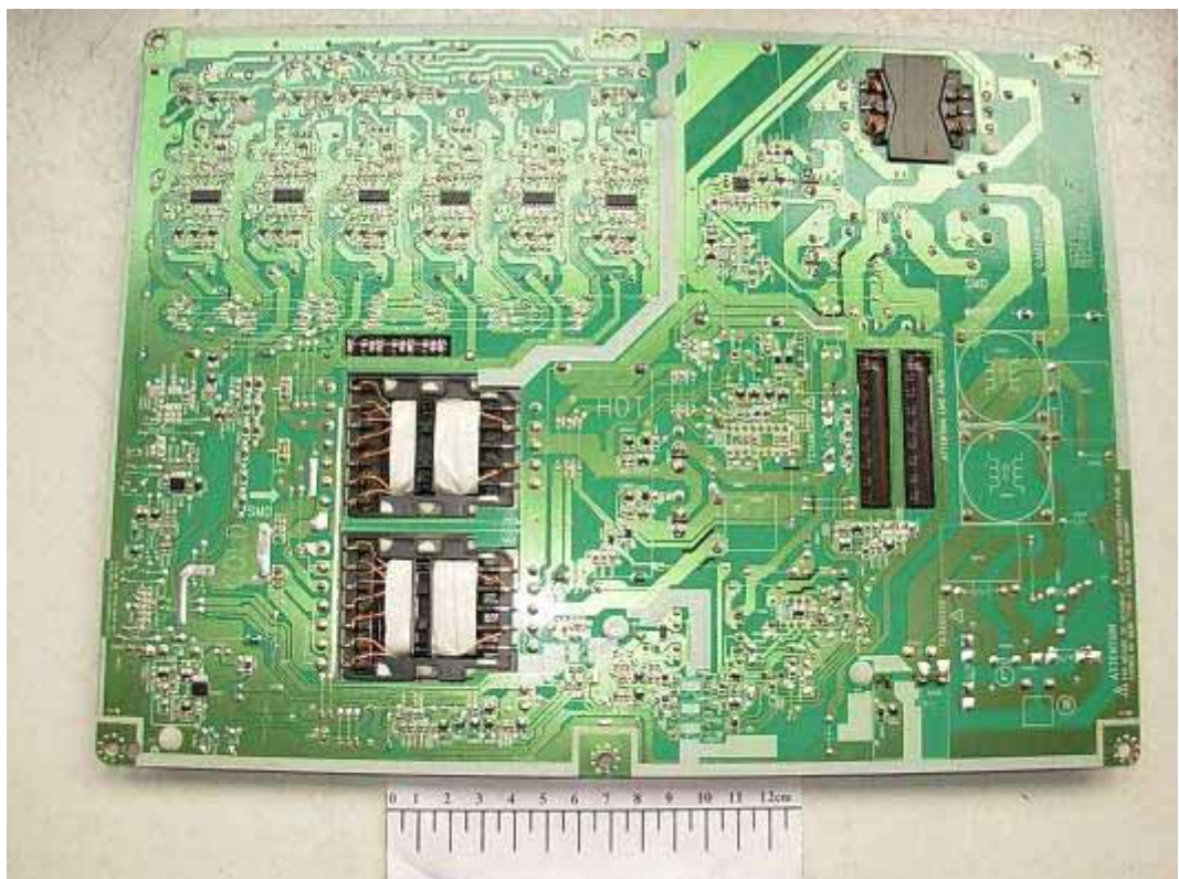
FIGURE 10 LCD TV (M/N: 55LED55SA) POWER BOARD (SOLDERED SIDE)
