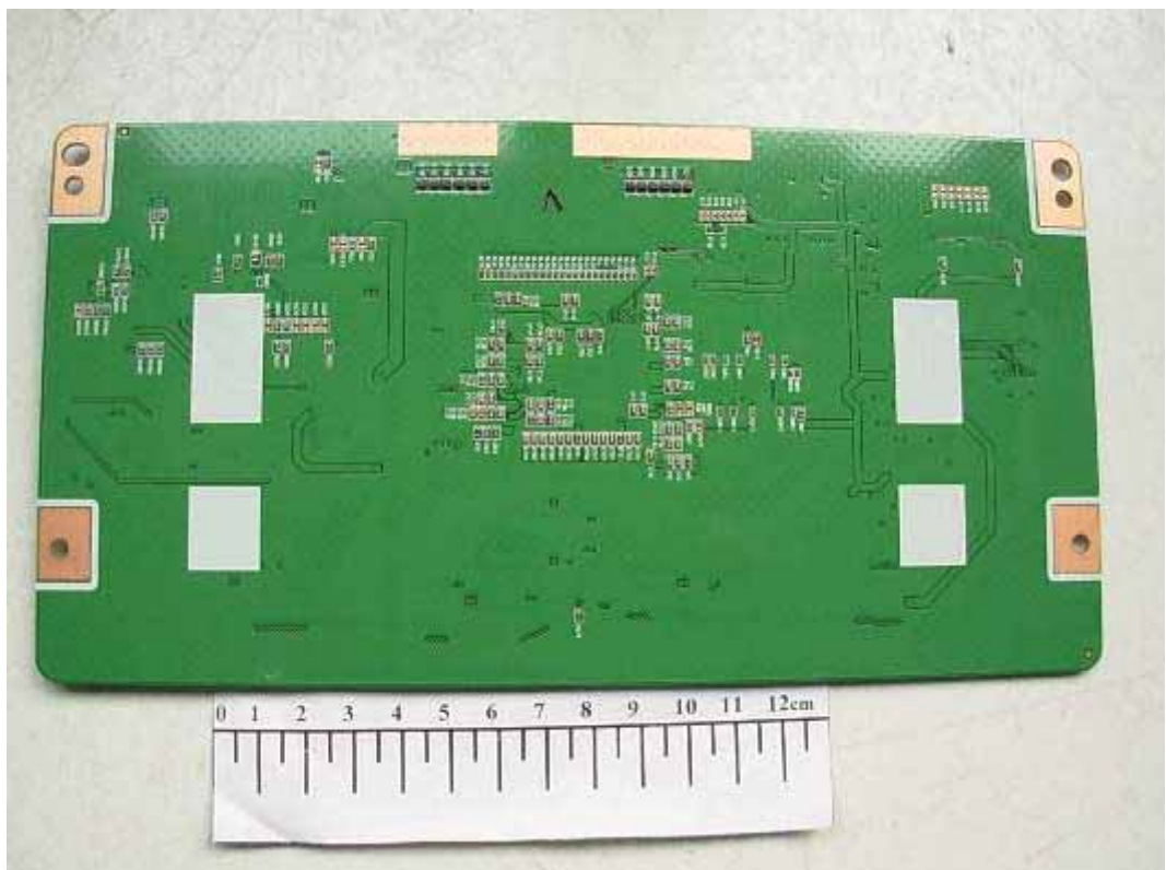
FIGURE 19 LCD TV (M/N: 55LED55SA) LCD PANEL MAIN BOARD (SOLDERED SIDE)
