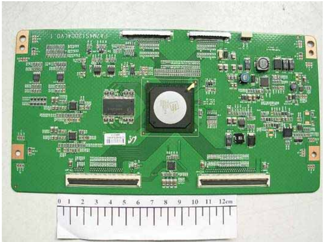
FIGURE 18 LCD TV (M/N: 55LED55SA) LCD PANEL MAIN BOARD (COMPONENT SIDE)
