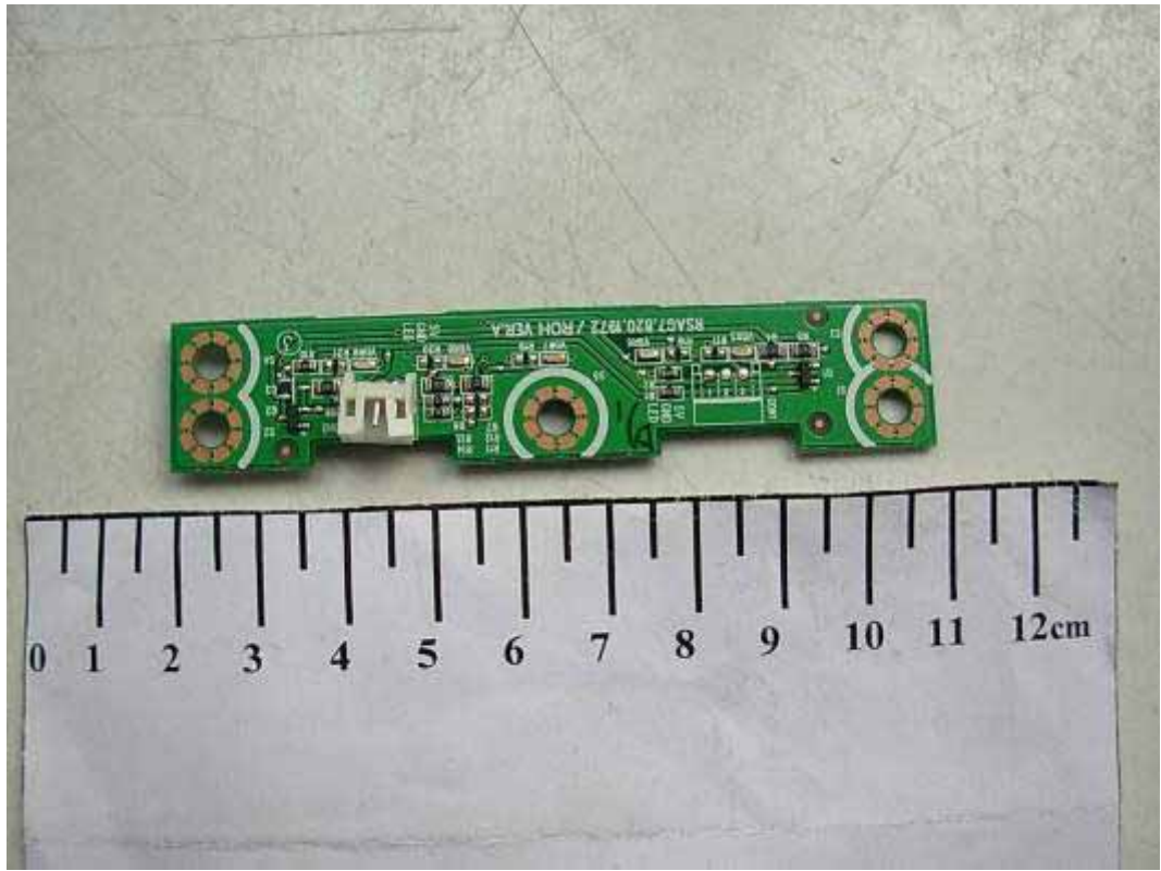
FIGURE 13 LCD TV (M/N: 55LED55SA) LED BOARD (COMPONENT SIDE)
