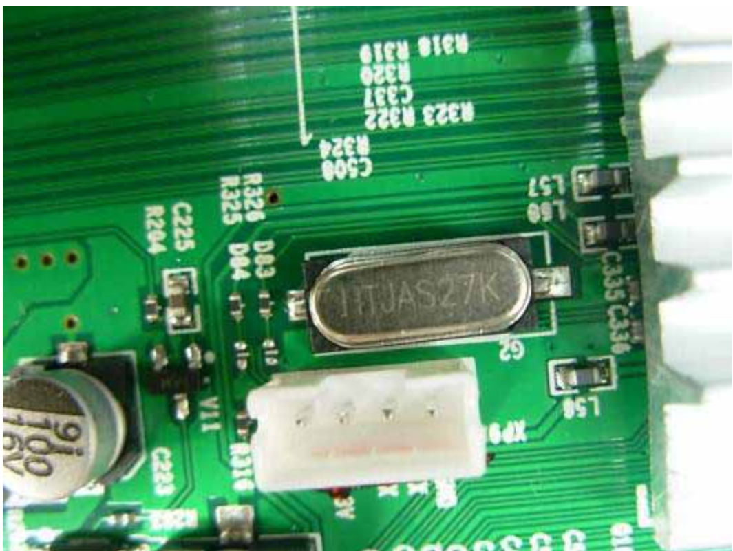
FIGURE 5 LCD TV (M/N: 55LED55SA) CRYSTAL #2 ON MAIN BOARD
