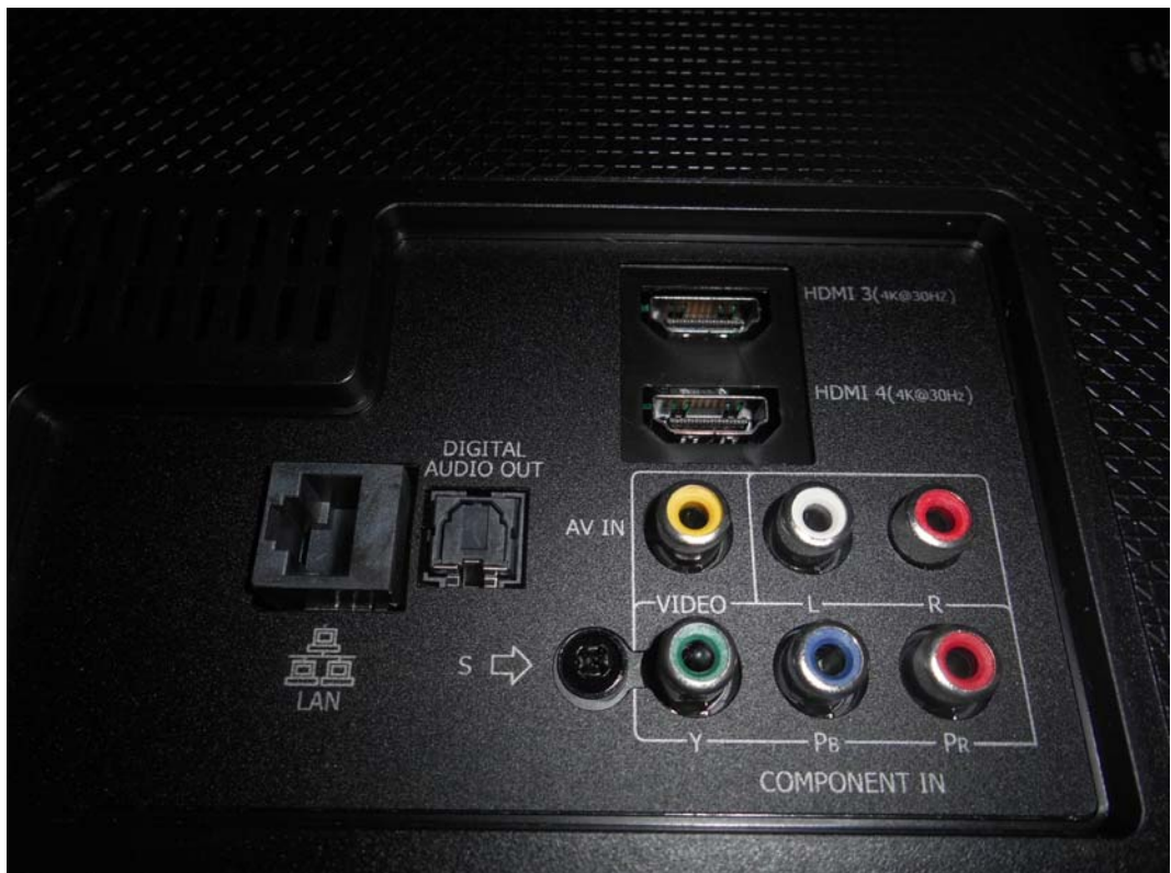
FIGURE 4 LED LCD TV (M/N: LC-50N8002U) PORTS #2
