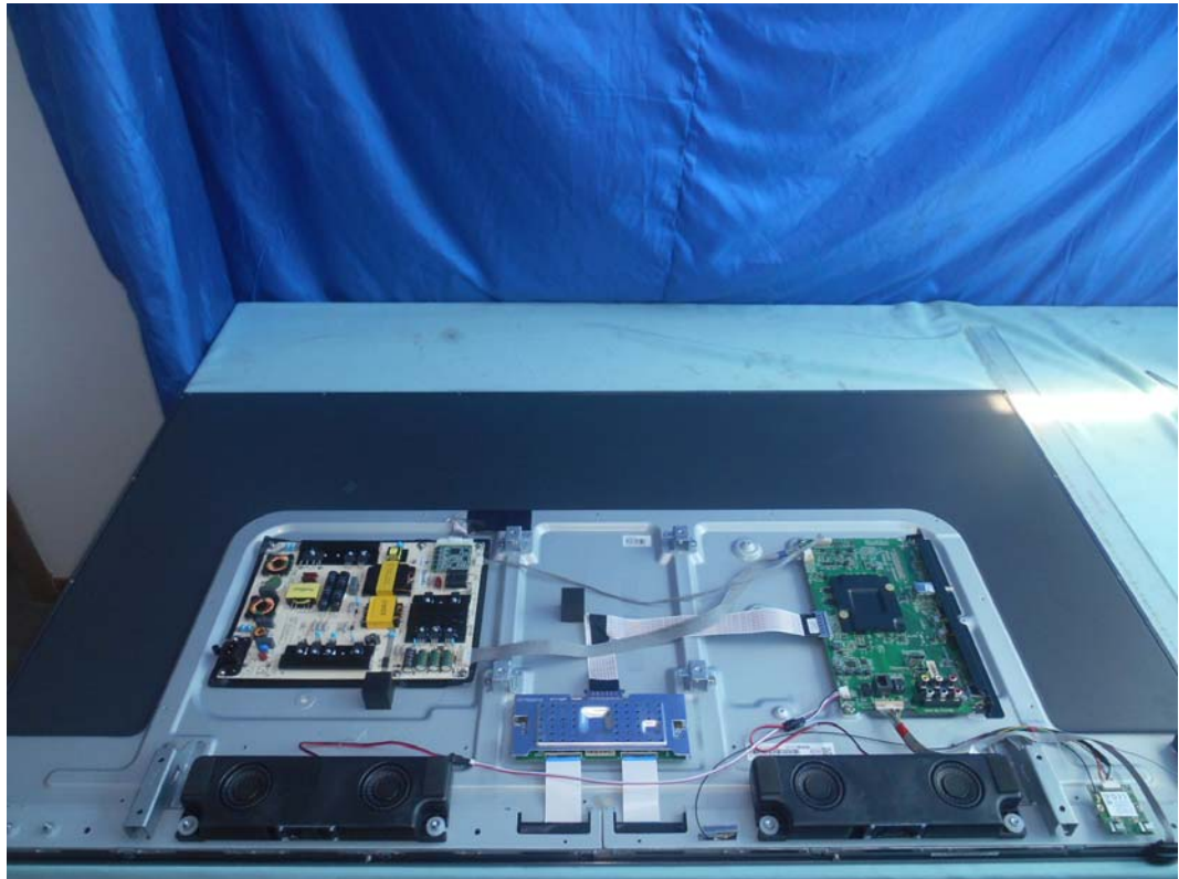
FIGURE 1 LED LCD TV (M/N: 55H9707) COVER REMOVED
