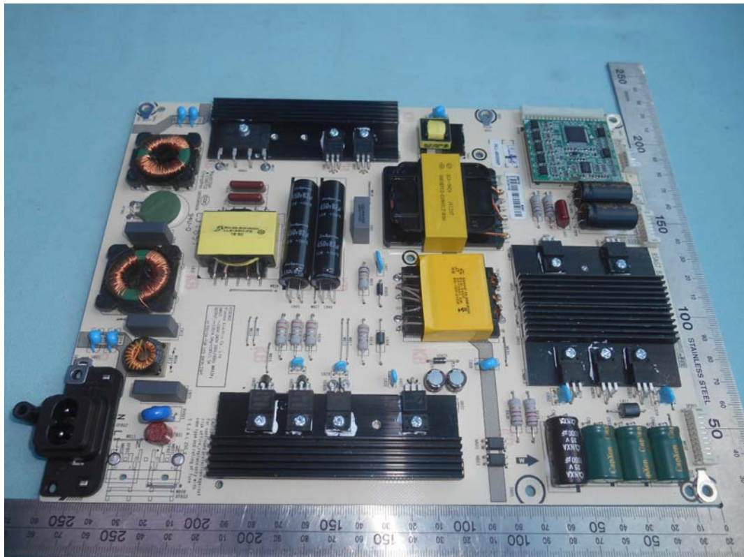
FIGURE 3 LED LCD TV (M/N: 55H9707) POWER BOARD (COMPONENT SIDE)
