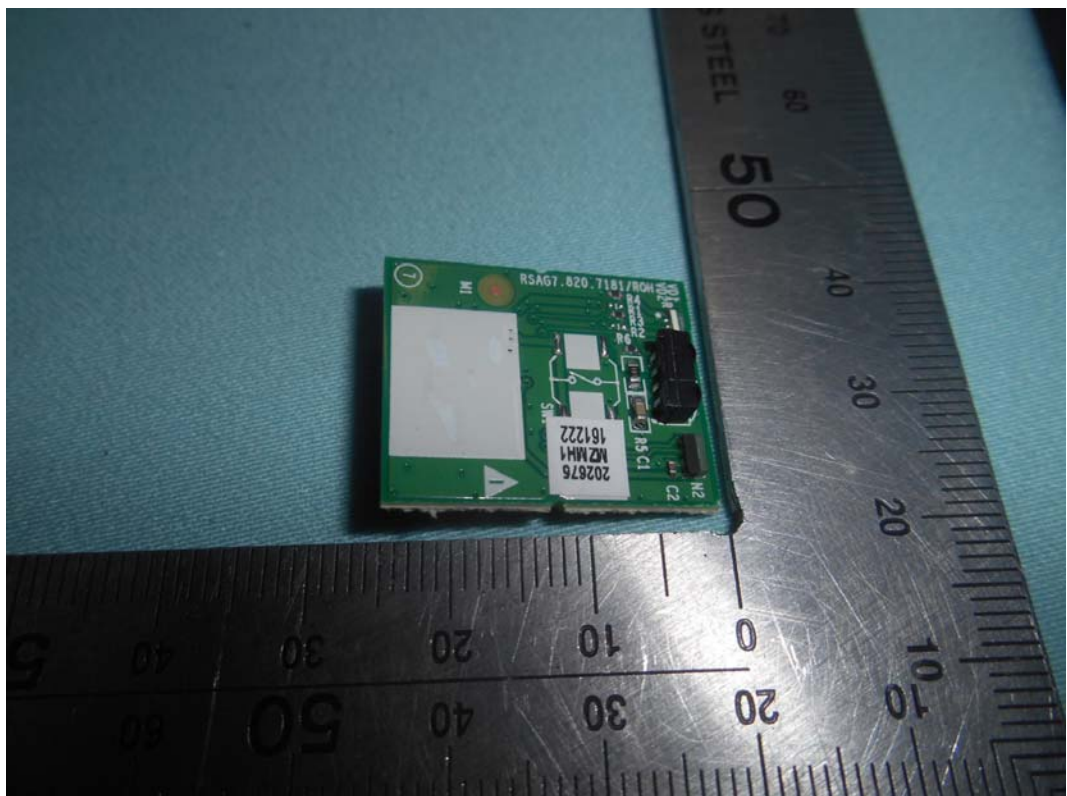
FIGURE 6 LED LCD TV (M/N: 55H9707) IR BOARD (SOLDERED SIDE)
