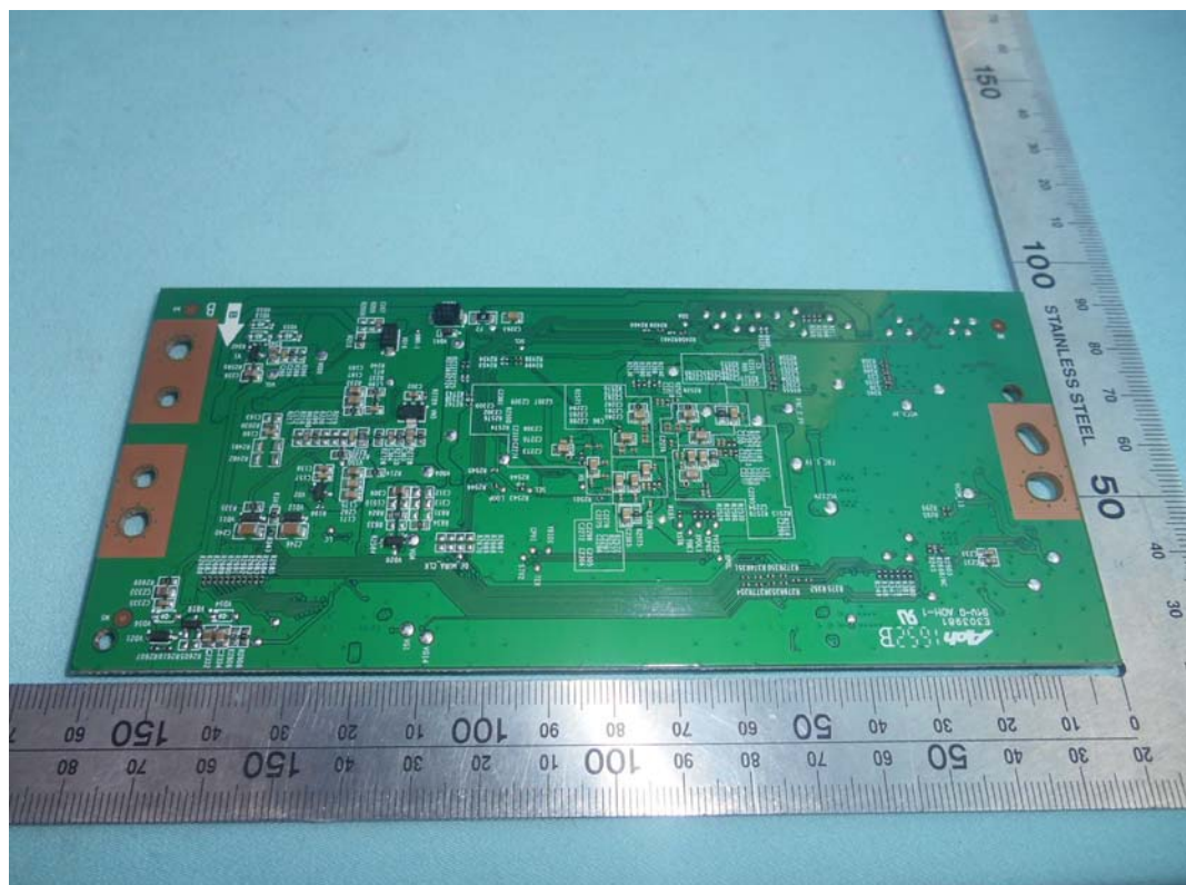
FIGURE 18 LED LCD TV (M/N: 55H9707) PANEL BOARD (SOLDERED SIDE)
