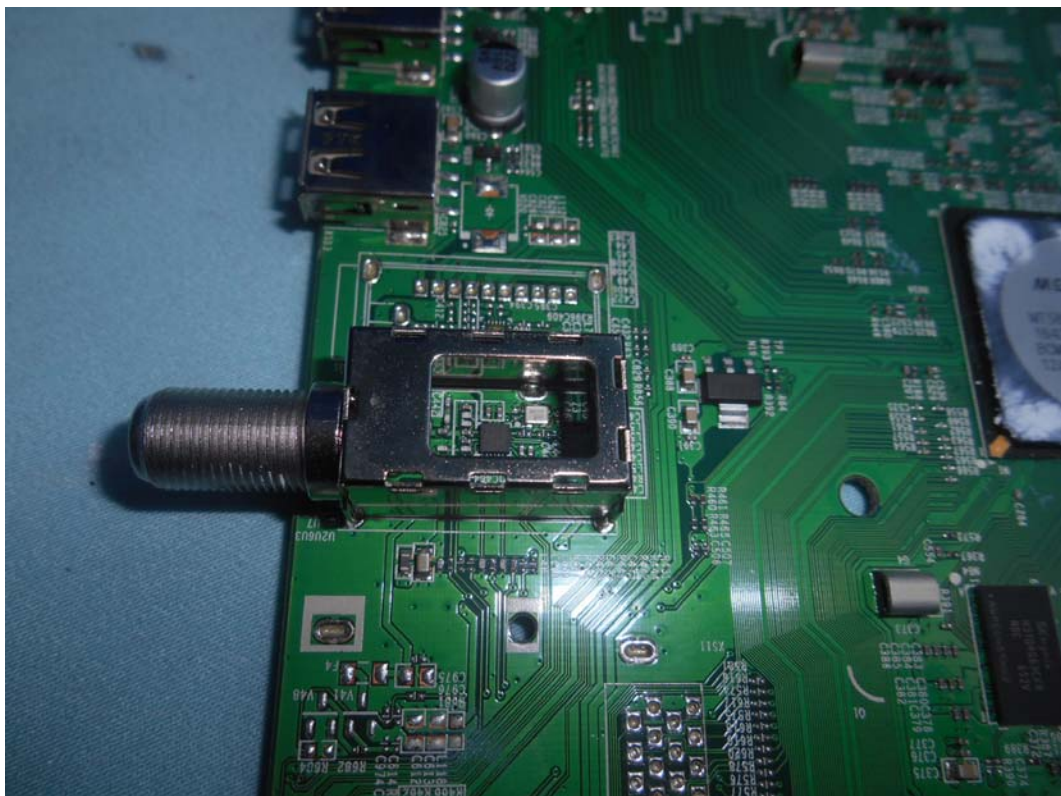
FIGURE 10 LED LCD TV (M/N: 55H9707) TUNER
