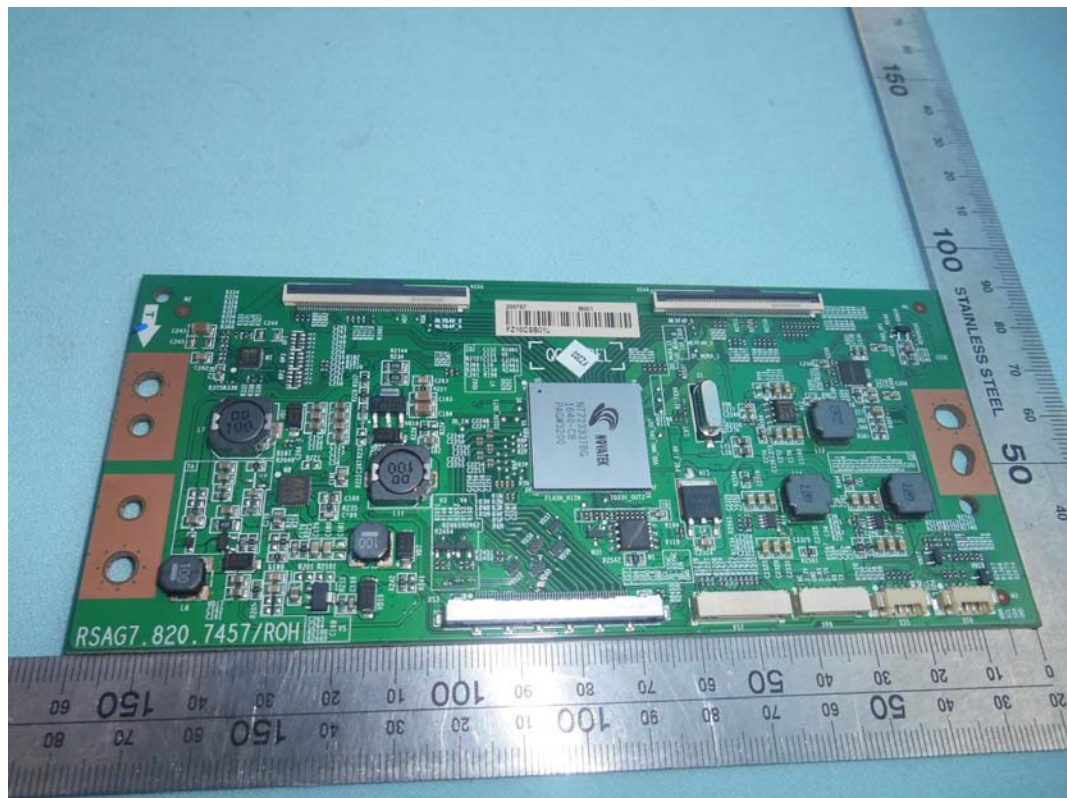
FIGURE 17 LED LCD TV (M/N: 55H9707) PANEL BOARD (COMPONENT SIDE)
