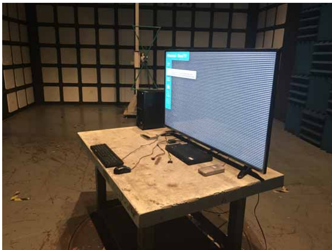
SETUP WITH MAXIMUM DETECTED EMISSION AT VERTICAL POLARIZATION (TEST MODE: HDMI1 1920*1080@60Hz & 1kHz)
