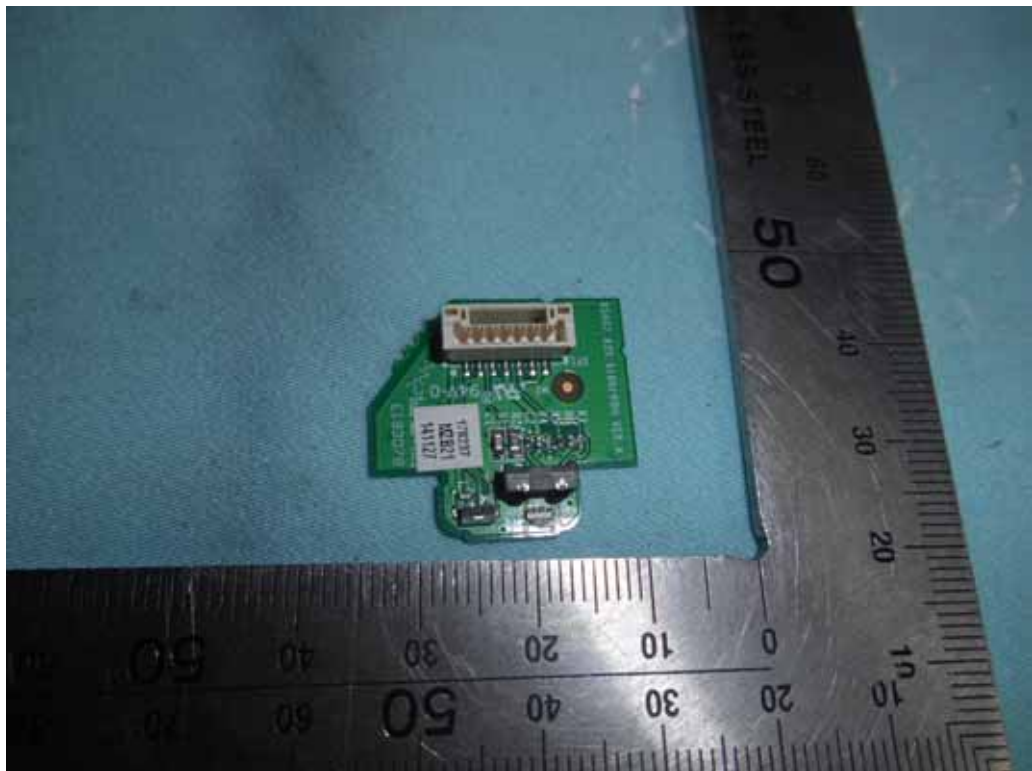
FIGURE 18 LED LCD TV (M/N: 55K2203W) IR BOARD (COMPONENT SIDE)
