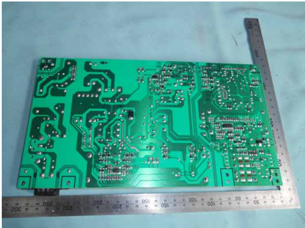
FIGURE 15 LED LCD TV (M/N: 55K2203W) POWER BOARD (SOLDERED SIDE)
