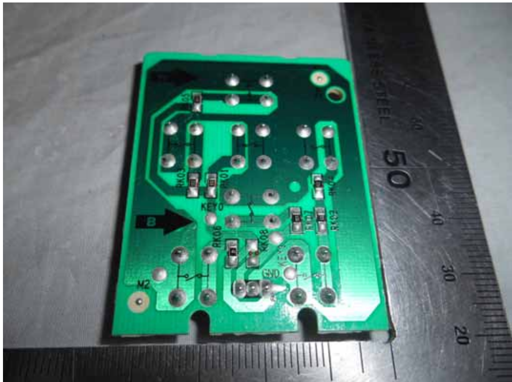
FIGURE 17 LED LCD TV (M/N: 55K2203W) KEY BOARD (SOLDERED SIDE)
