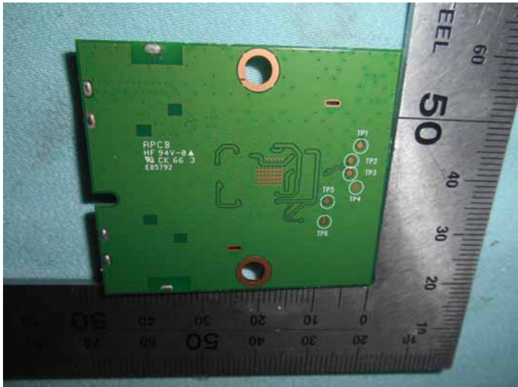
FIGURE 11 LED LCD TV (M/N: 55K2203W) RF BOARD (SOLDERED SIDE)
