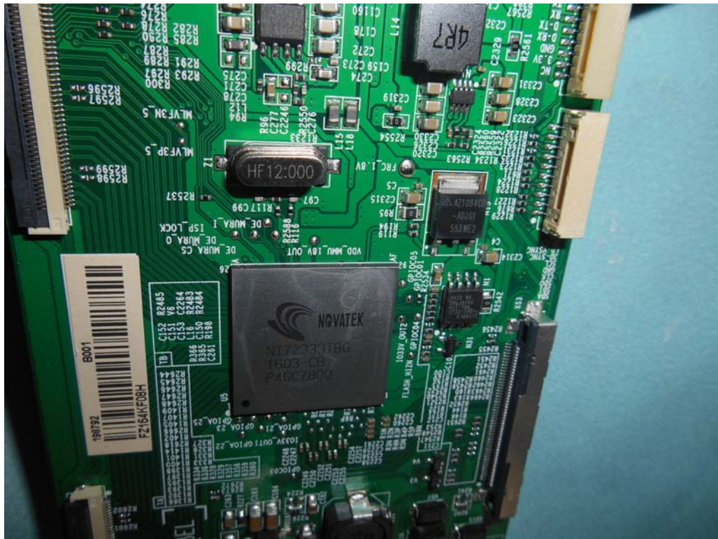
FIGURE 21 LED LCD TV (M/N: LC-55N7000U) CONTROL BOARD (COMPONENT SIDE)
