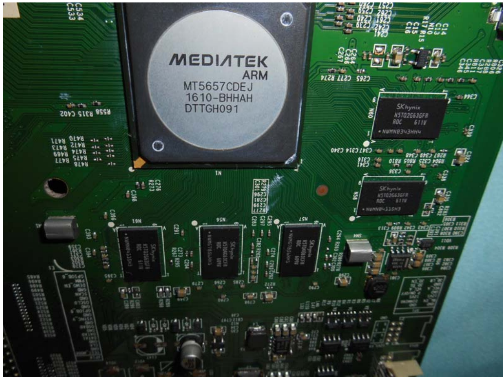
FIGURE 5 LED LCD TV (M/N: LC-55N7000U) CHIP & CRYSTAL ON MAIN BOARD
