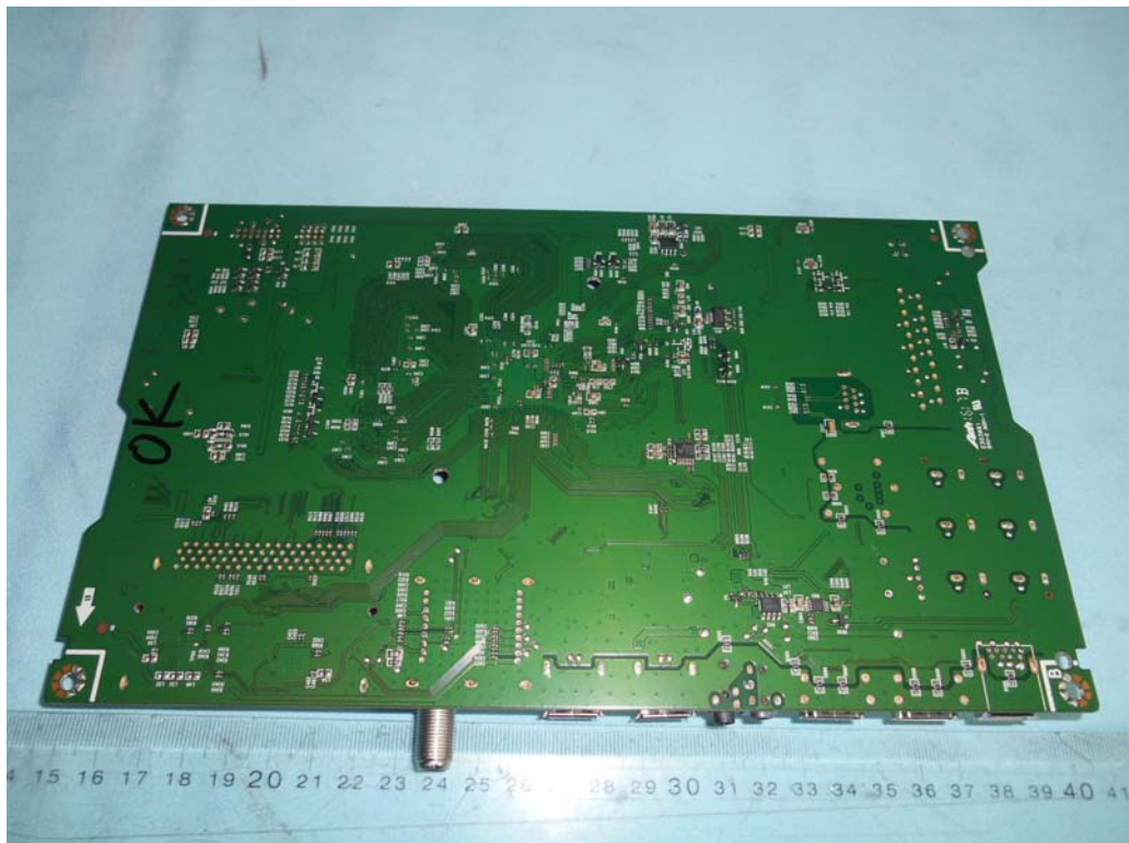
FIGURE 4 LED LCD TV (M/N: LC-55N7000U) MAIN BOARD (SOLDERED SIDE)
