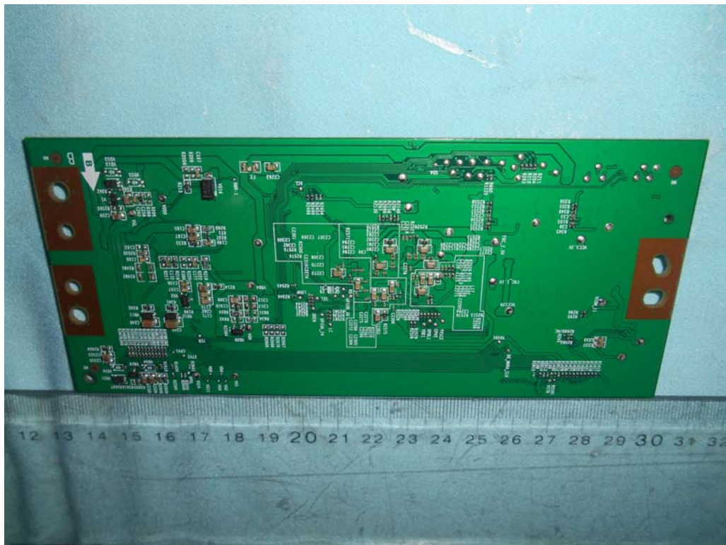
FIGURE 22 LED LCD TV (M/N: LC-55N7000U) CONTROL BOARD (SOLDERED SIDE)
