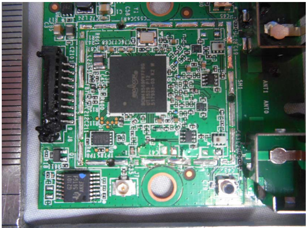
FIGURE 16 LED LCD TV (M/N: HU55K5500UWG) CHIP & CRYSTAL ON RF BOARD
