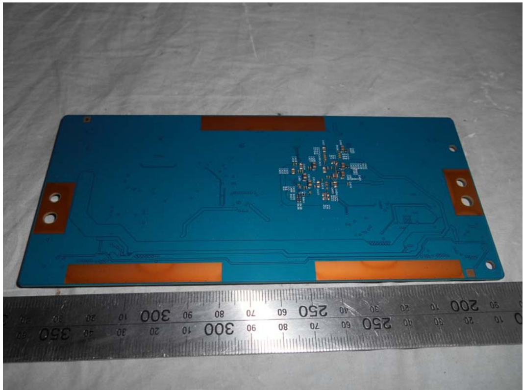
FIGURE 4 LED LCD TV (M/N: HU55K3300UWG) PANEL BOARD (SOLDERED SIDE)
