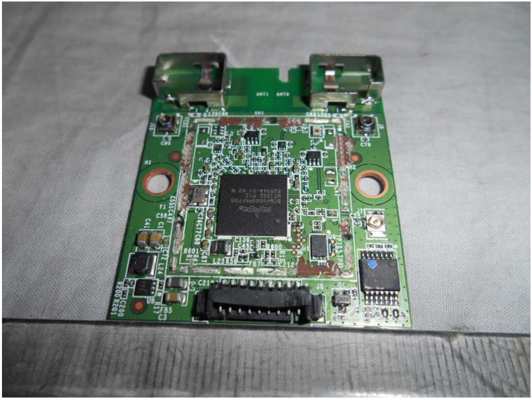
FIGURE 22 LED LCD TV (M/N: HU55K3300UWG) RF BOARD COVER REMOVED
