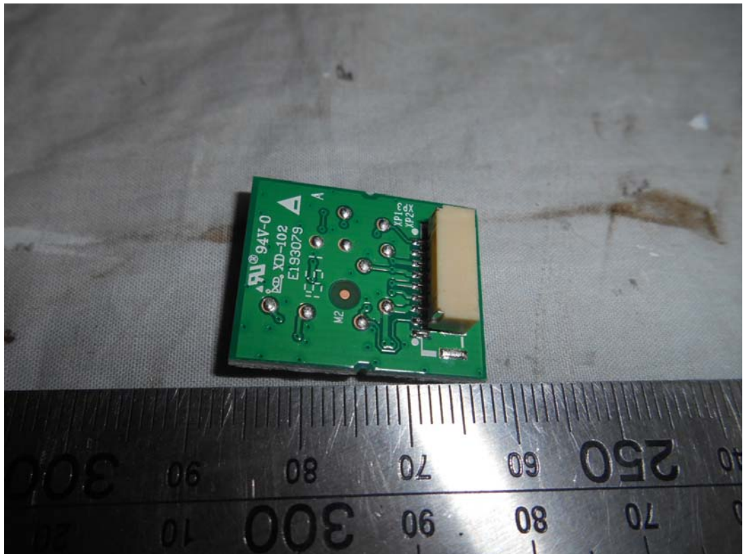
FIGURE 16 LED LCD TV (M/N: HU55K3300UWG) IR BOARD (SOLDERED SIDE)
