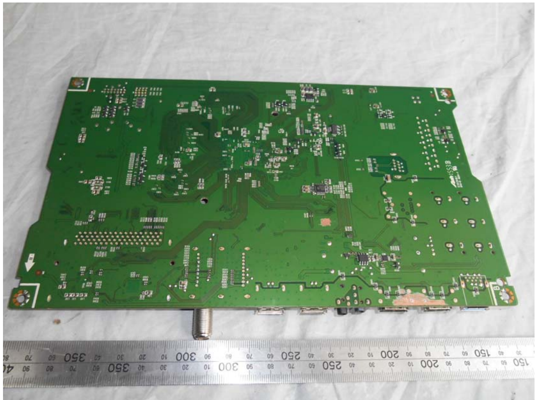
FIGURE 8 LED LCD TV (M/N: HU55K3300UWG) CHIP & CRYSTAL ON MAIN BOARD
