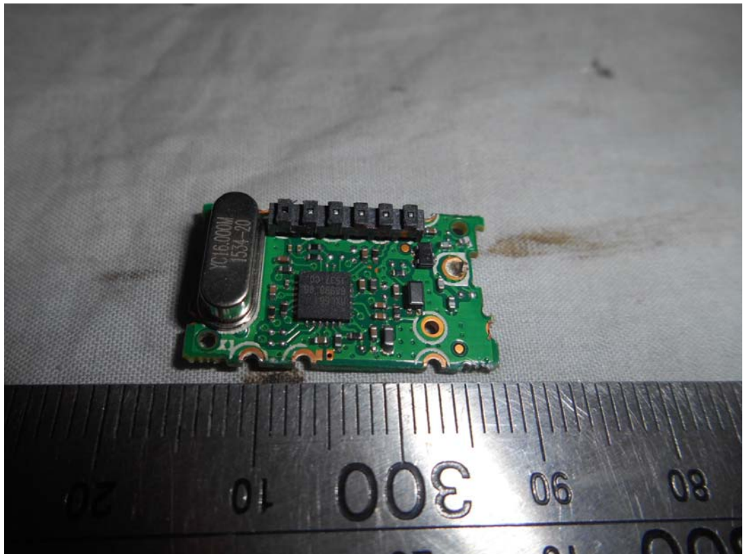
FIGURE 12 LED LCD TV (M/N: HU55K3300UWG) TUNER BOARD (COMPONENT SIDE)
