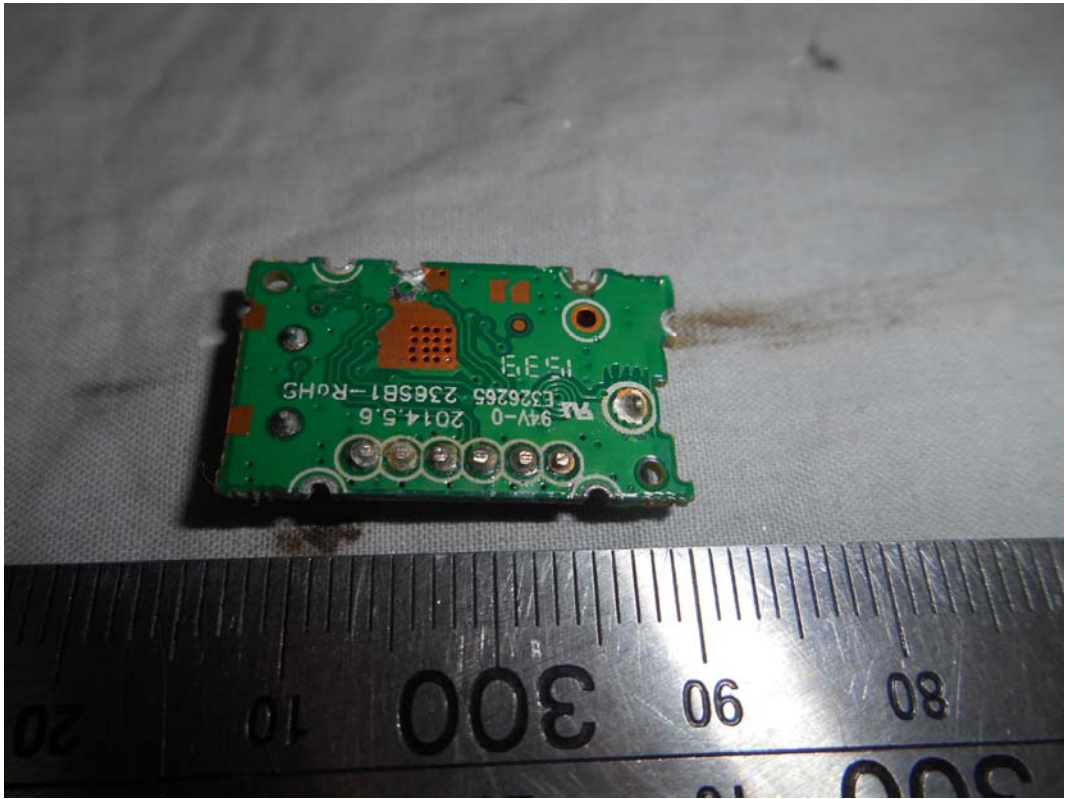
FIGURE 14 LED LCD TV (M/N: HU55K3300UWG) CHIP & CRYSTAL ON TUNER BOARD
