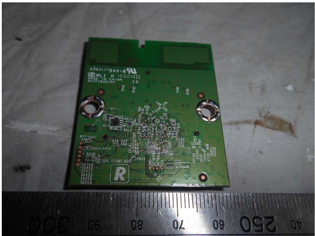
FIGURE 20 LED LCD TV (M/N: HU55K3300UWG) RF BOARD (SOLDERED SIDE)
