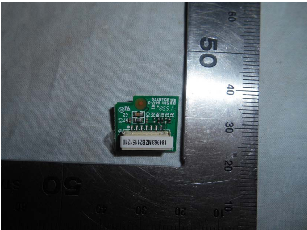
FIGURE 22 LED LCD TV (M/N: 55K2203W) IR BOARD (SOLDERED SIDE)
