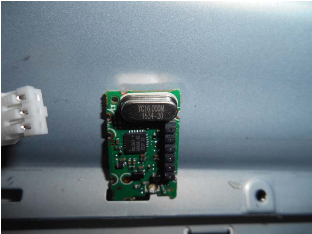
FIGURE 9 LED LCD TV (M/N: 55K2203W) TUNER CRYSTAL ON MAIN BOARD
