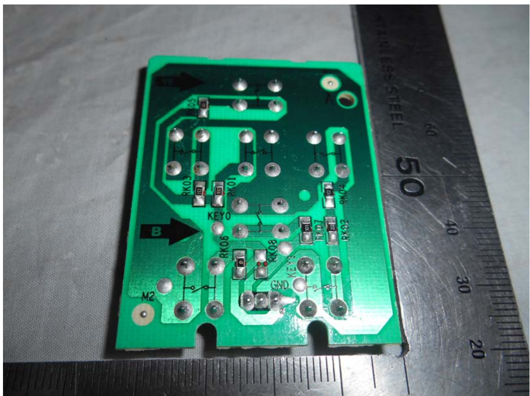
FIGURE 20 LED LCD TV (M/N: 55K2203W) KEY BOARD (SOLDERED SIDE)
