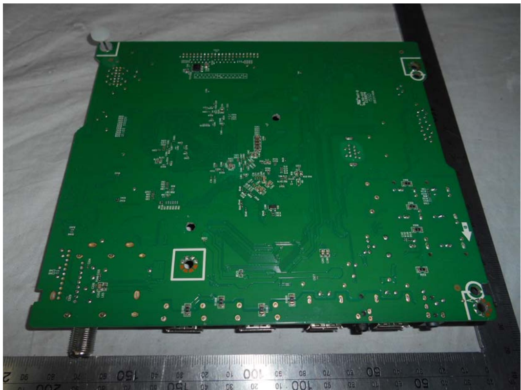
FIGURE 4 LED LCD TV (M/N: 55K2203W) MAIN BOARD (SOLDERED SIDE)
