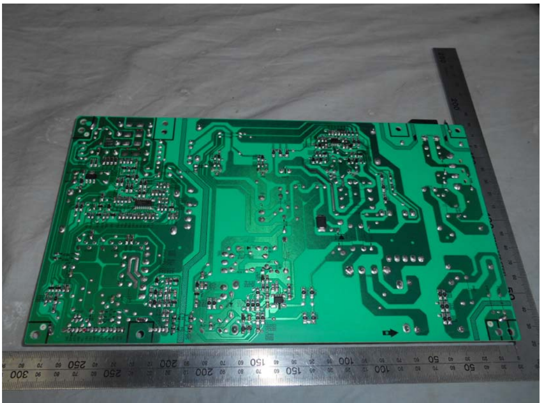
FIGURE 18 LED LCD TV (M/N: 55K2203W) POWER BOARD (SOLDERED SIDE)
