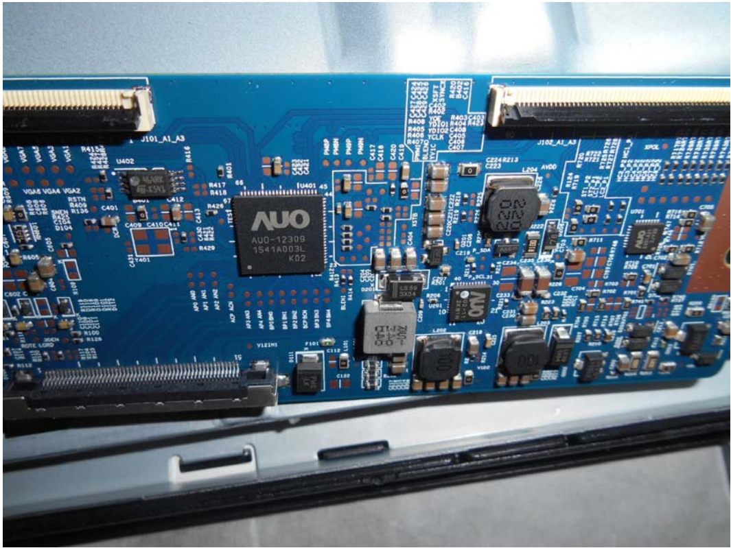
FIGURE 12 LED LCD TV (M/N: 55K2203W) CHIP & CRYSTAL ON PANEL BOARD
