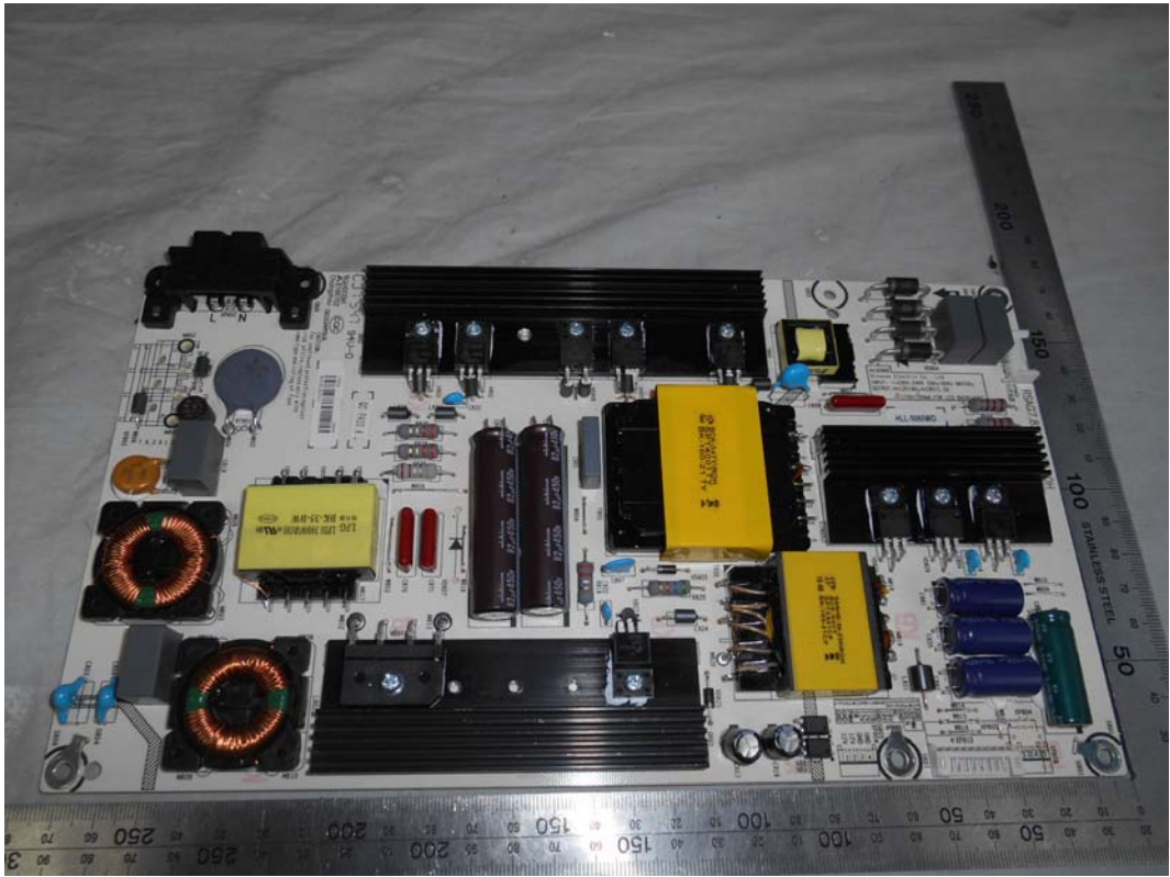
FIGURE 17 LED LCD TV (M/N: 55K2203W) POWER BOARD (COMPONENT SIDE)
