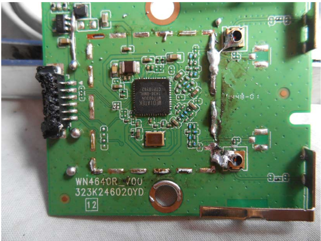
FIGURE 16 LED LCD TV (M/N: 55K2203W) CHIP & CRYSTAL ON RF BOARD
