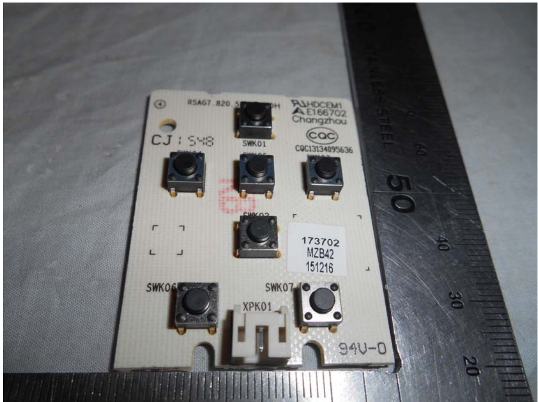
FIGURE 19 LED LCD TV (M/N: 55K2203W) KEY BOARD (COMPONENT SIDE)
