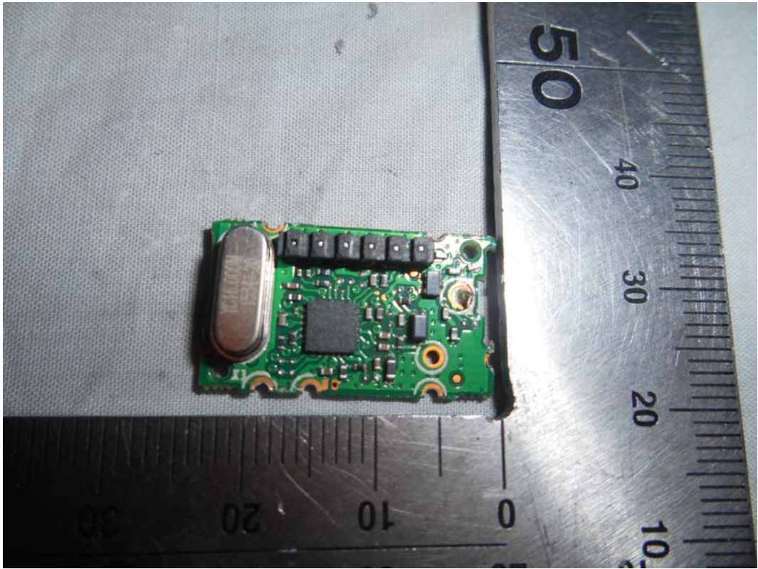
FIGURE 7 LED LCD TV (M/N: 55K2203W) TUNER BOARD (COMPONENT SIDE)
