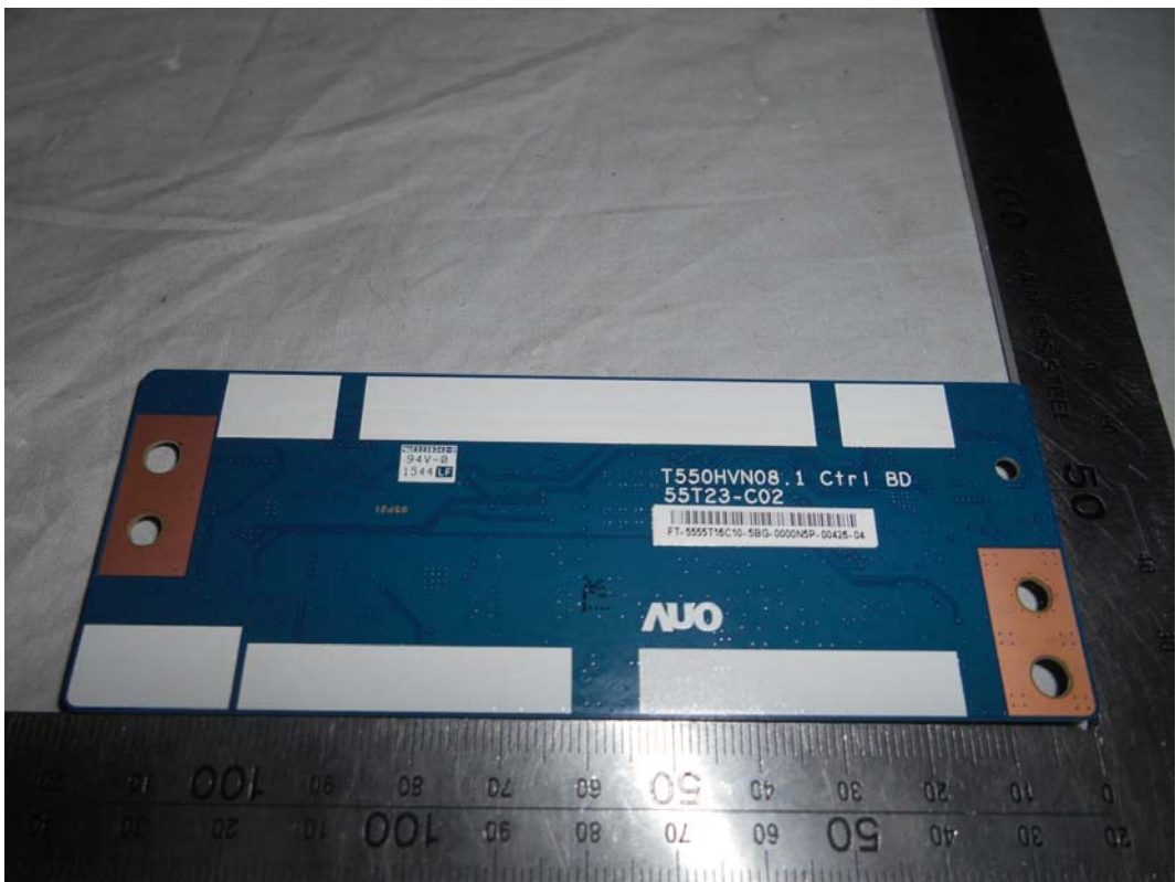
FIGURE 11 LED LCD TV (M/N: 55K2203W) PANEL BOARD (SOLDERED SIDE)
