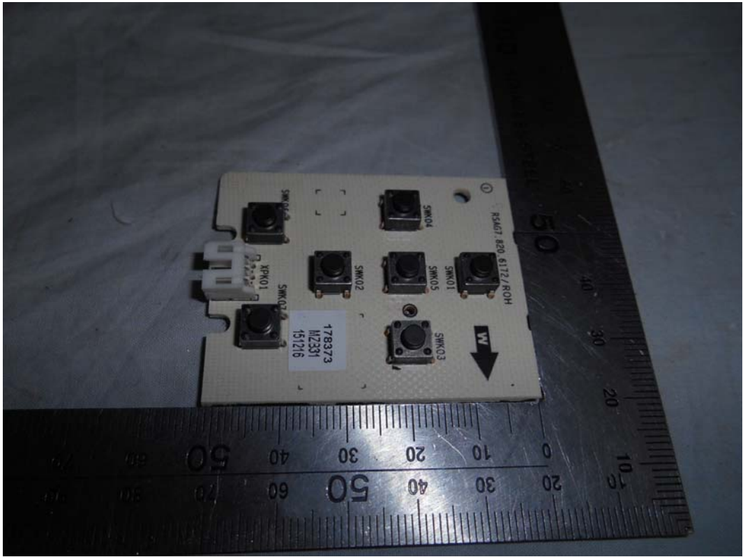
FIGURE 19 LED LCD TV (M/N: 50K2203W) KEY BOARD (COMPONENT SIDE)
