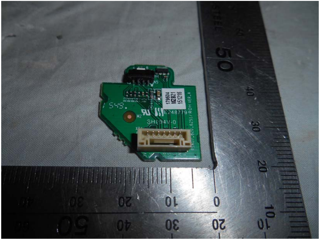
FIGURE 21 LED LCD TV (M/N: 50K2203W) IR BOARD (COMPONENT SIDE)
