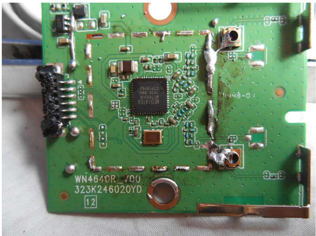
FIGURE 16 LED LCD TV (M/N: 50K2203W) CHIP & CRYSTAL ON RF BOARD
