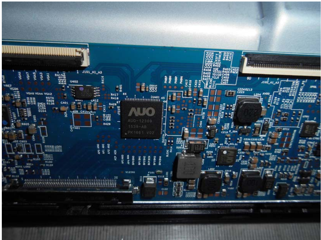
FIGURE 12 LED LCD TV (M/N: 50K2203W) CHIP & CRYSTAL ON PANEL BOARD
