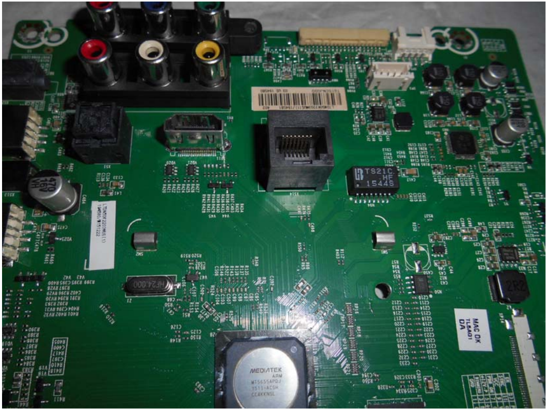
FIGURE 23 LED LCD TV (M/N: 50K2203W) DEBUG
