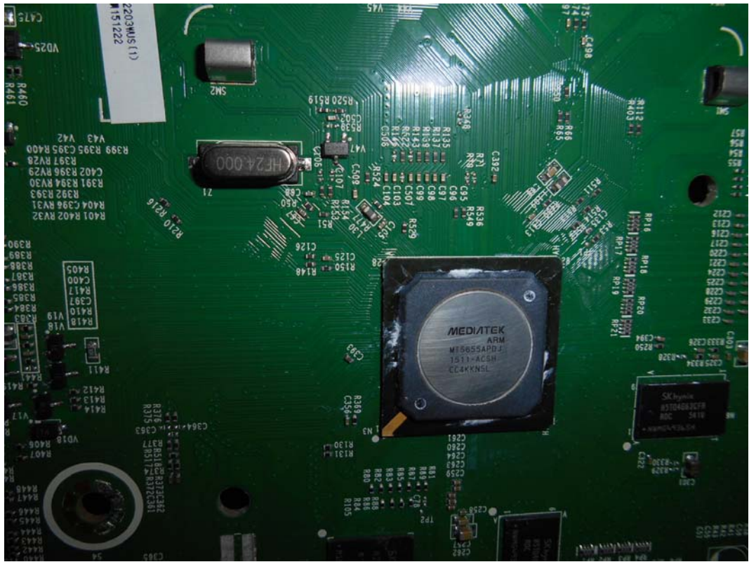
FIGURE 5 LED LCD TV (M/N: 50K2203W) CHIP AND CRYSTAL ON MAIN BOARD
