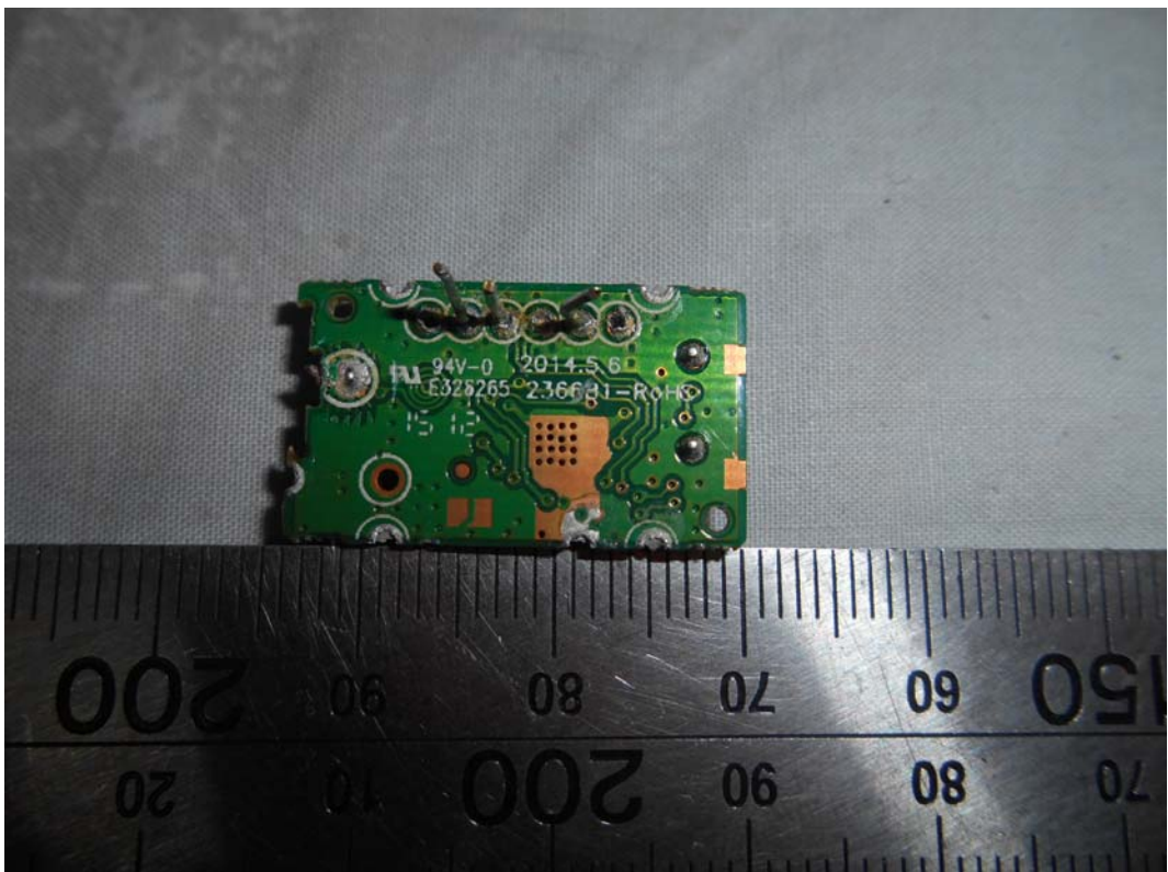
FIGURE 8 LED LCD TV (M/N: 50K2203W) TUNER BOARD (SOLDERED SIDE)
