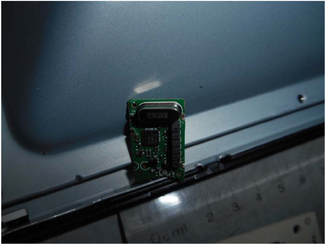
FIGURE 9 LED LCD TV (M/N: 50K2203W) TUNER CRYSTAL ON MAIN BOARD
