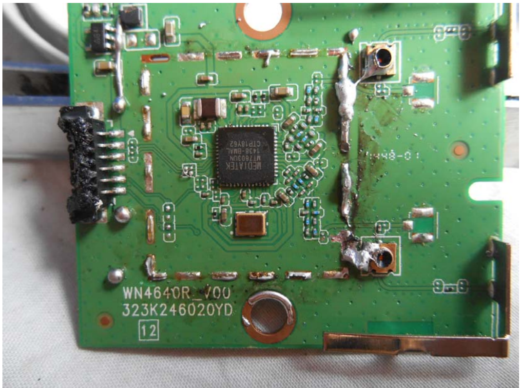
FIGURE 13 LED LCD TV (M/N: HU50K300FW) CHIP & CRYSTAL ON RF BOARD
