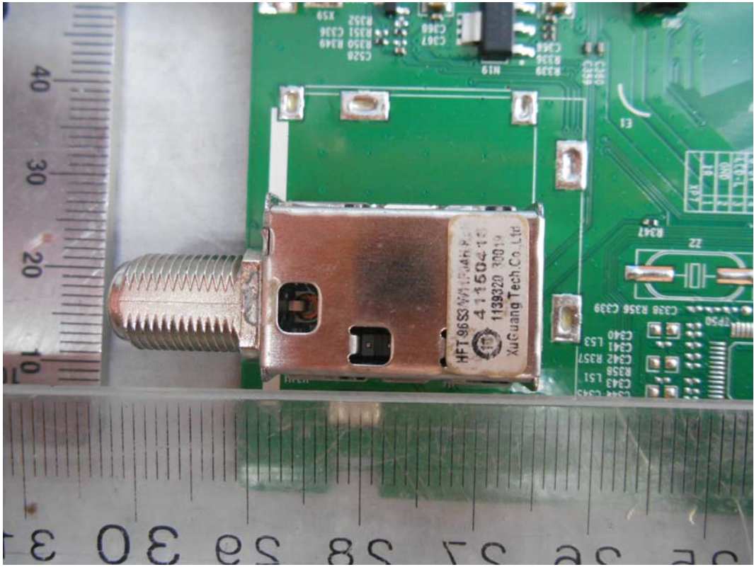
FIGURE 7 LED LCD TV (M/N: HU50K300FW) TUNER
