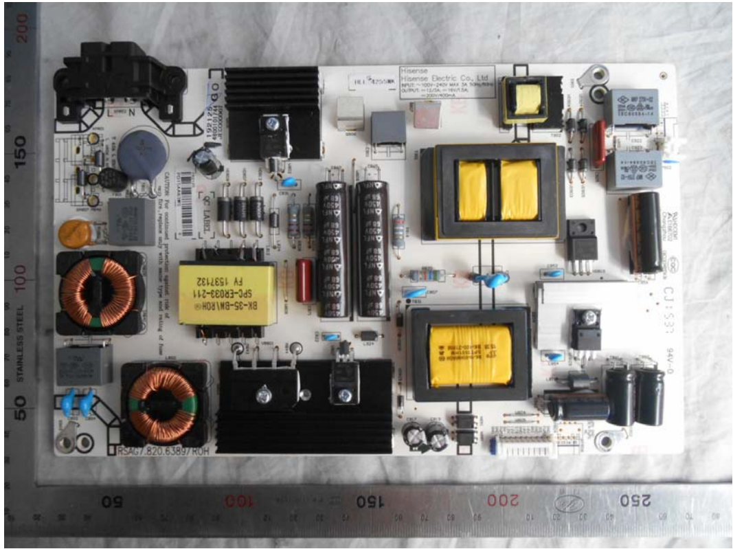
FIGURE 20 LED LCD TV (M/N: HU50K300FW) POWER BOARD (COMPONENT SIDE)
