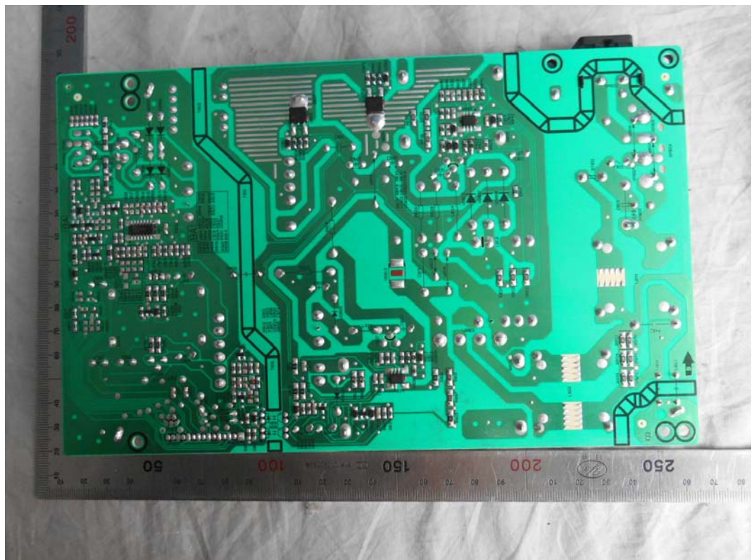
FIGURE 21 LED LCD TV (M/N: HU50K300FW) POWER BOARD (SOLDERED SIDE)
