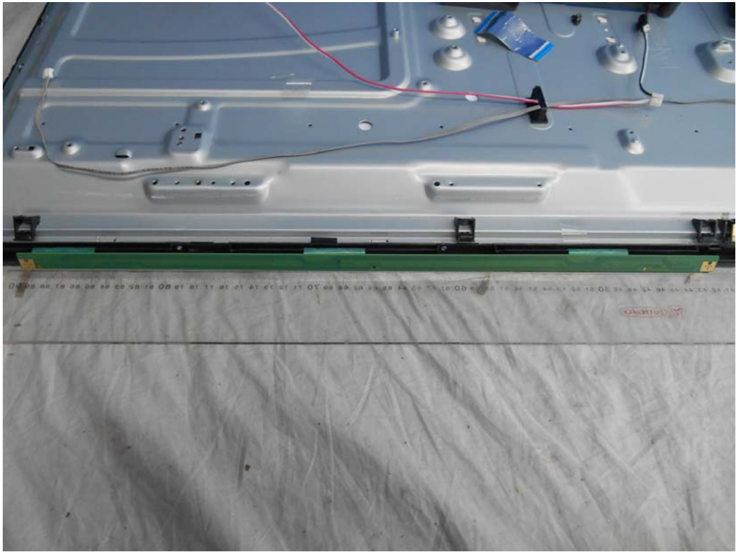
FIGURE 22 LED LCD TV (M/N: HU50K300FW) SIGNAL BOARD#1 (COMPONENT SIDE)
