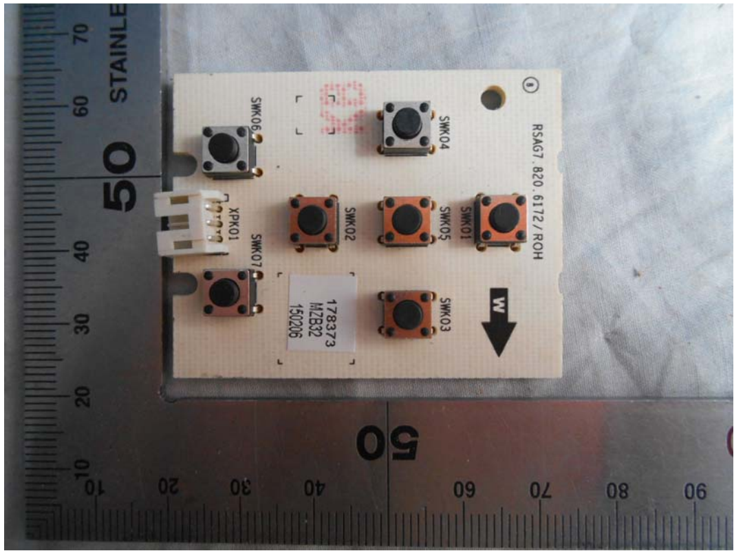
FIGURE 16 LED LCD TV (M/N: HU50K300FW) KEY BOARD (COMPONENT SIDE)
