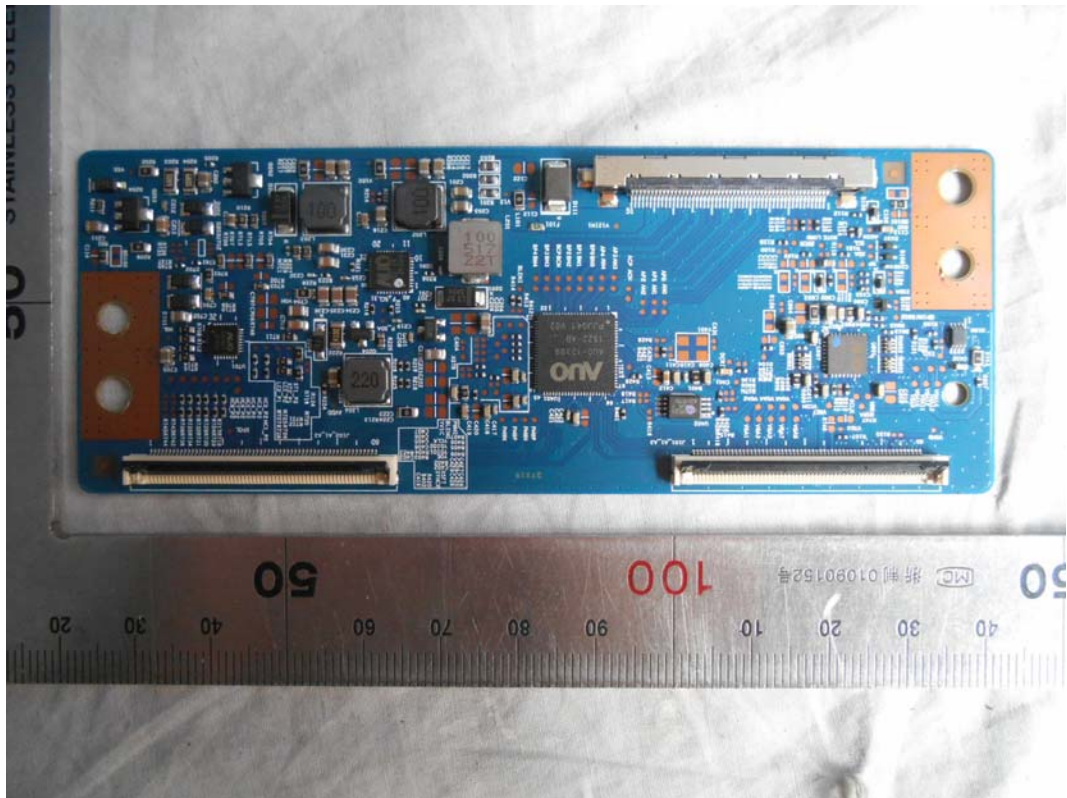
FIGURE 14 LED LCD TV (M/N: HU50K300FW) CONTROL BOARD (COMPONENT SIDE)
