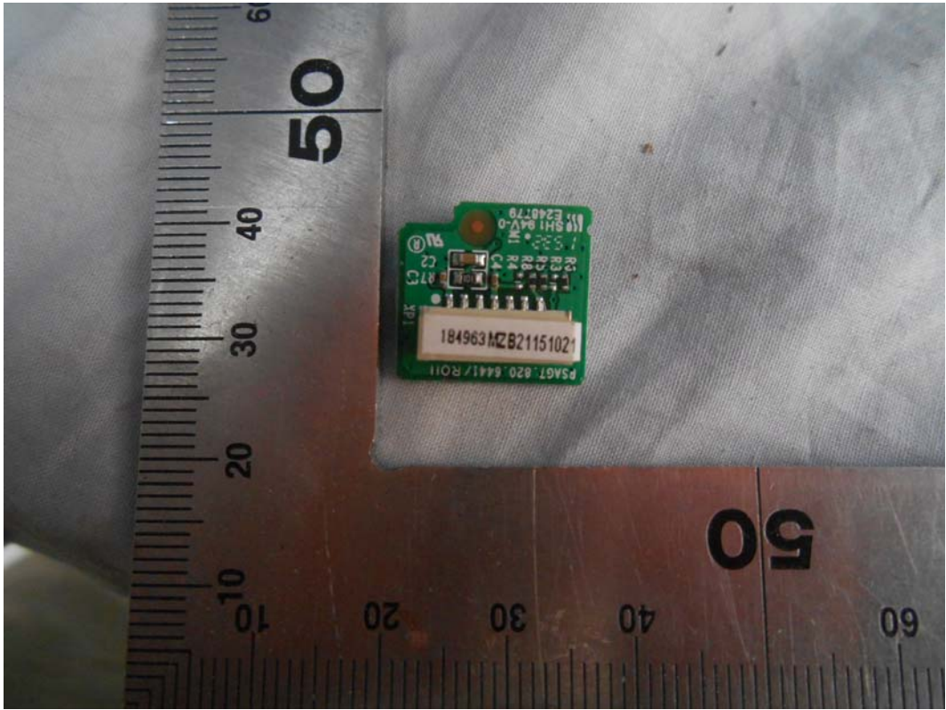
FIGURE 18 LED LCD TV (M/N: HU50K300FW) IR BOARD (COMPONENT SIDE)
