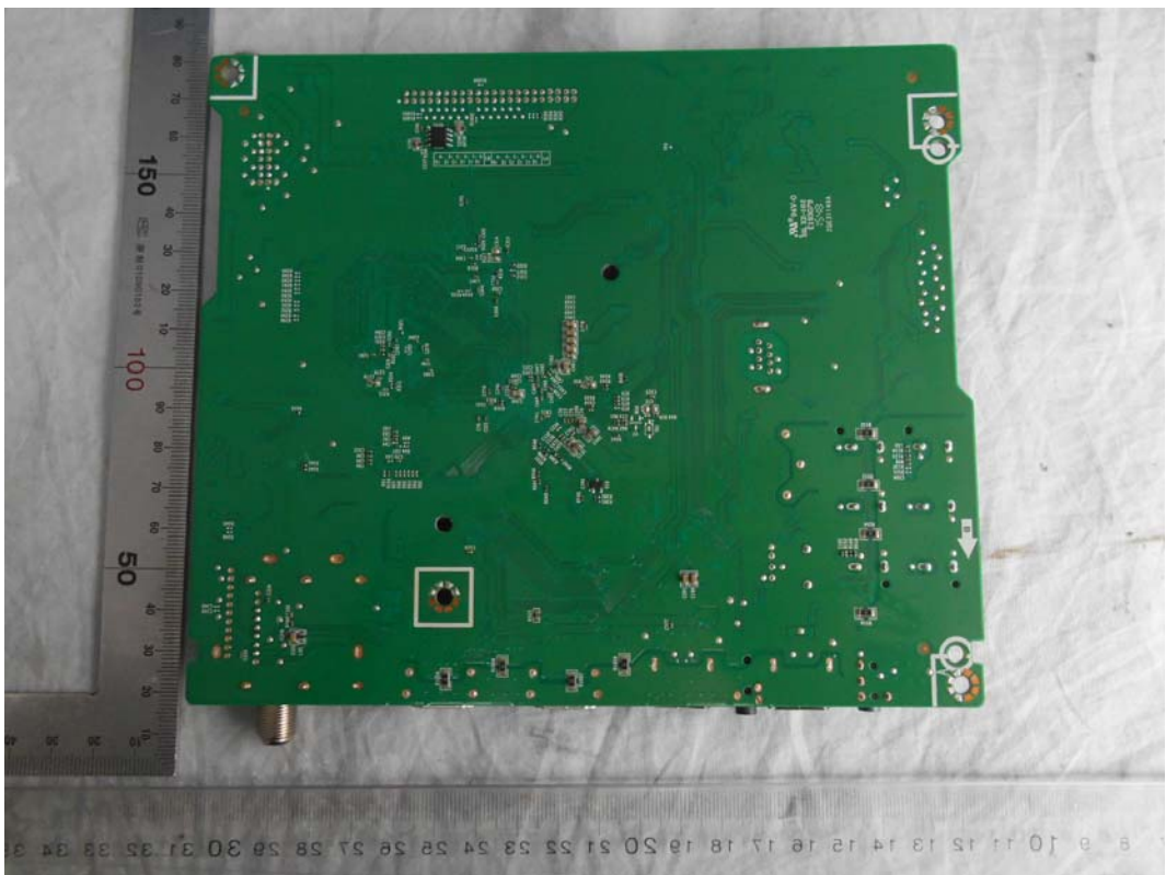
FIGURE 5 LED LCD TV (M/N: HU50K300FW) MAIN BOARD (SOLDERED SIDE)
