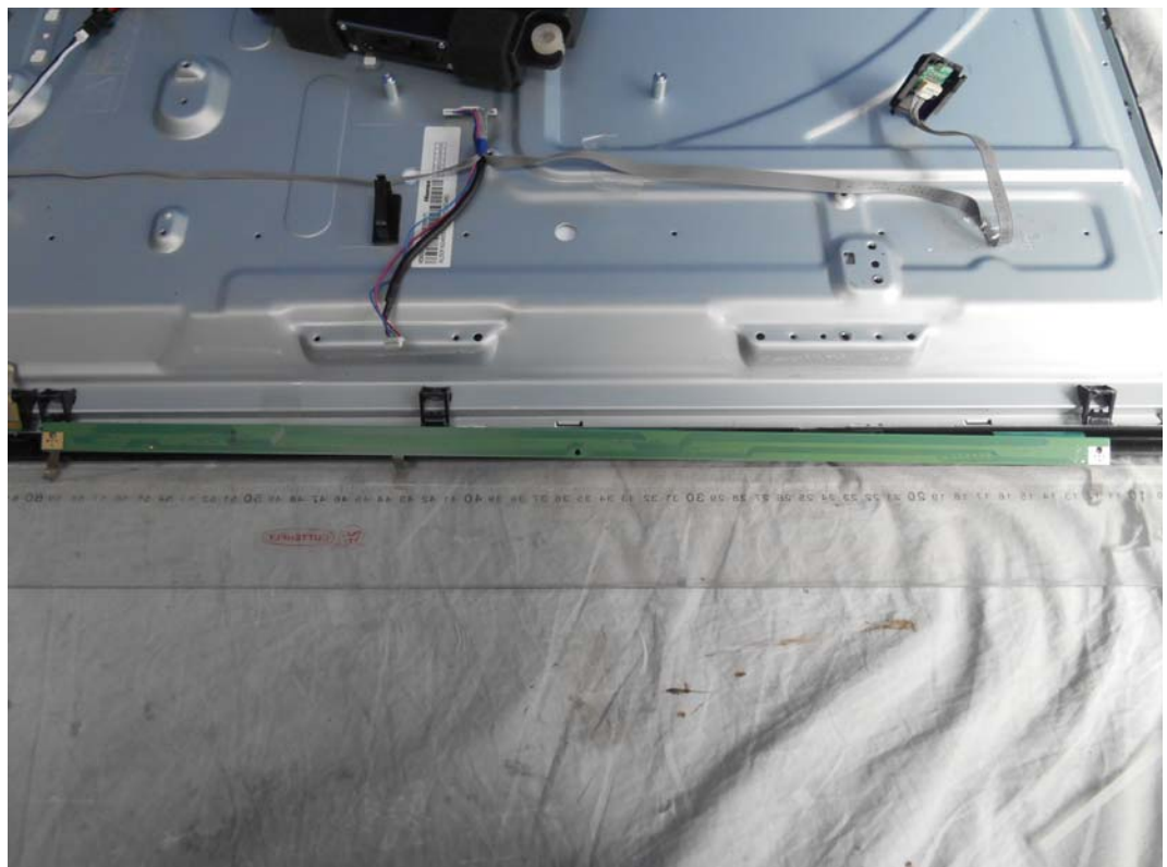
FIGURE 25 LED LCD TV (M/N: HU50K300FW) SIGNAL BOARD#2 (SOLDERED SIDE)
