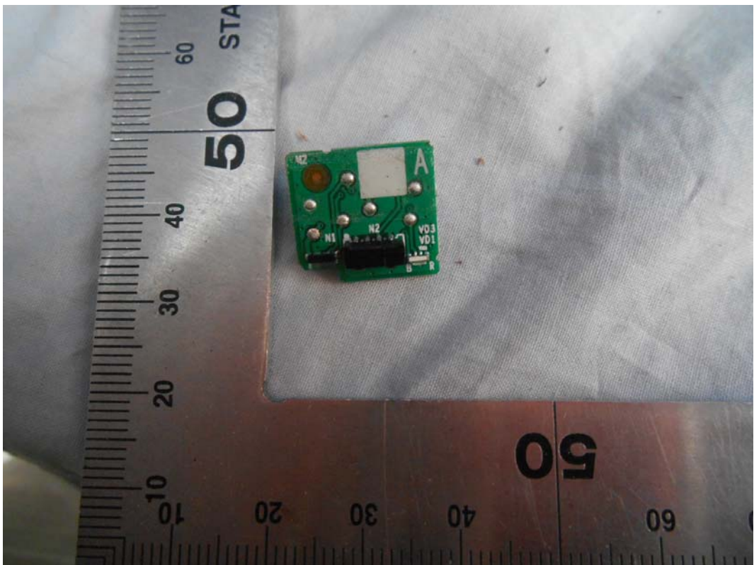
FIGURE 19 LED LCD TV (M/N: HU50K300FW) IR BOARD (COMPONENT SIDE)
