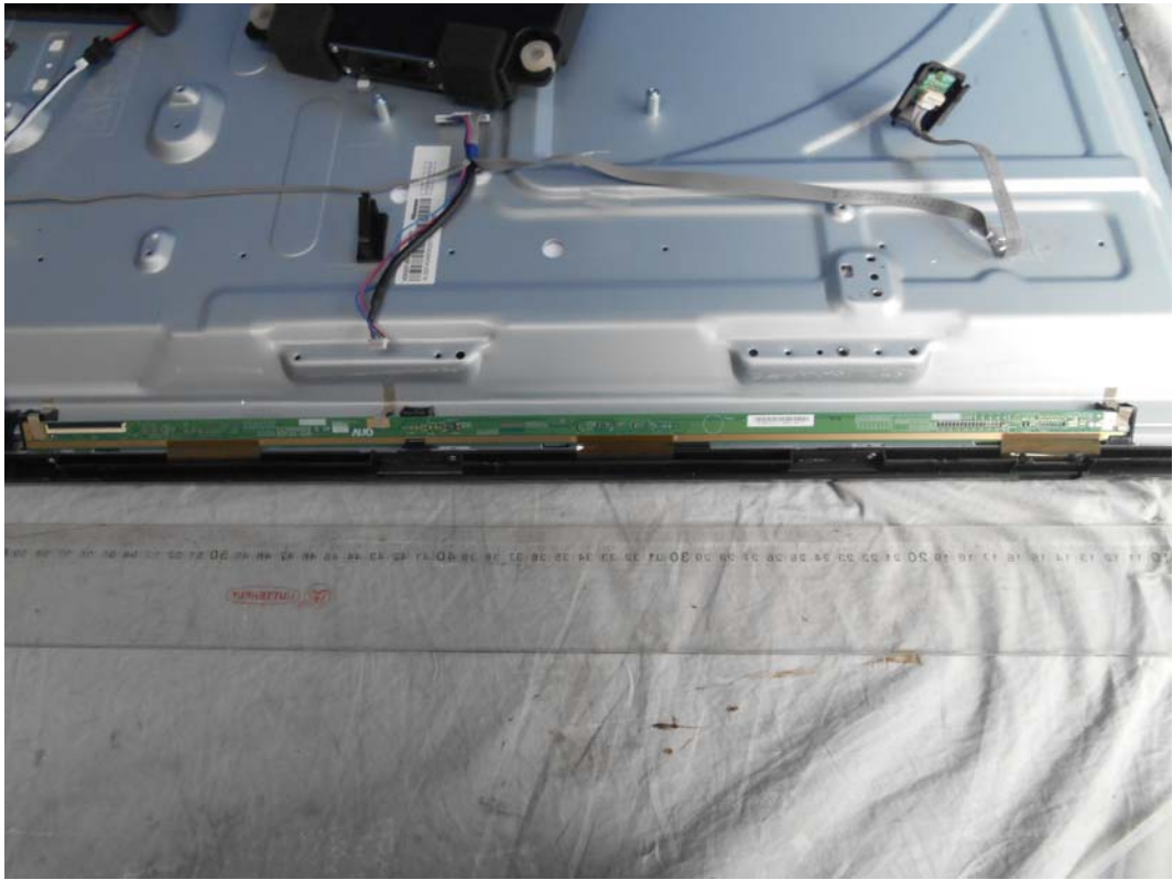
FIGURE 24 LED LCD TV (M/N: HU50K300FW) SIGNAL BOARD#2 (COMPONENT SIDE)
