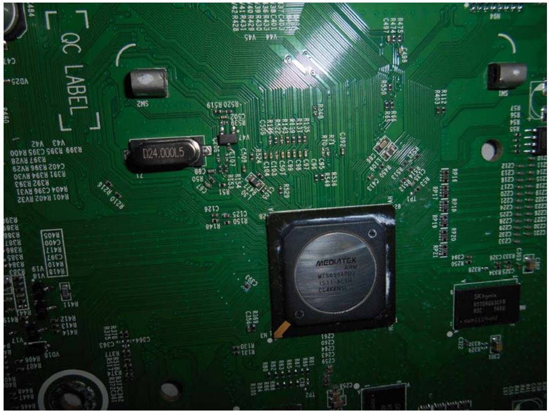
FIGURE 6 LED LCD TV (M/N: HU50K300FW) CHIP & CRYSTAL ON MAIN BOARD
