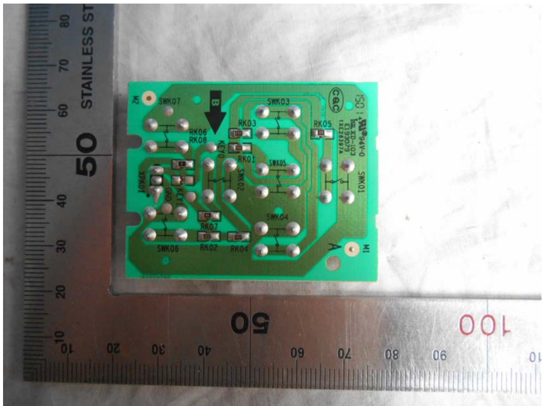
FIGURE 17 LED LCD TV (M/N: HU50K300FW) KEY BOARD (COMPONENT SIDE)
