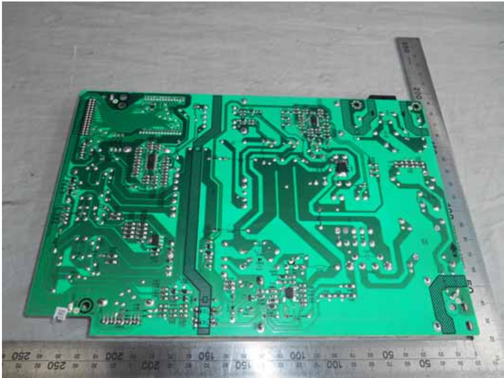
FIGURE 19 LED LCD TV (M/N: HU50K3300UWG) POWER BOARD (SOLDERED SIDE)
