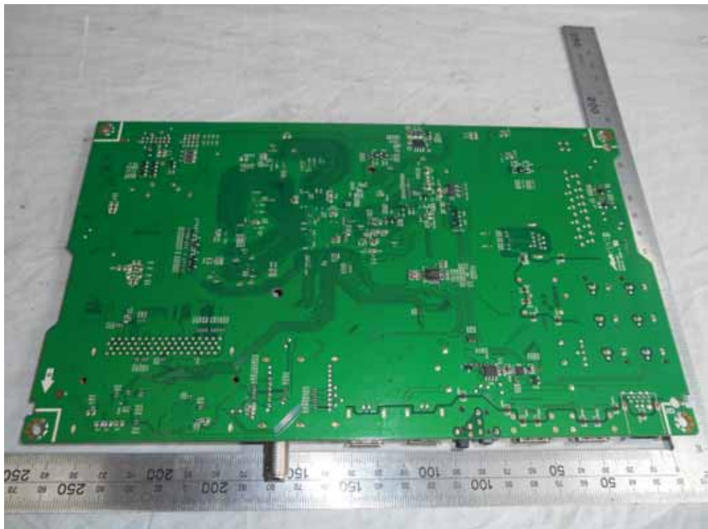
FIGURE 4 LED LCD TV (M/N: HU50K3300UWG) MAIN BOARD (SOLDERED SIDE)
