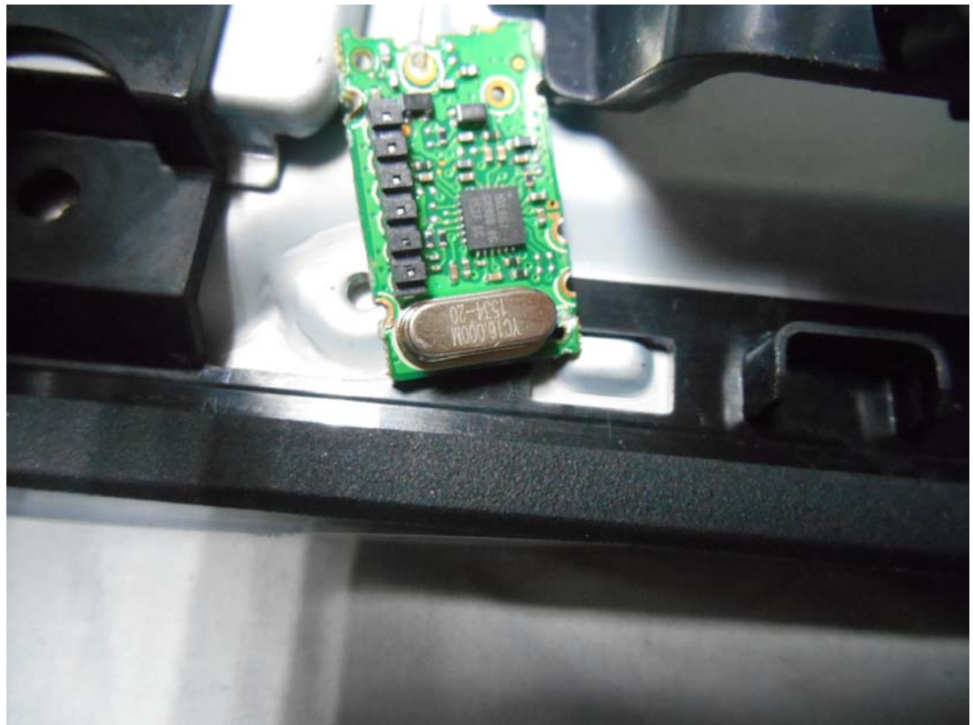
FIGURE 9 LED LCD TV (M/N: HU55K5500UWG) TUNER CRYSTAL ON MAIN BOARD
