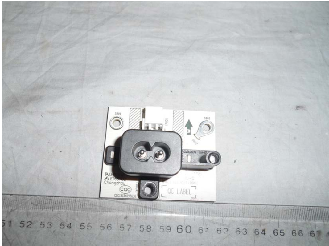
FIGURE 20 LED LCD TV (M/N: LTDN75K700GUWUS) AC BOARD (COMPONENT SIDE)
