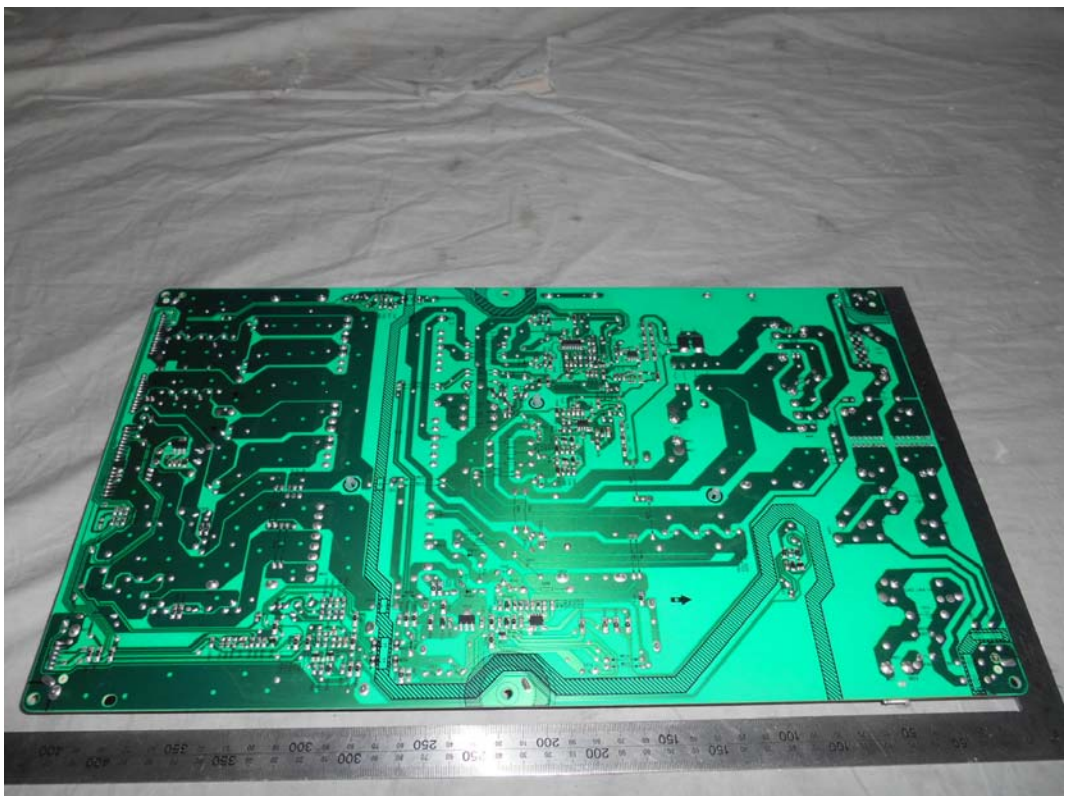
FIGURE 19 LED LCD TV (M/N: LTDN75K700GUWUS) POWER BOARD (SOLDERED SIDE)
