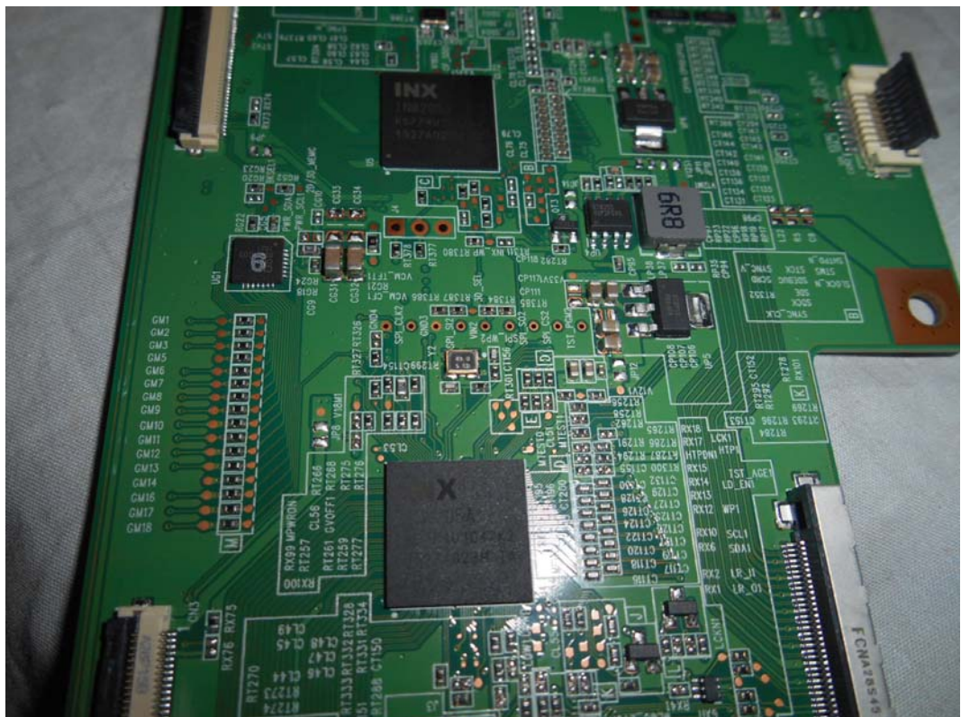
FIGURE 13 LED LCD TV (M/N: LTDN75K700GUWUS) CHIP & CRYSTAL#1 ON PANEL BOARD
