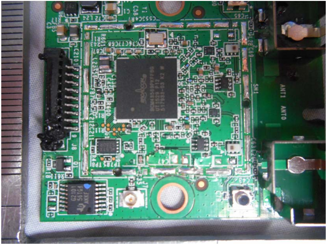
FIGURE 17 LED LCD TV (M/N: LTDN75K700G UWUS) CHIP & CRYSTAL ON RF BOARD
