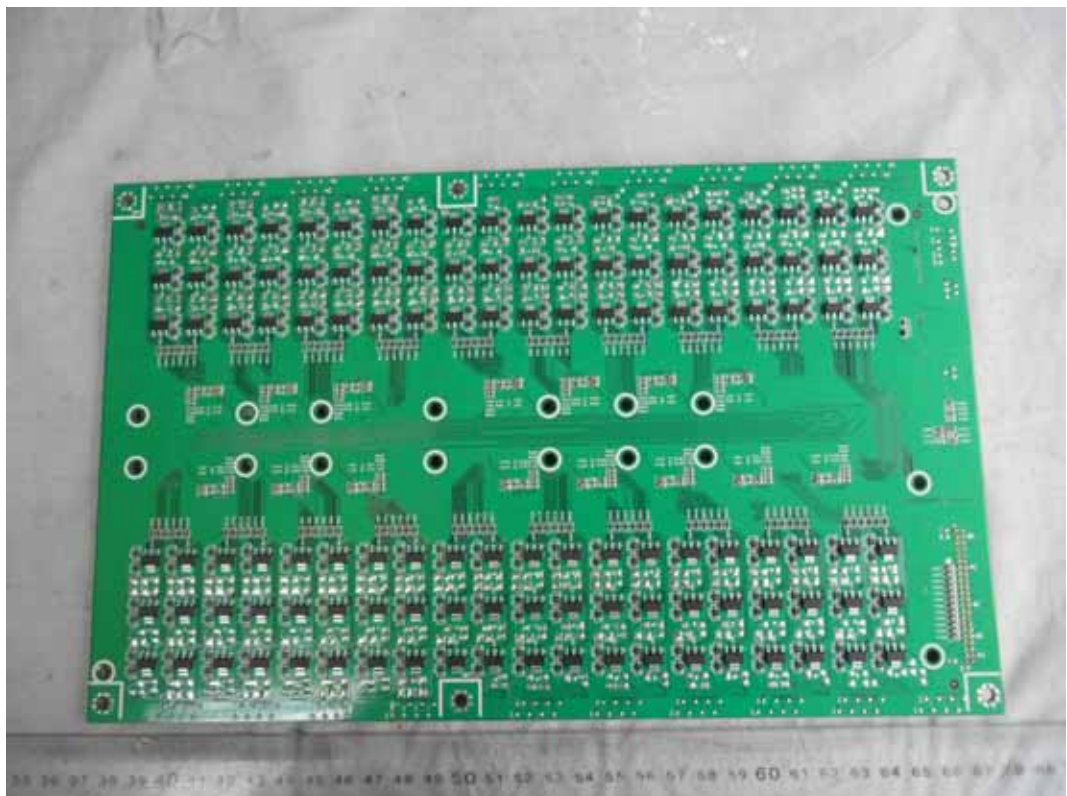
FIGURE 20 LED LCD TV (M/N: 65H10B) SIGNAL BOARD #2 (COMPONENT SIDE)
