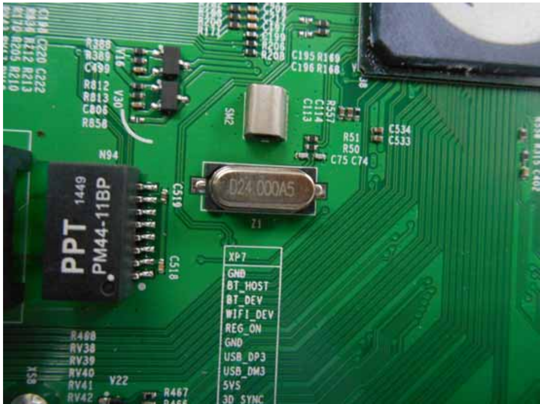
FIGURE 7 LED LCD TV (M/N: 65H10B) CRYSTAL ON MAIN BOARD
