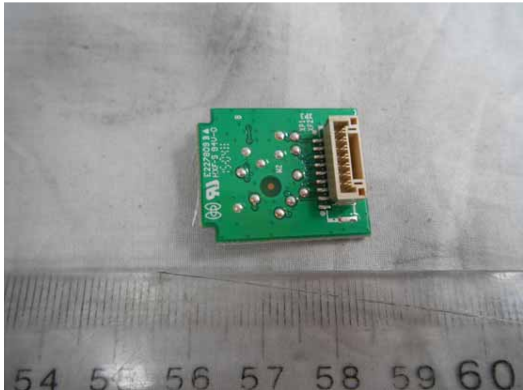
FIGURE 23 LED LCD TV (M/N: 65H10B) INTERFACE BOARD (COMPONENT SIDE)
