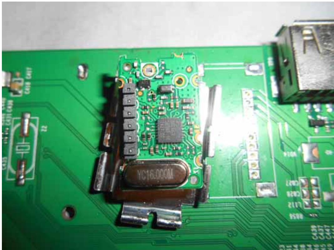
FIGURE 9 LED LCD TV (M/N: 65H10B) TUNER BOARD (COMPONENT SIDE)
