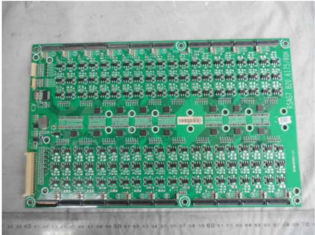
FIGURE 19 LED LCD TV (M/N: 65H10B) SIGNAL BOARD #2 (COMPONENT SIDE)
