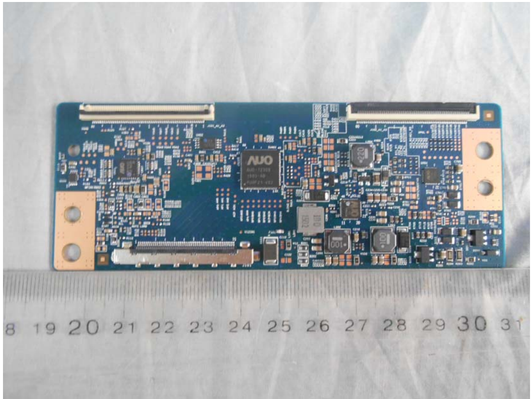
FIGURE 19 LED LCD TV (M/N: LTDN50K220WUS) SIGNAL BOARD (COMPONENT SIDE)
