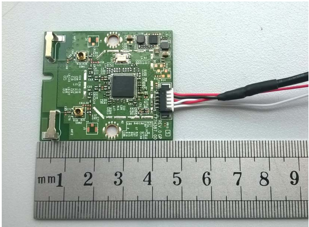
FIGURE 16 LED LCD TV (M/N: LTDN50K220WUS) RF BOARD (COVER REMOVED)
