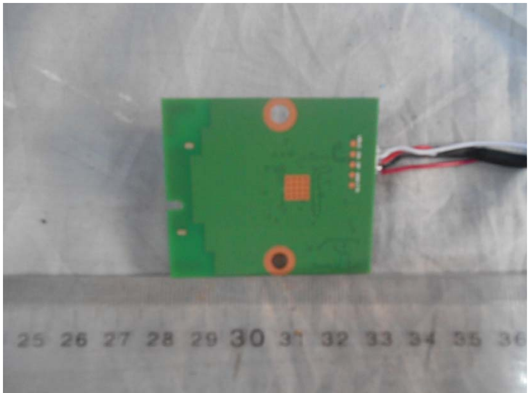
FIGURE 15 LED LCD TV (M/N: LTDN50K220WUS) RF BOARD (SOLDERED SIDE)
