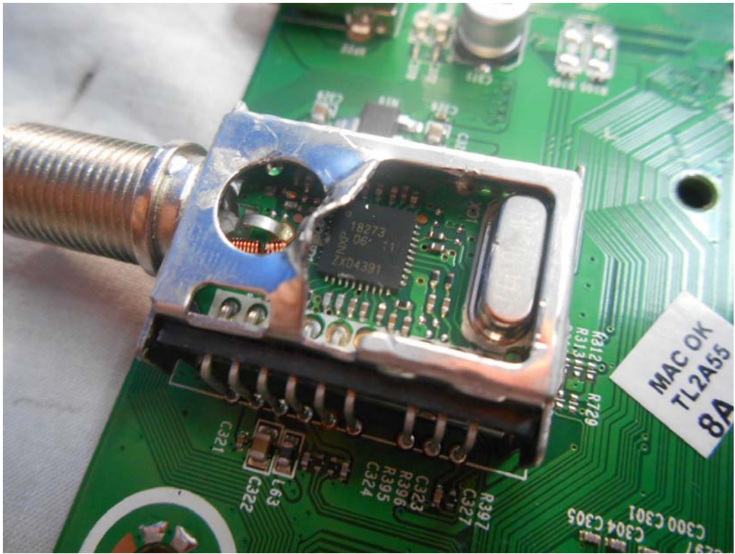
FIGURE 12 LED LCD TV (M/N: LTDN50K220WUS) TUNER ON MAIN BOARD
