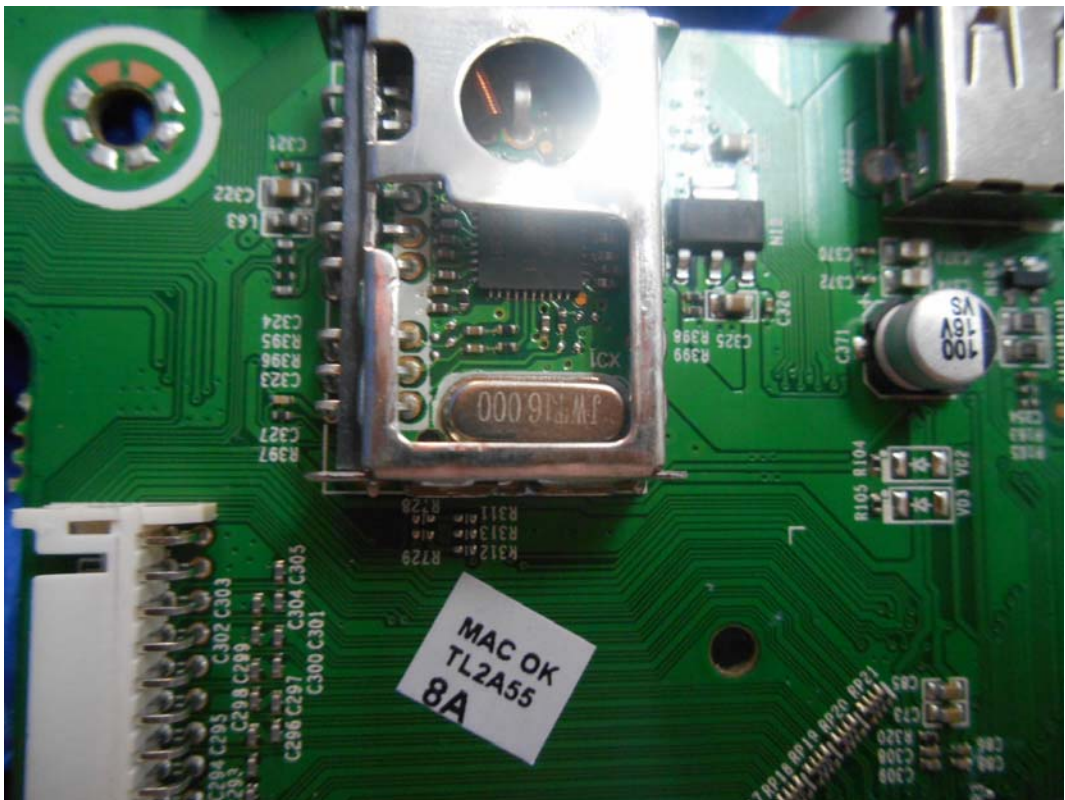
FIGURE 13 LED LCD TV (M/N: LTDN50K220WUS) CRYSTAL ON TUNER
