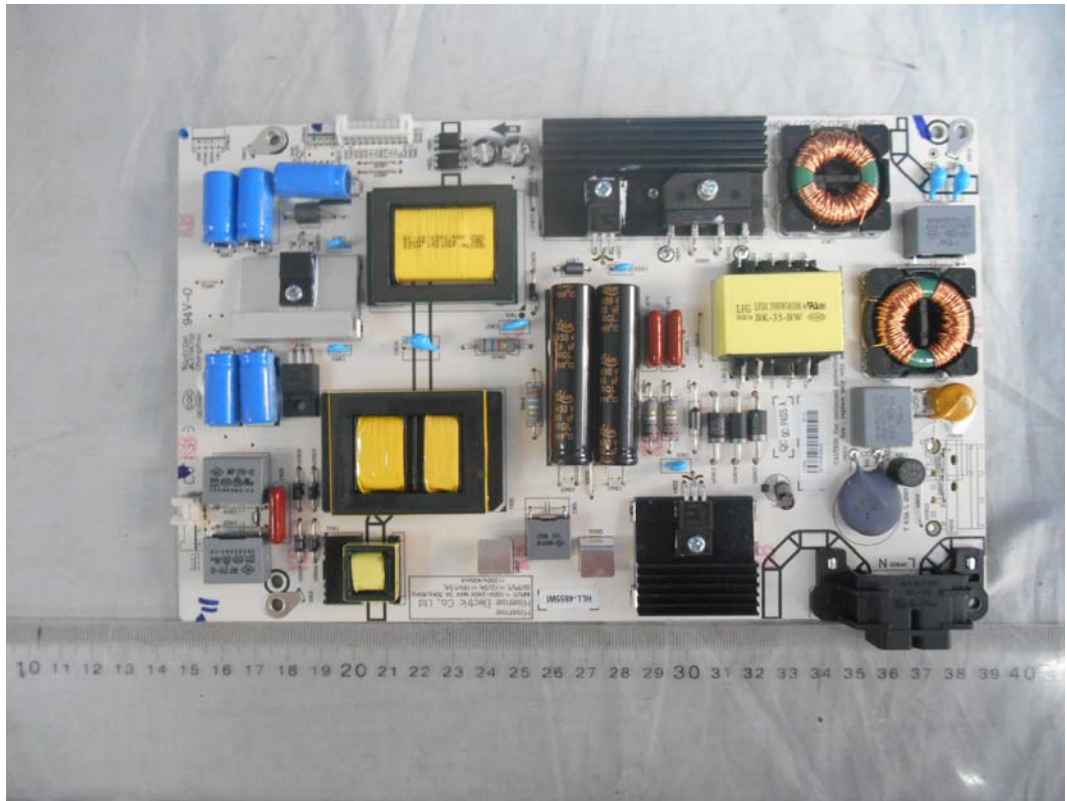
FIGURE 17 LED LCD TV (M/N: LTDN50K220WUS) POWER BOARD (COMPONENT SIDE)
