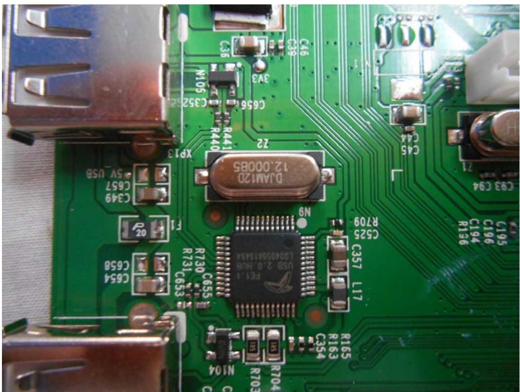
FIGURE 11 LED LCD TV (M/N: LTDN50K220WUS) CHIP #2 & CRYSTAL #2 ON MAIN BOARD
