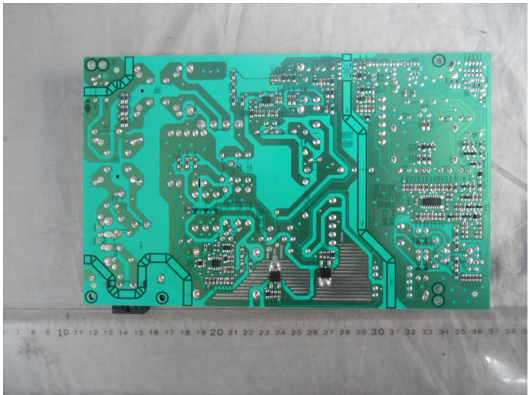
FIGURE 18 LED LCD TV (M/N: LTDN50K220WUS) POWER BOARD (SOLDERED SIDE)
