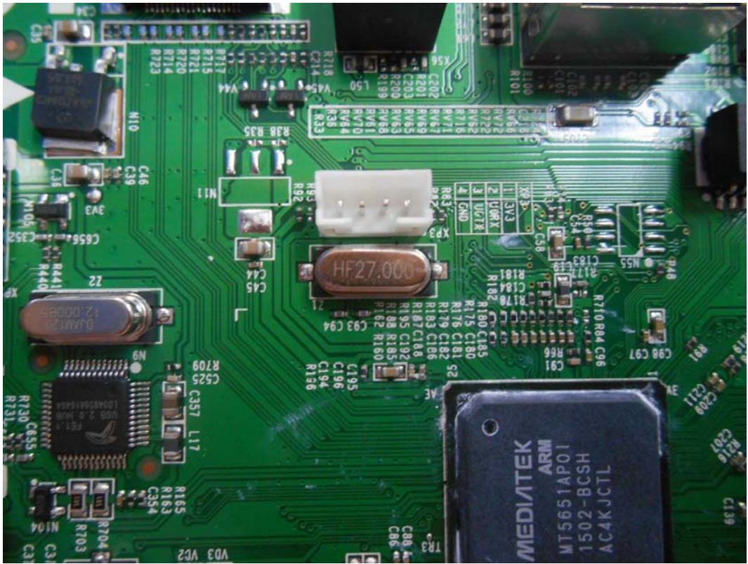
FIGURE 10 LED LCD TV (M/N: LTDN50K220WUS) CHIP #1 & CRYSTAL #1 ON MAIN BOARD
