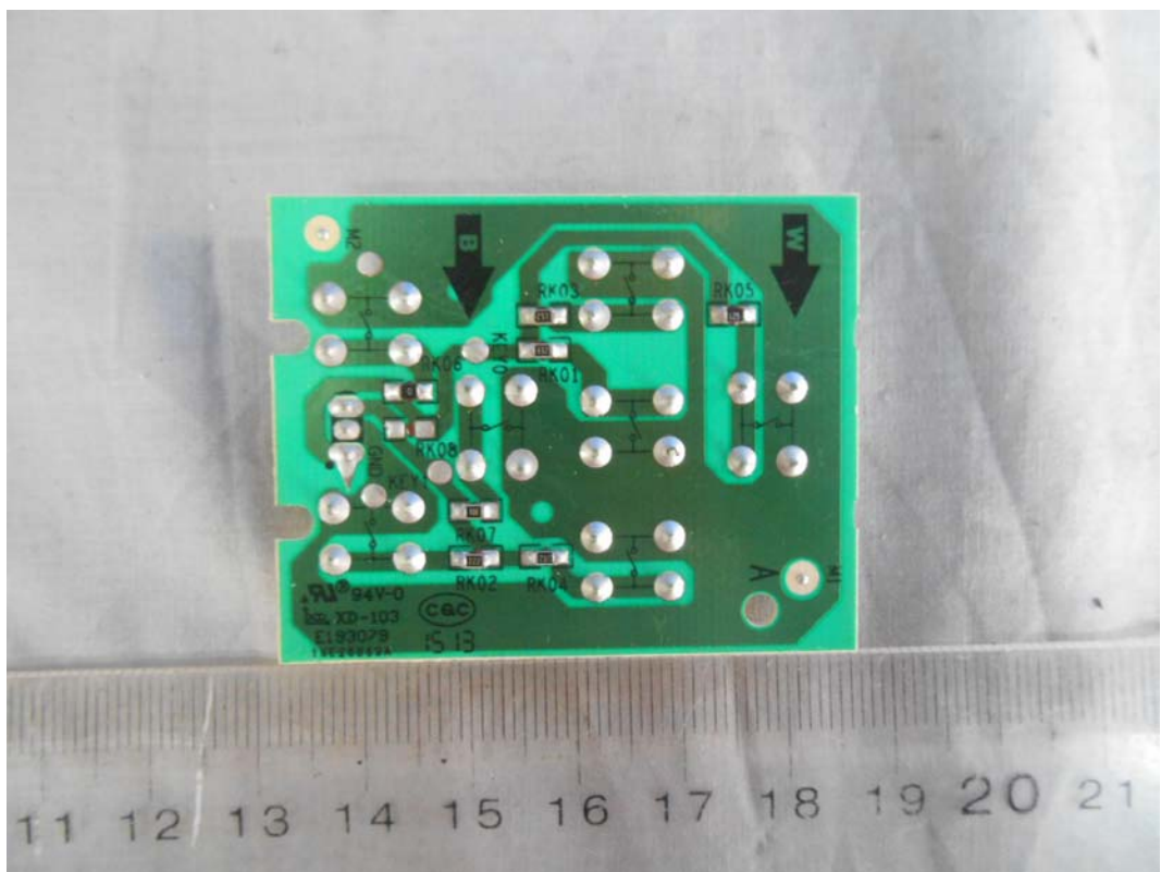
FIGURE 22 LED LCD TV (M/N: LTDN50K220WUS) KEY BOARD (SOLDERED SIDE)
