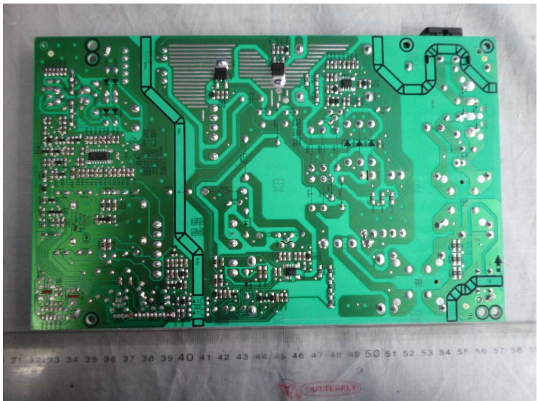
FIGURE 26 LED LCD TV (M/N: LTDN50K2203WUS) POWER BOARD (SOLDERED SIDE)
