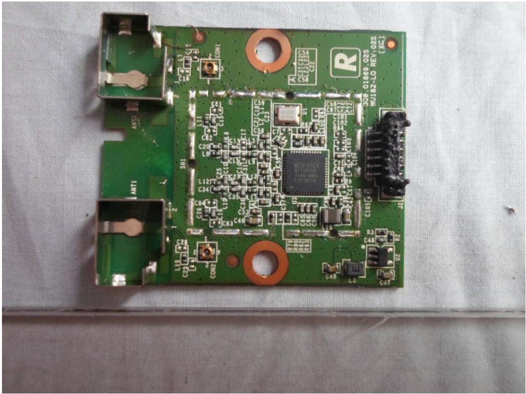
FIGURE 18 LED LCD TV (M/N: LTDN50K2203WUS) RF BOARD (COMPONENT SIDE)
