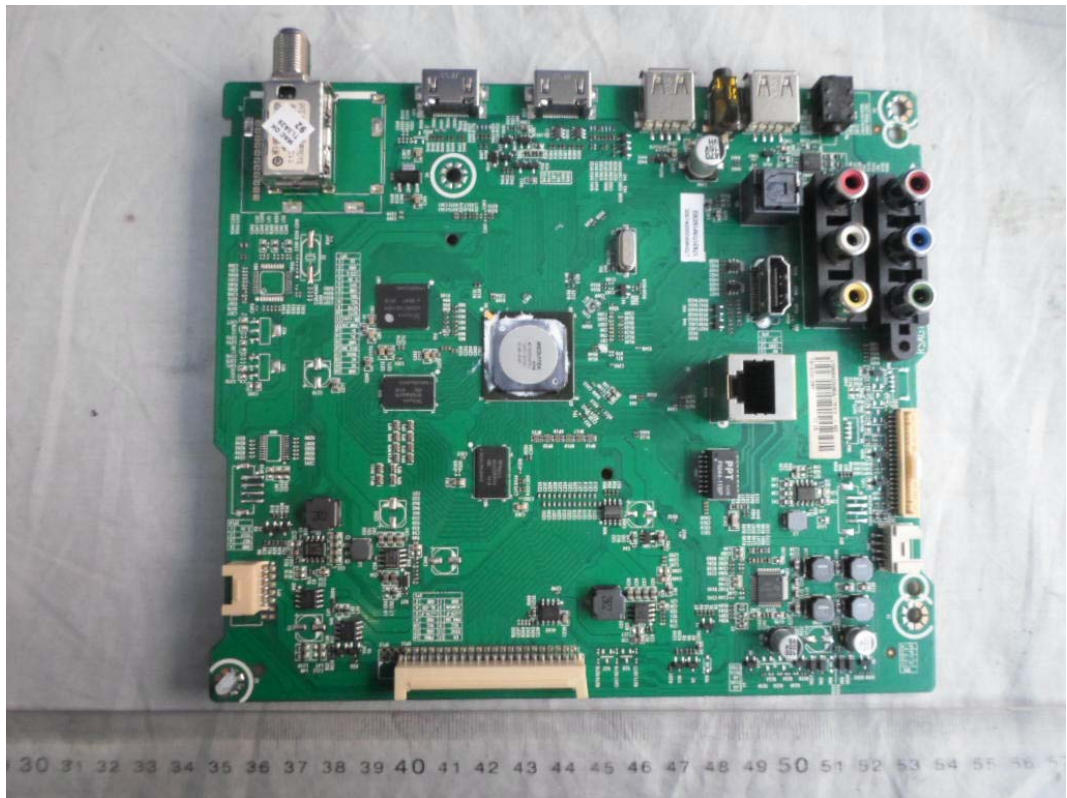
FIGURE 4 LED LCD TV (M/N: LTDN50K2203WUS) MAIN BOARD (COMPONENT SIDE)
