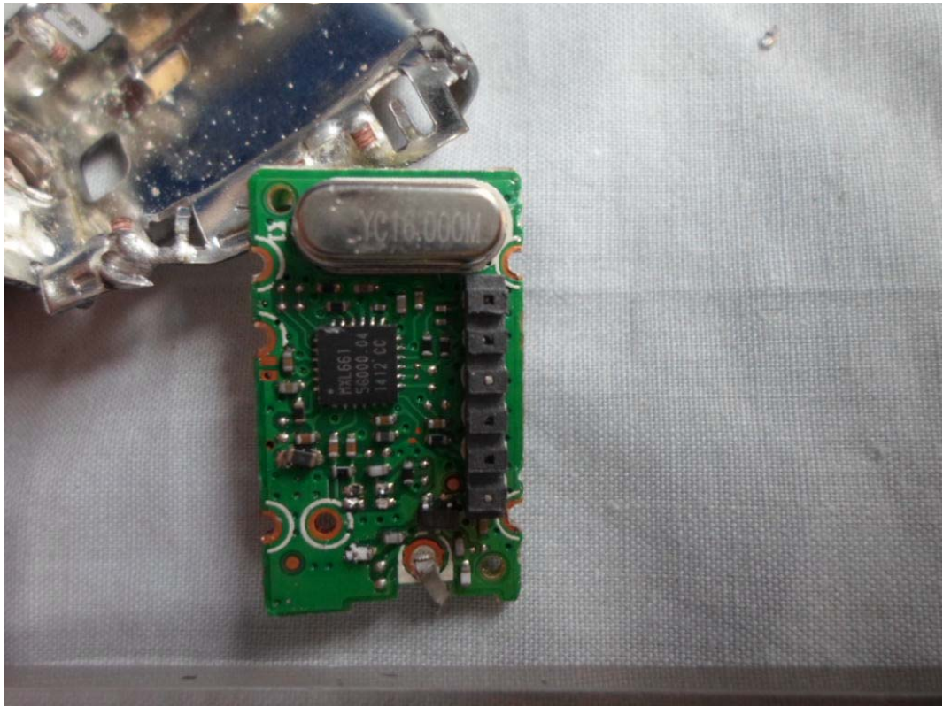
FIGURE 12 LED LCD TV (M/N: LTDN50K2203WUS) CHIP & CRYSTAL ON TUNER BOARD
