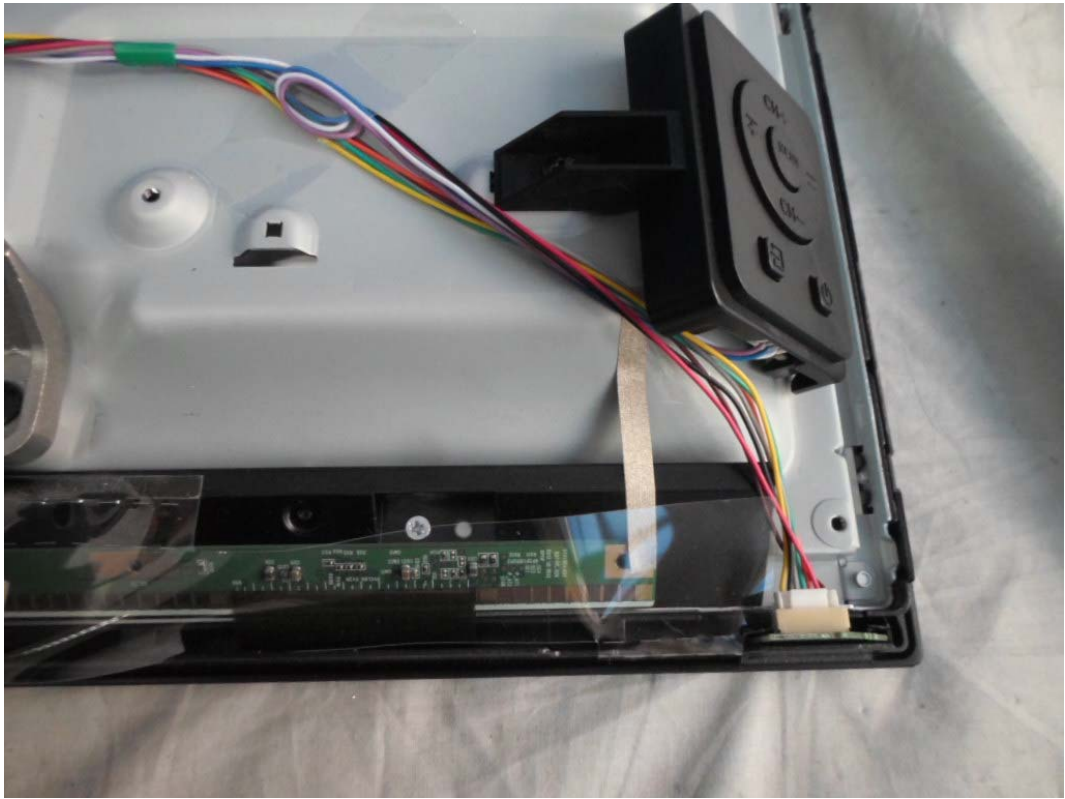
FIGURE 27 LED LCD TV (M/N: LTDN50K2203WUS) DEBUG #1
