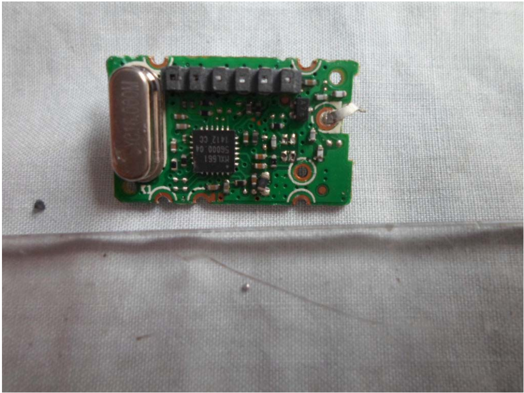
FIGURE 10 LED LCD TV (M/N: LTDN50K2203WUS) TUNER BOARD (COMPONENT SIDE)
