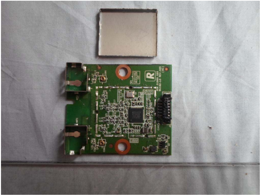
FIGURE 17 LED LCD TV (M/N: LTDN50K2203WUS) RF BOARD COVER REMOVED
