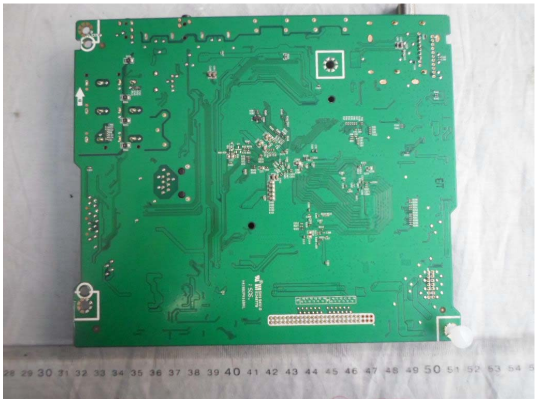
FIGURE 5 LED LCD TV (M/N: LTDN50K2203WUS) MAIN BOARD (SOLDERED SIDE)
