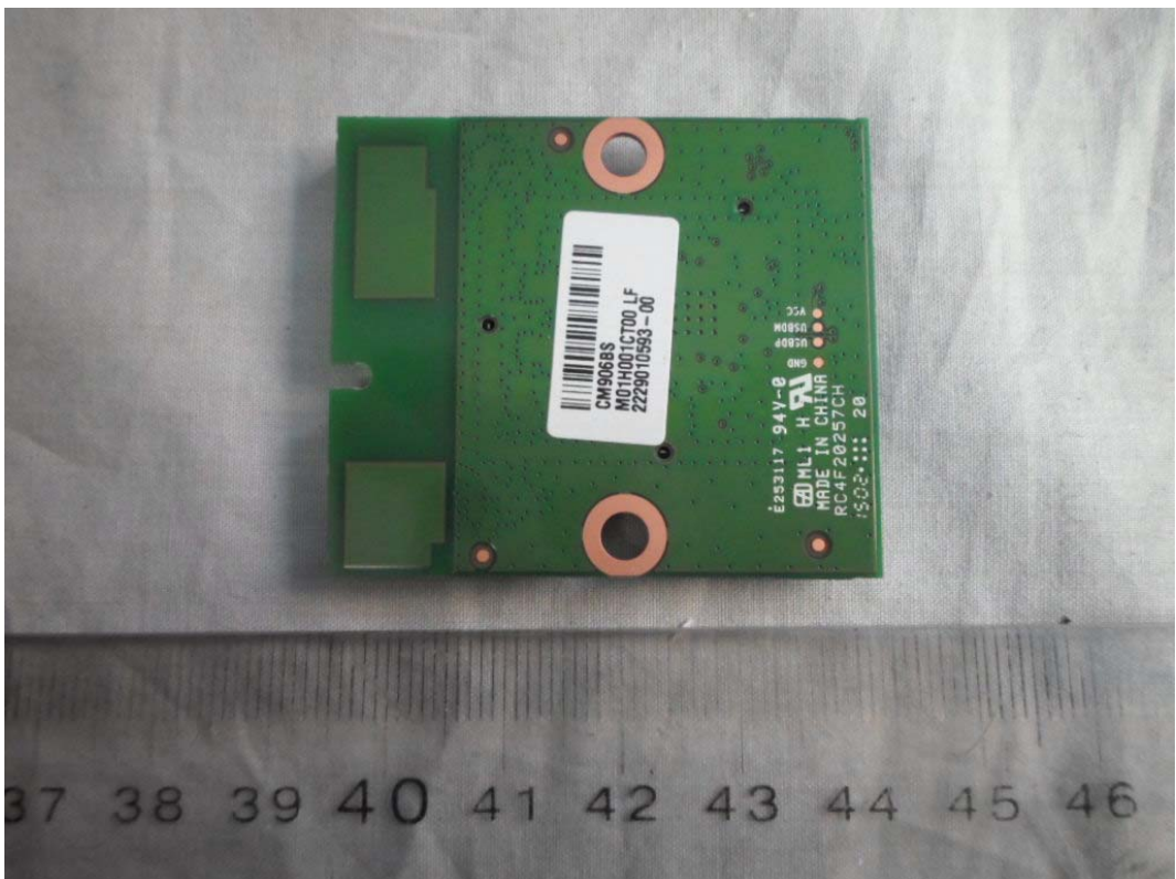
FIGURE 19 LED LCD TV (M/N: LTDN50K2203WUS) RF BOARD (SOLDERED SIDE)
