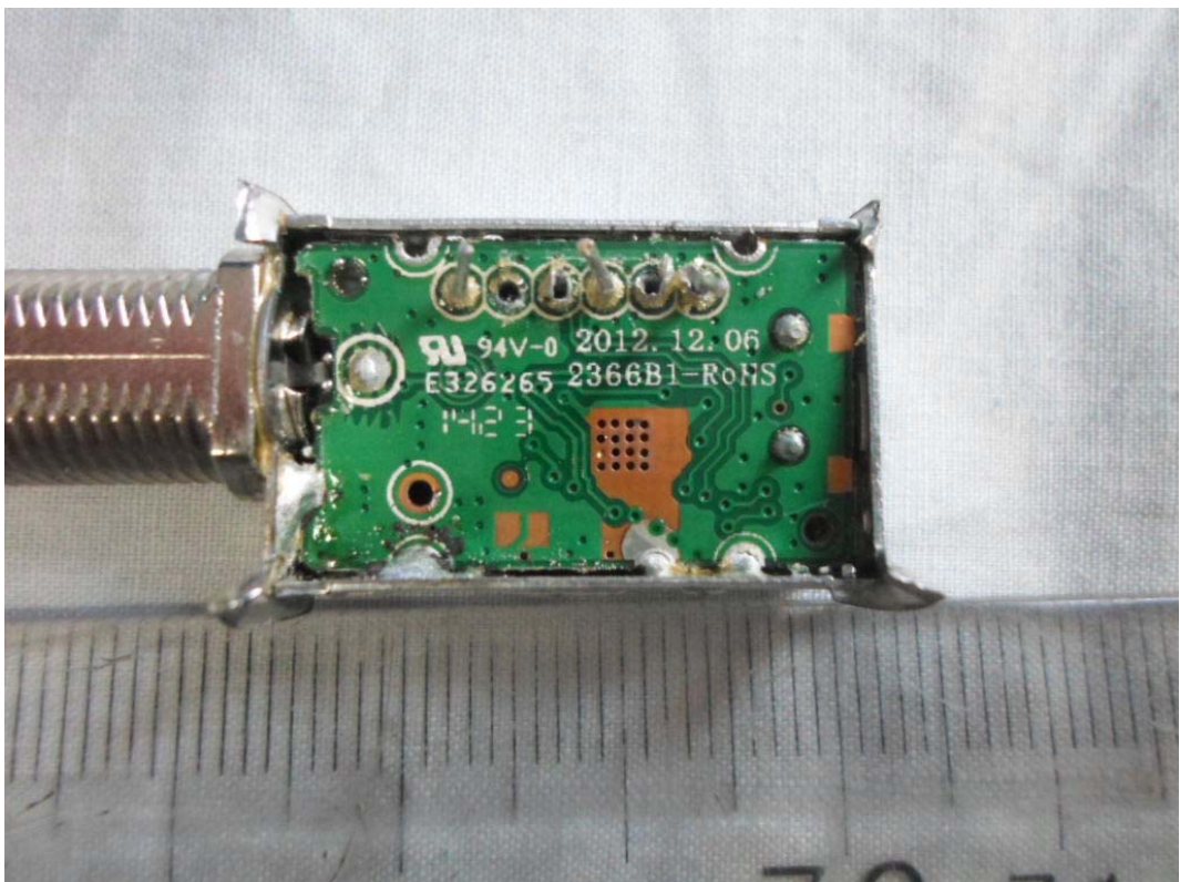
FIGURE 11 LED LCD TV (M/N: LTDN50K2203WUS) TUNER BOARD (SOLDERED SIDE)
