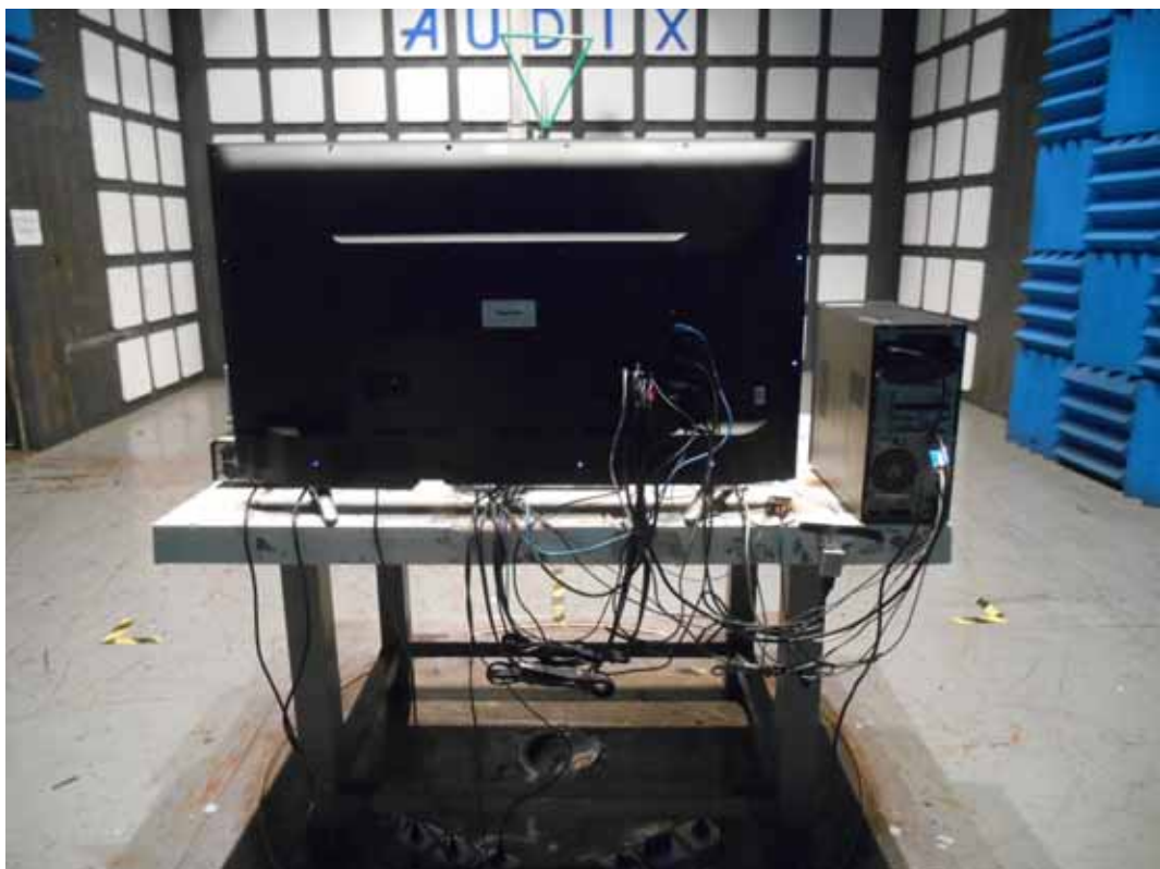
BACK VIEW OF RADIATED EMISSION TEST (BEIOW 1GHZ)
