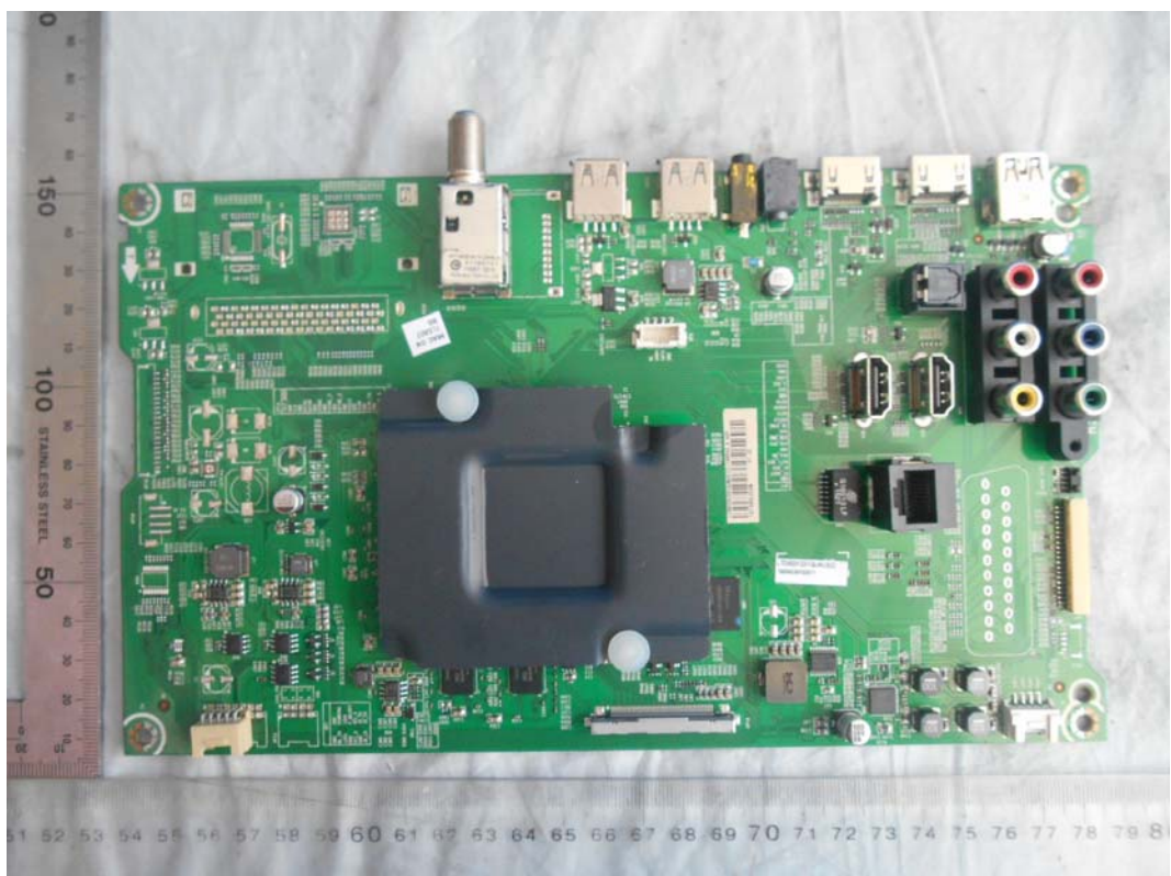
FIGURE 5 LED LCD TV (M/N: 50H7GB) MAIN BOARD (COMPONENT SIDE)
