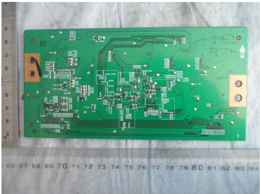
FIGURE 11 LED LCD TV (M/N: 50H7GB) SIGNAL BOARD (SOLDERED SIDE)
