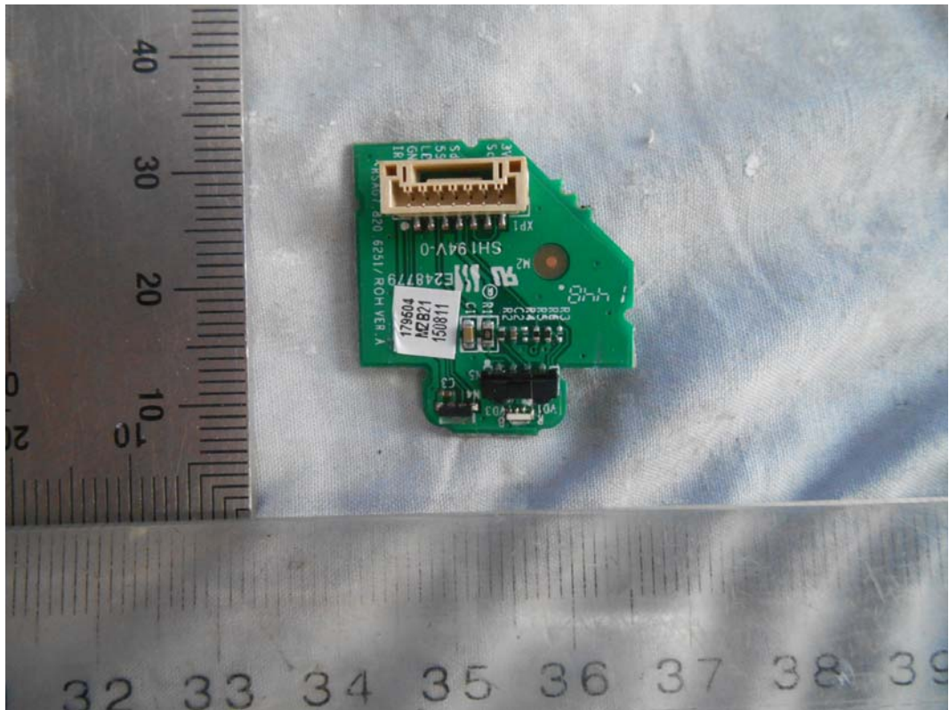
FIGURE 19 LED LCD TV (M/N: 50H7GB) IR BOARD (COMPONENT SIDE)
