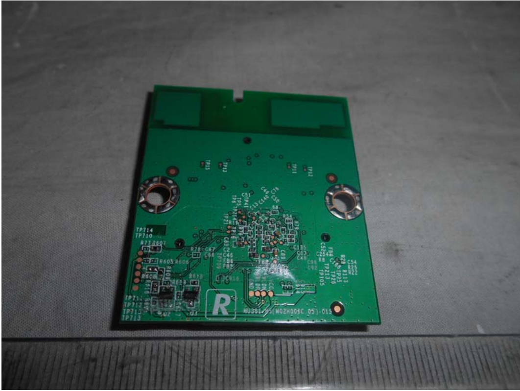
FIGURE 14 LED LCD TV (M/N: 50H7GB) RF BOARD (SOLDERED SIDE)
