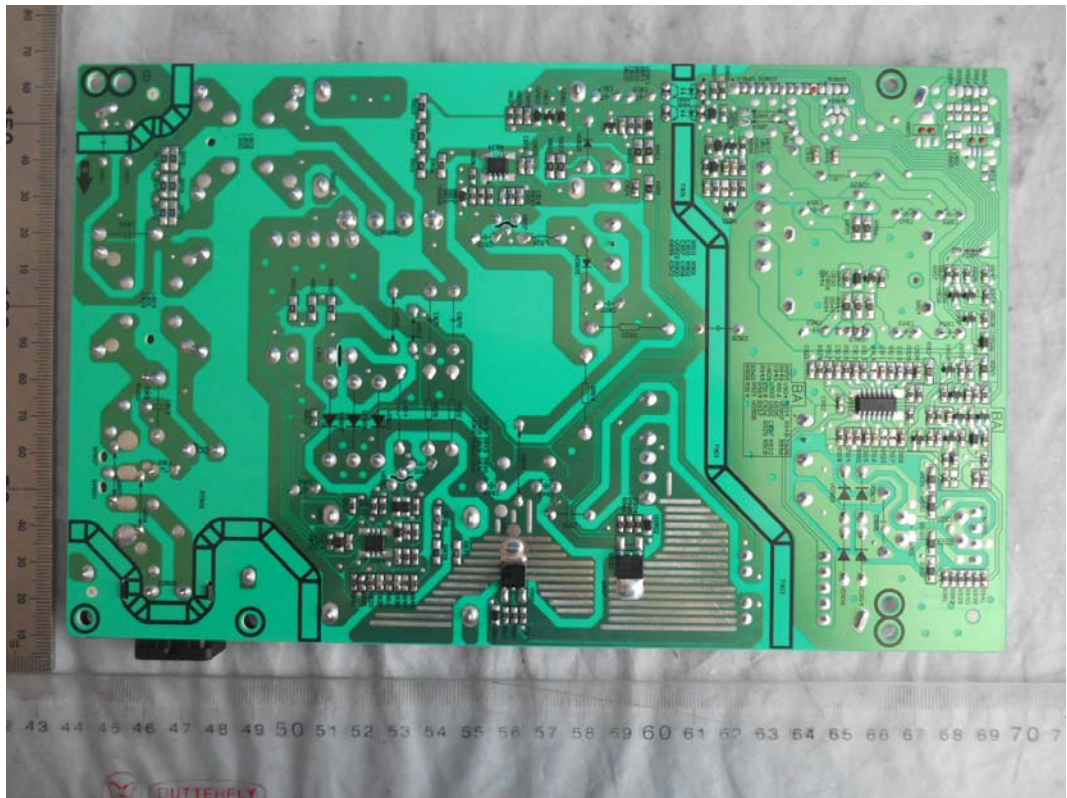
FIGURE 4 LED LCD TV (M/N: 50H7GB) POWER BOARD (SOLDERED SIDE)
