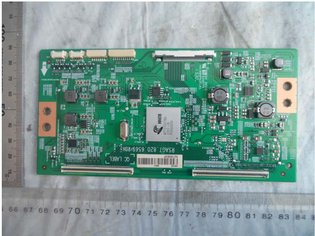
FIGURE 10 LED LCD TV (M/N: 50H7GB) SIGNAL BOARD (COMPONENT SIDE)
