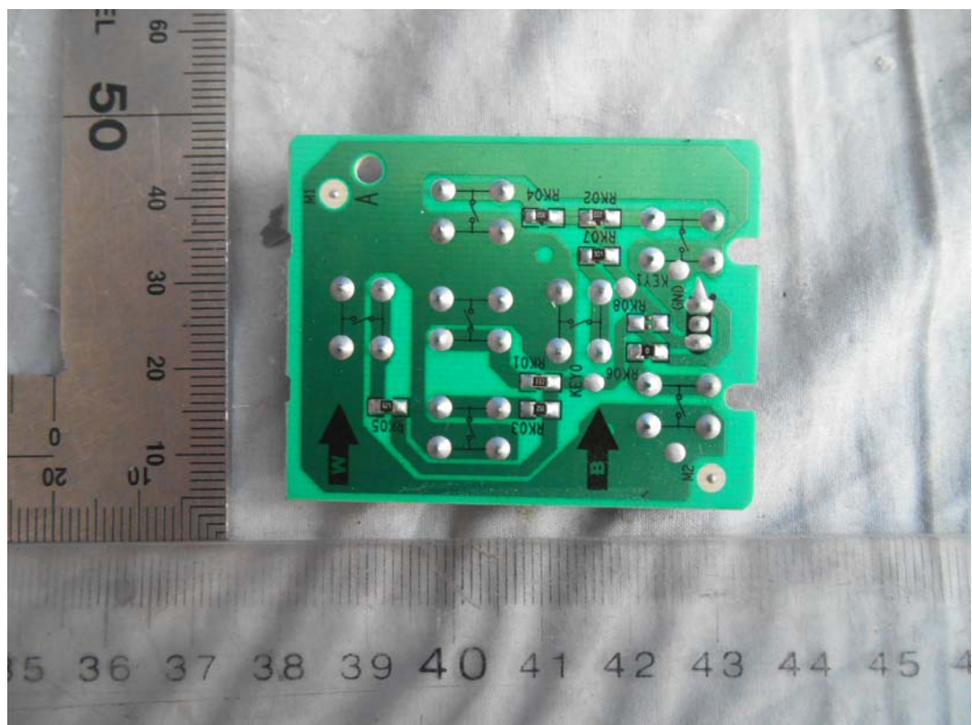
FIGURE 18 LED LCD TV (M/N: 50H7GB) KEY BOARD (SOLDERED SIDE)
