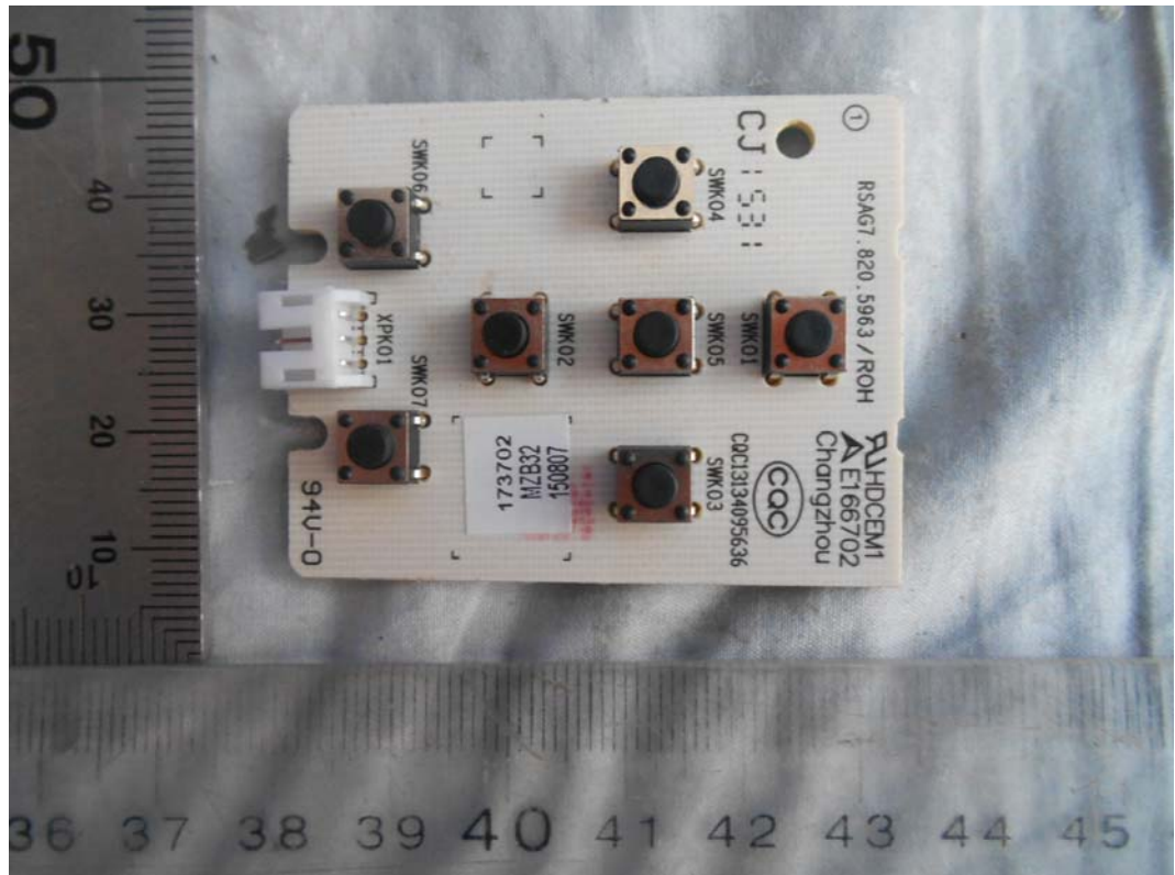
FIGURE 17 LED LCD TV (M/N: 50H7GB) KEY BOARD (COMPONENT SIDE)
