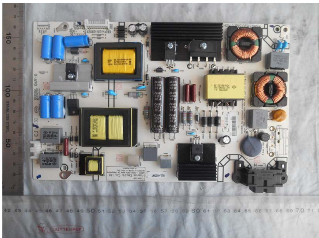
FIGURE 3 LED LCD TV (M/N: 50H7GB) POWER BOARD (COMPONENT SIDE)
