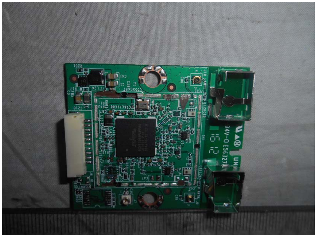
FIGURE 16 LED LCD TV (M/N: 50H7GB) CHIP AND CRYSTAL ON RF BOARD
