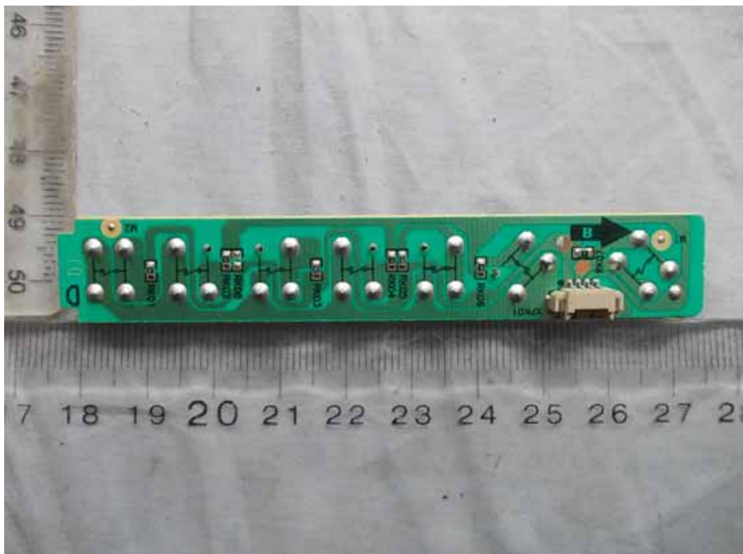
FIGURE 12 LED LCD TV (M/N: 50K20DG) KEY BOARD (SOLDERED SIDE)
