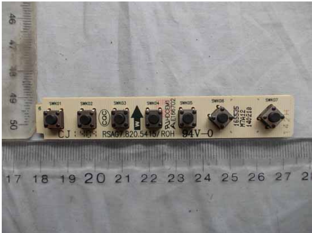
FIGURE 11 LED LCD TV (M/N: 50K20DG) KEY BOARD (COMPONENT SIDE)
