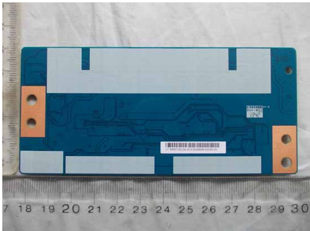
FIGURE 10 LED LCD TV (M/N: 50K20DG) LCD PANEL CONTROL BOARD (SOLDERED SIDE)
