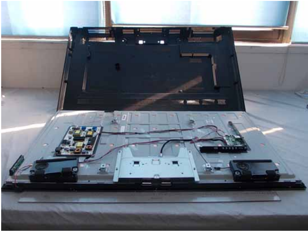
FIGURE 1 LED LCD TV (M/N: 50K20D) COVER REMOVED
