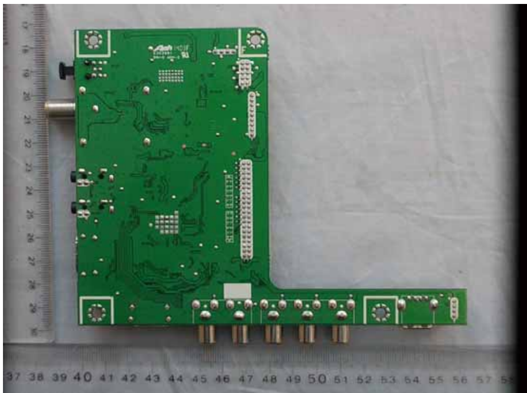
FIGURE 6 LED LCD TV (M/N: 50K20D) MAIN BOARD (SOLDERED SIDE)
