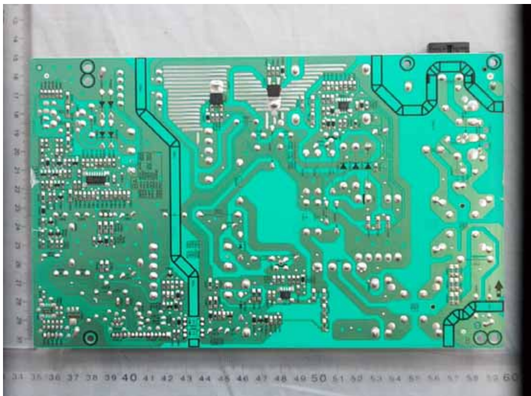
FIGURE 4 LED LCD TV (M/N: 50K20D) POWER BOARD (SOLDERED SIDE)
