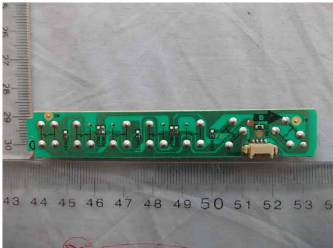
FIGURE 10 LED LCD TV (M/N: 50K20D) KEY BOARD (SOLDERED SIDE)
