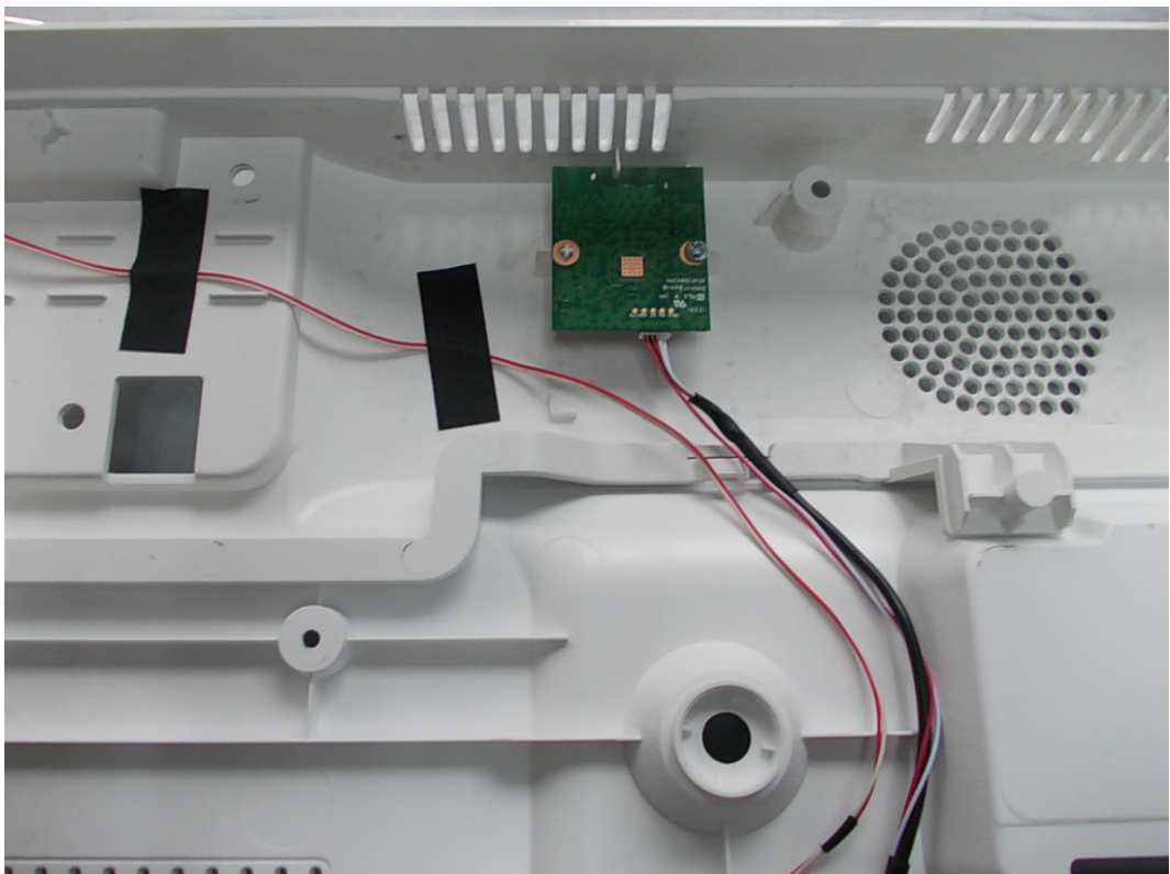
FIGURE 16 LED LCD TV (M/N: 55H8CG) LOCATION OF RF BOARD
