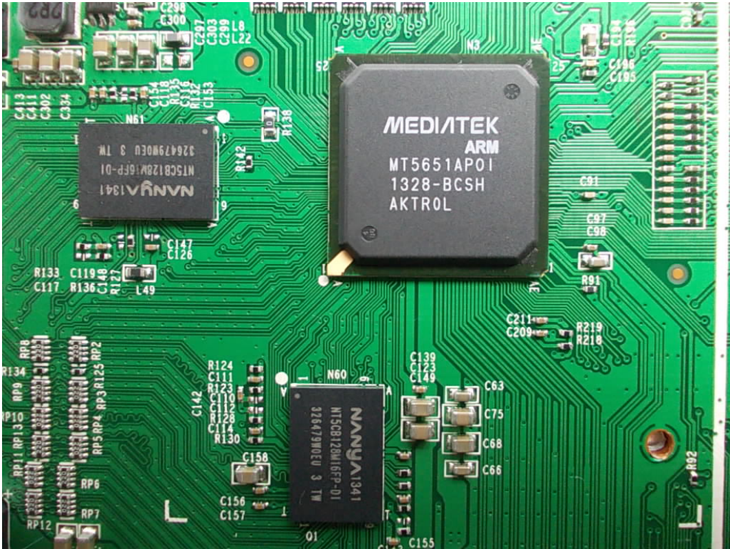
FIGURE 10 LED LCD TV (M/N: 55H8CG) CHIP #1 ON MAIN BOARD
