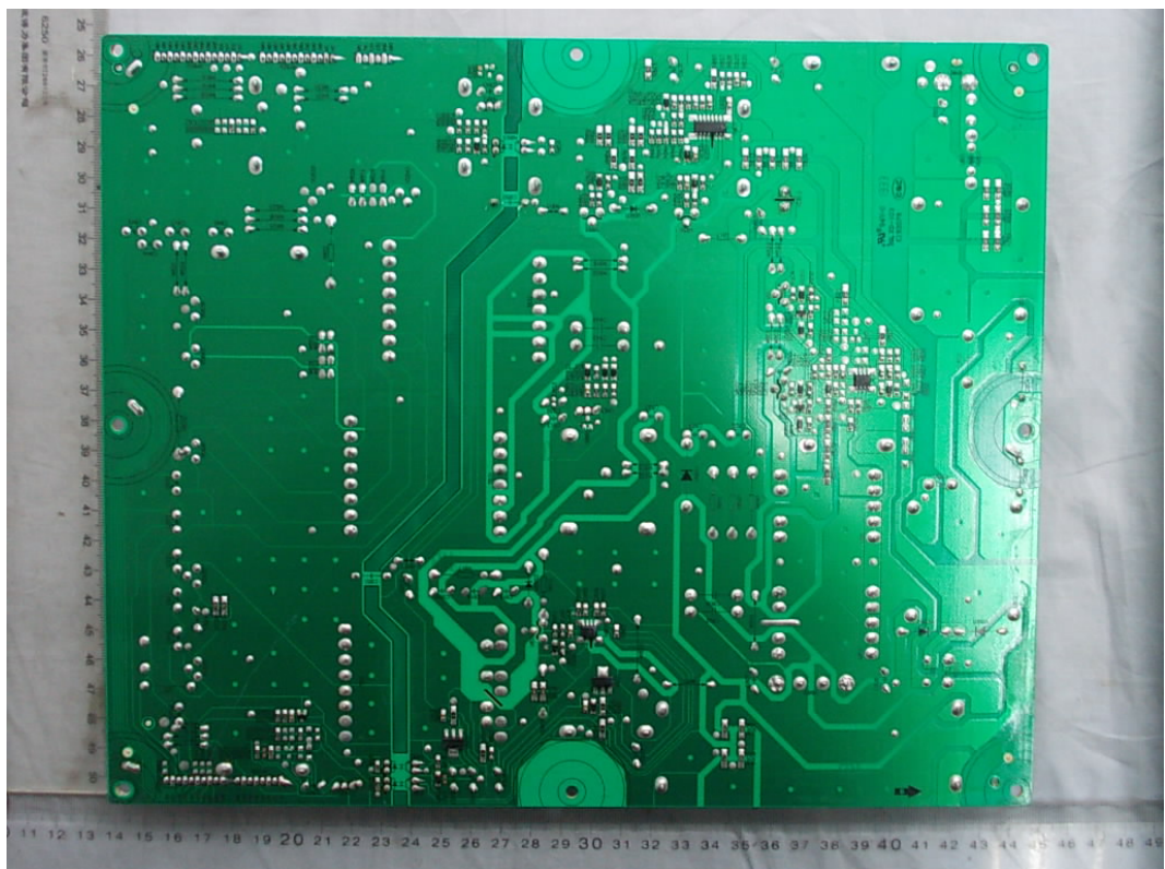
FIGURE 4 LED LCD TV (M/N: 55H8CG) POWER BOARD (SOLDERED SIDE)
