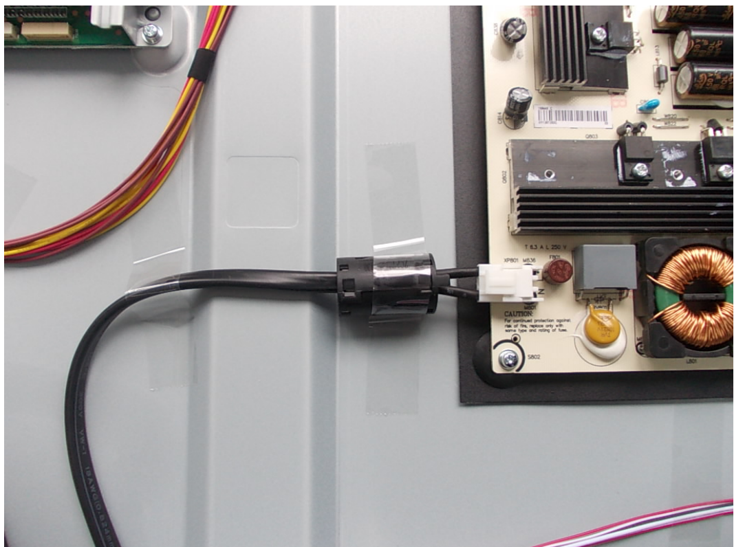
FIGURE 24 LED LCD TV (M/N: 55H8CG) DEBUG
