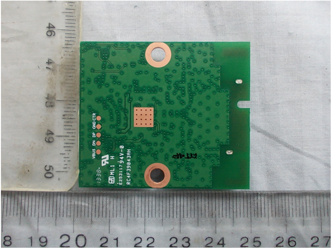
FIGURE 18 LED LCD TV (M/N: 55H8CG) RF BOARD (SOLDERED SIDE)
