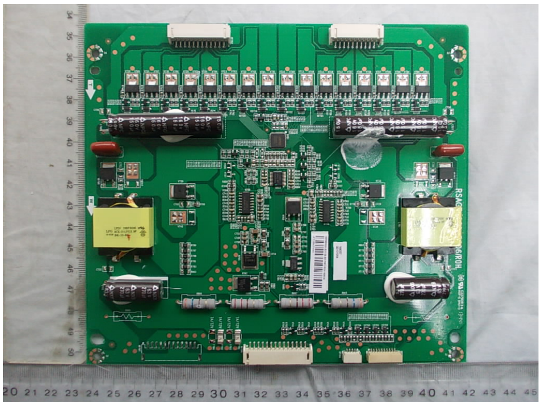
FIGURE 22 LED LCD TV (M/N: 55H8CG) BOARD (COMPONENT SIDE)
