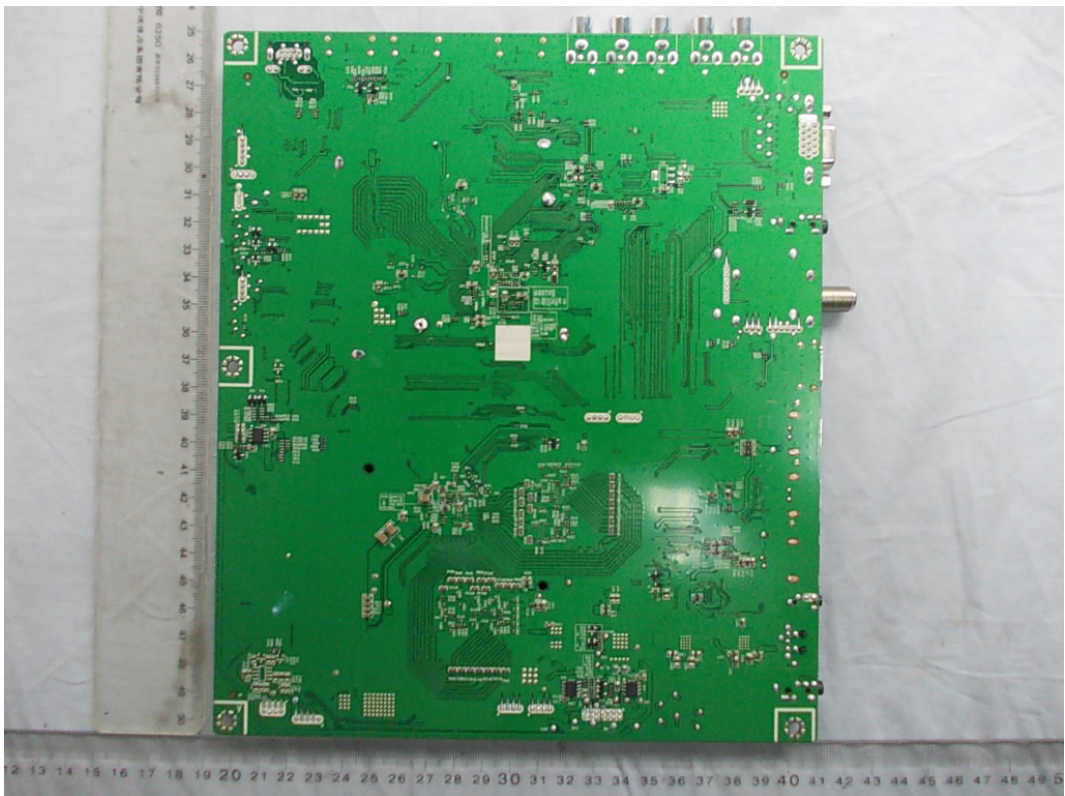
FIGURE 6 LED LCD TV (M/N: 55H8CG) MAIN BOARD (SOLDERED SIDE)
