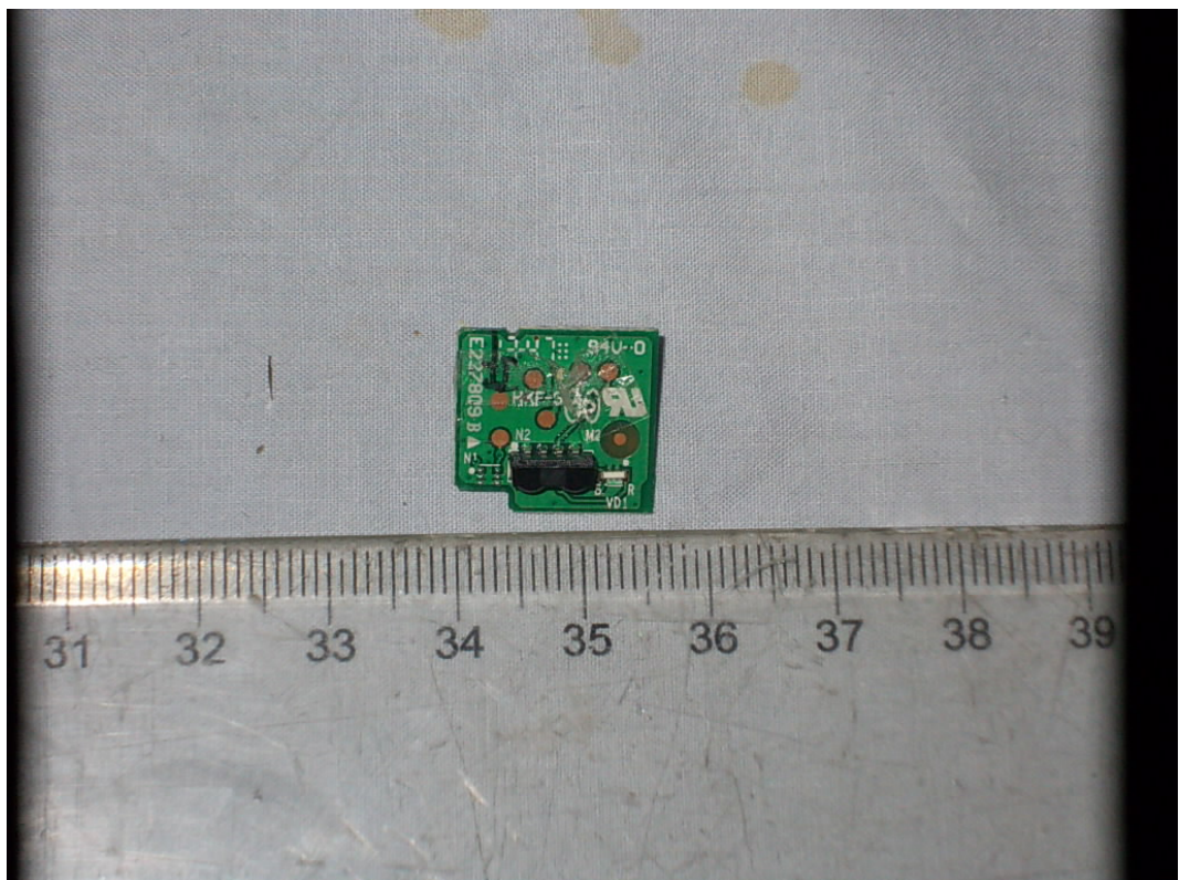
FIGURE 14 LED LCD TV (M/N: 55H8CG) IR BOARD (COMPONENT SIDE)
