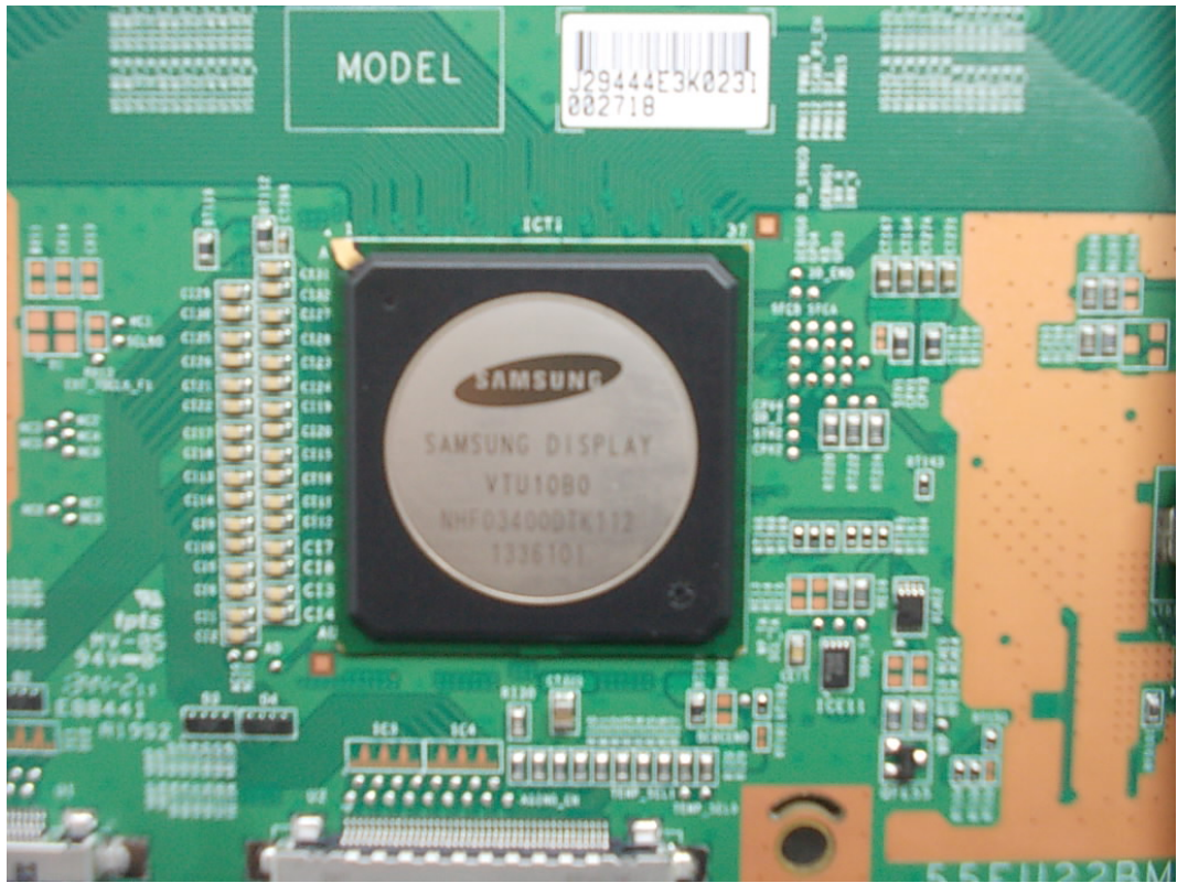
FIGURE 21 LED LCD TV (M/N: 55H8CG) CHIP ON LCD PANEL CONTROL BOARD
