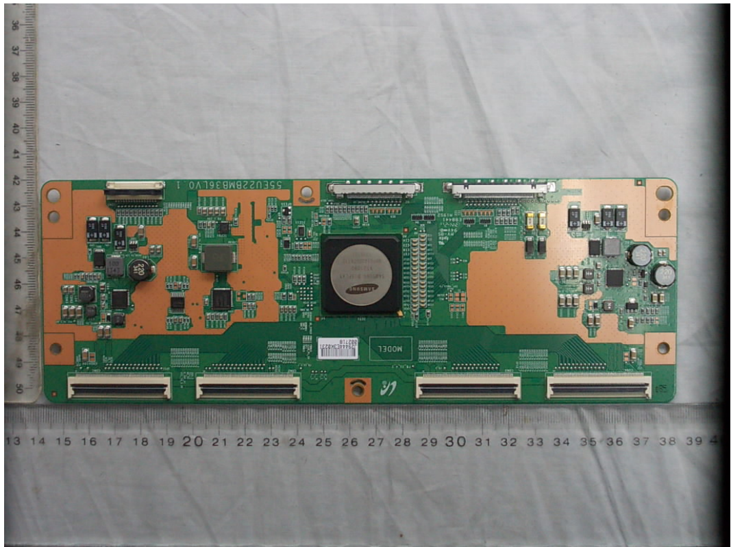
FIGURE 19 LED LCD TV (M/N: 55H8CG) LCD PANEL CONTROL BOARD (COMPONENT SIDE)
