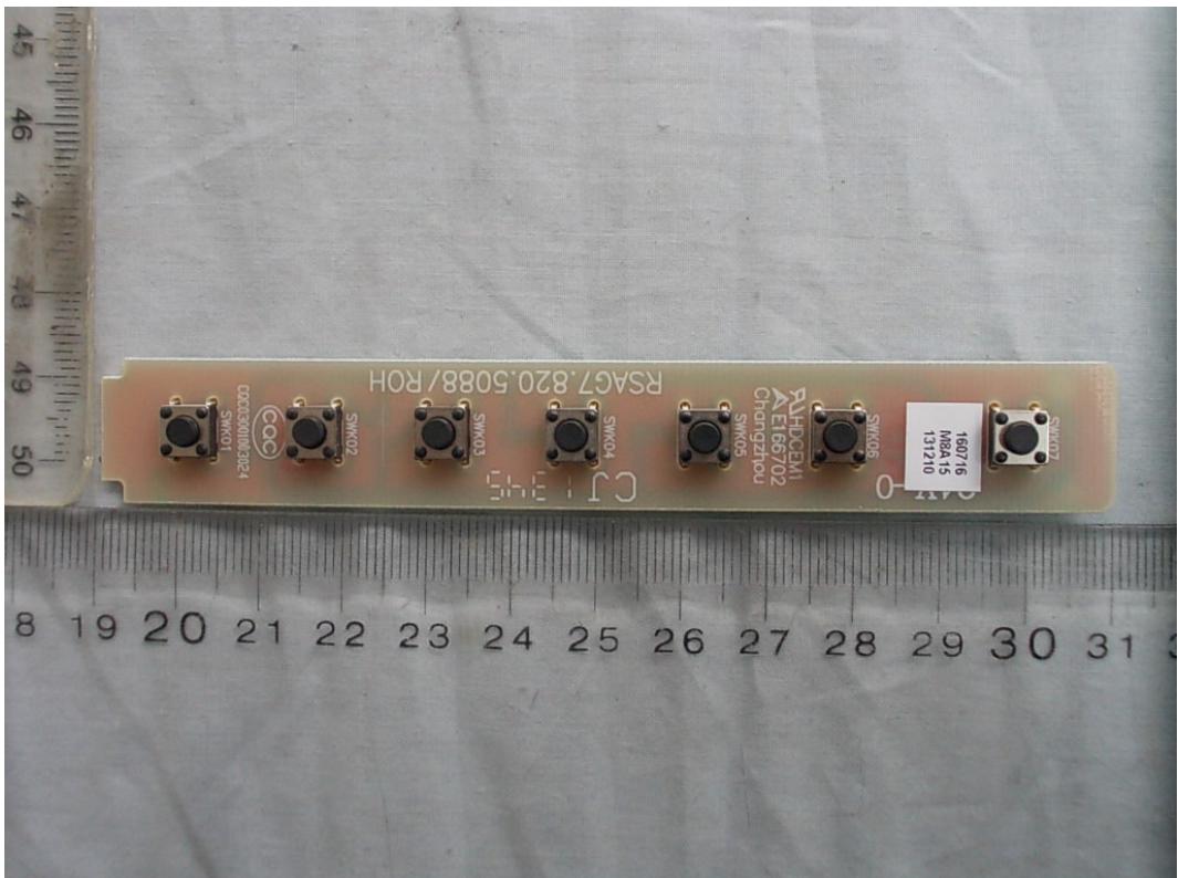
FIGURE 12 LED LCD TV (M/N: 55H8CG) KEY BOARD (COMPONENT SIDE)
