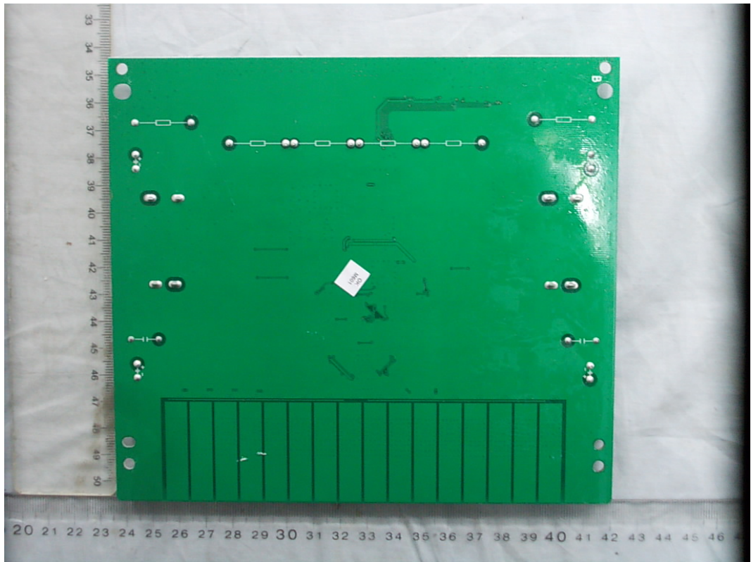
FIGURE 23 LED LCD TV (M/N: 55H8CG) BOARD (SOLDERED SIDE)
