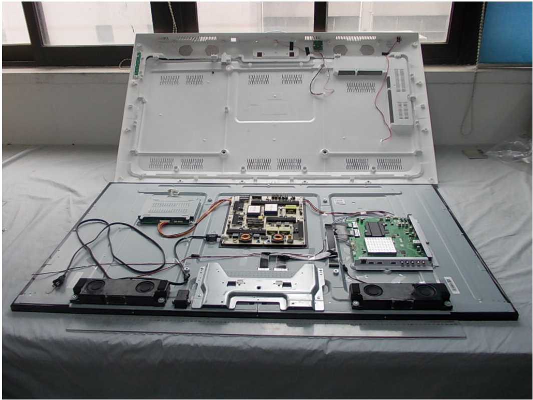
FIGURE 1 LED LCD TV (M/N: 55H8CG) COVER REMOVED
