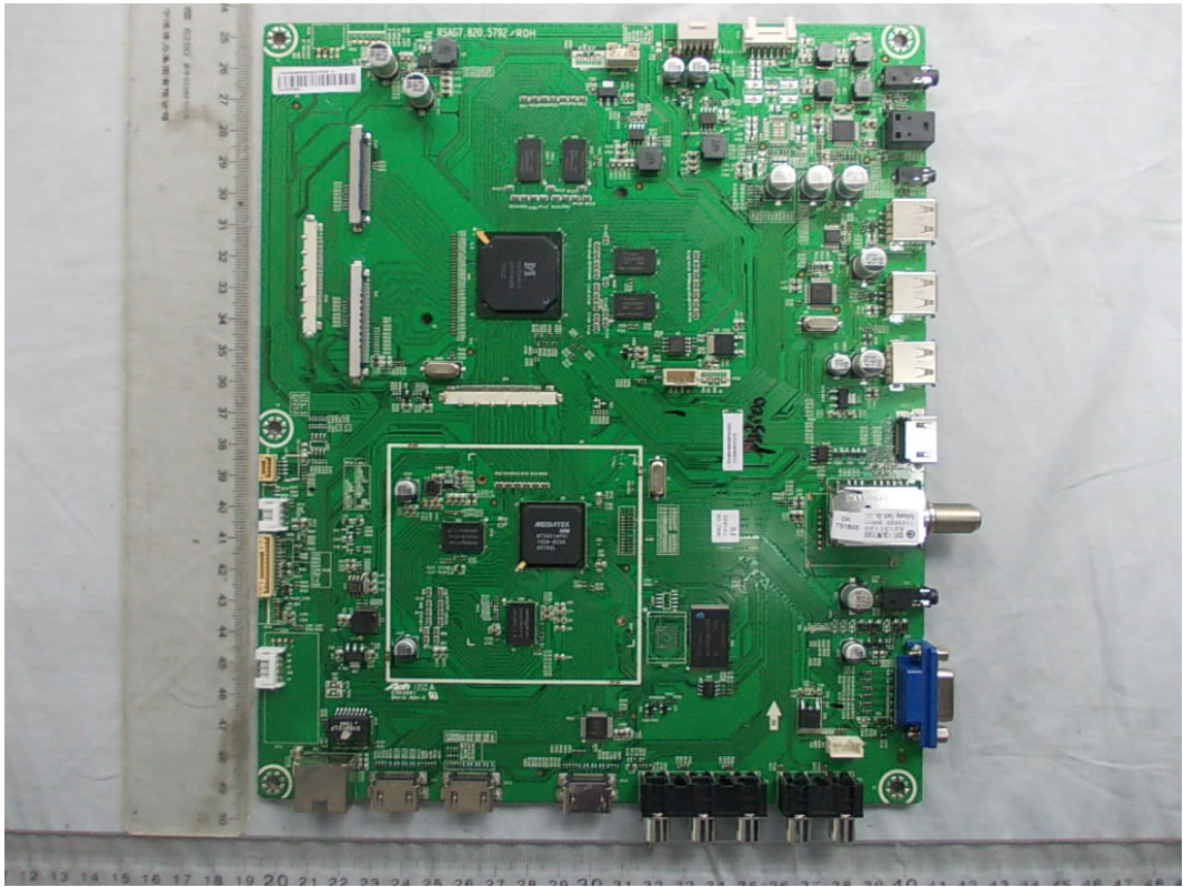
FIGURE 5 LED LCD TV (M/N: 55H8CG) MAIN BOARD (COMPONENT SIDE)
