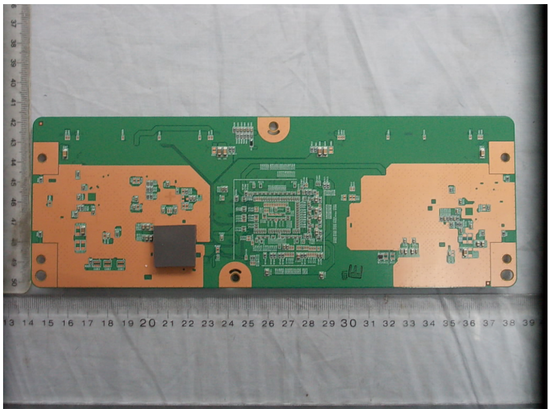
FIGURE 20 LED LCD TV (M/N: 55H8CG) LCD PANEL CONTROL BOARD (SOLDERED SIDE)
