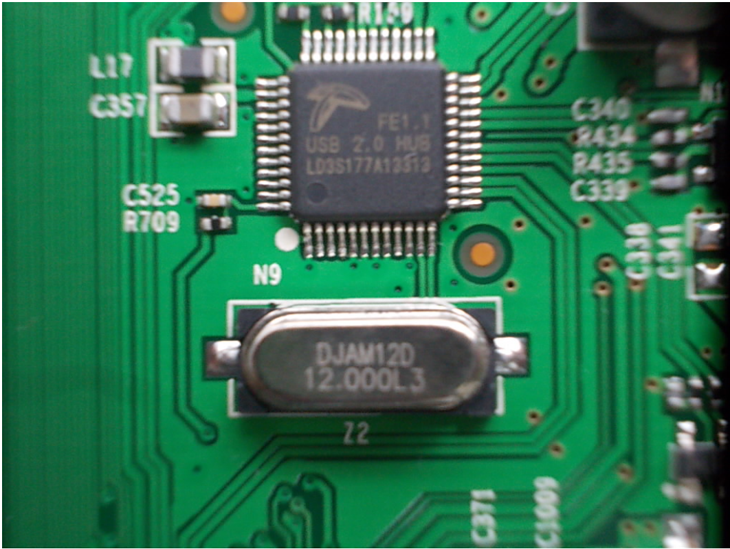
FIGURE 9 LED LCD TV (M/N: 55H8CG) CRYSTAL #3 ON MAIN BOARD
