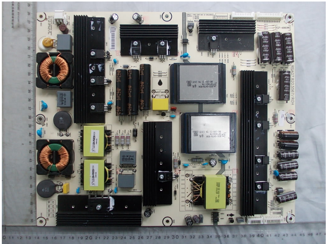
FIGURE 3 LED LCD TV (M/N: 55H8CG) POWER BOARD (COMPONENT SIDE)
