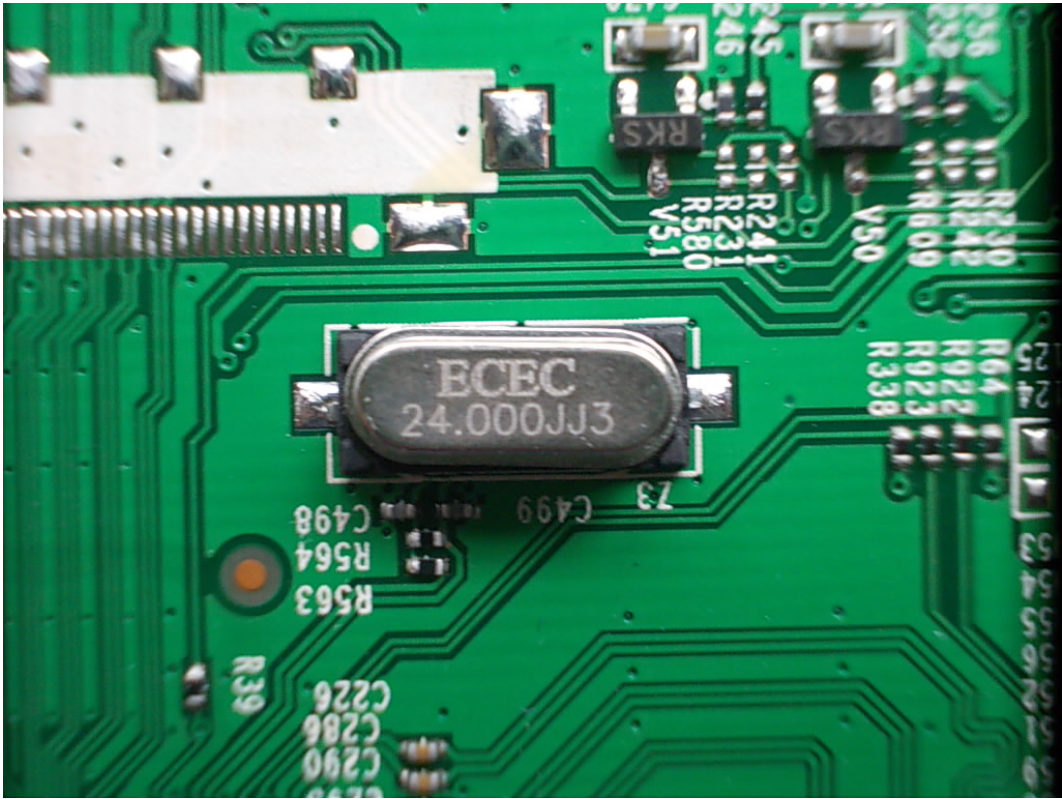
FIGURE 7 LED LCD TV (M/N: 55H8CG) CRYSTAL #1 ON MAIN BOARD
