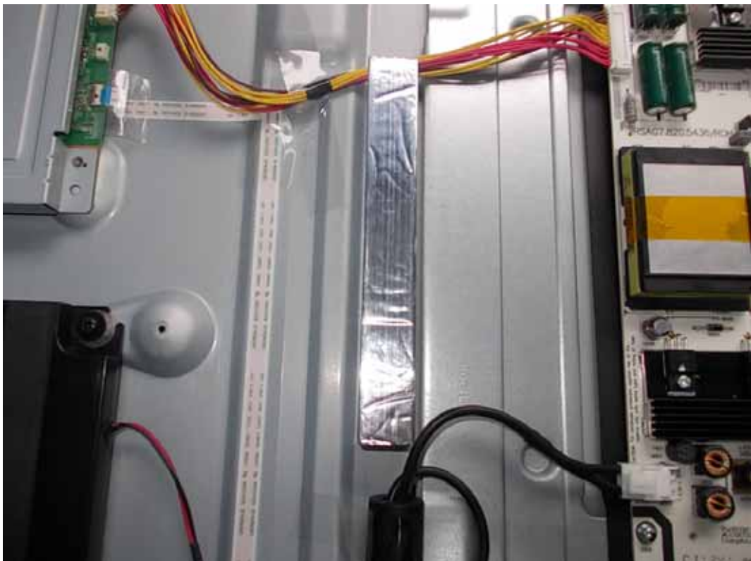
FIGURE 27 LED LCD TV (M/N: LTDN55XT880WUS) DEBUG #4
