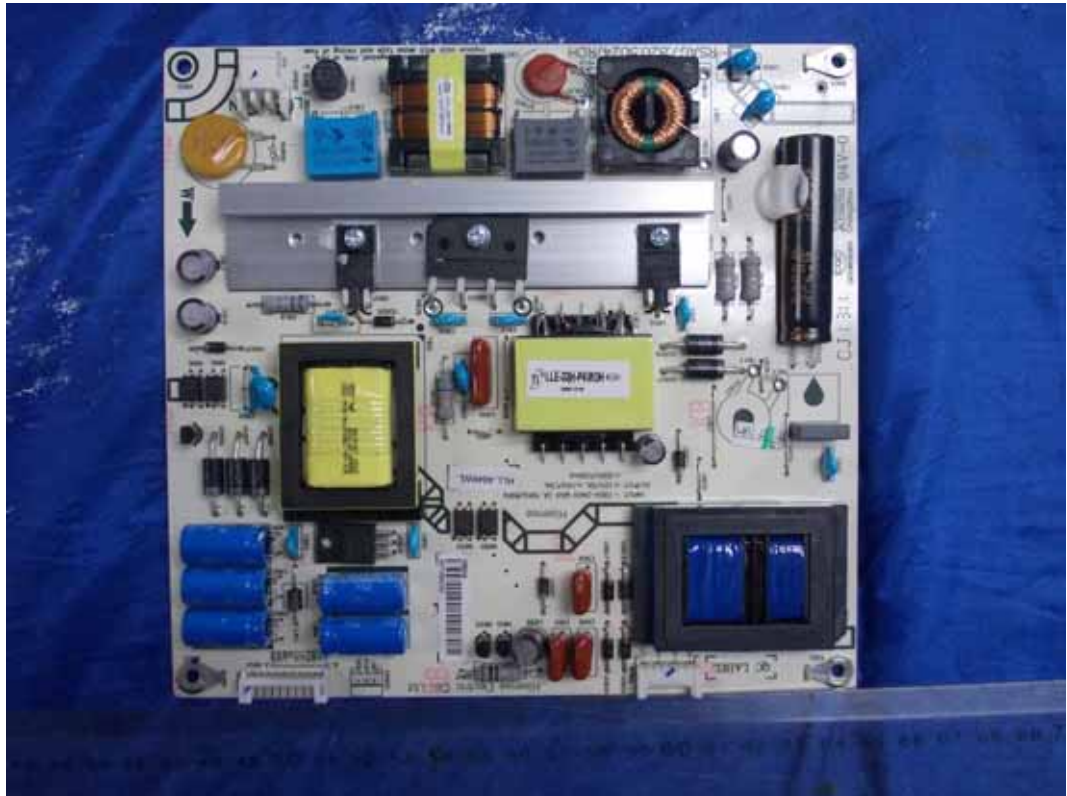
FIGURE 3 LED LCD TV (M/N: 50K362G) POWER BOARD (COMPONENT SIDE)
