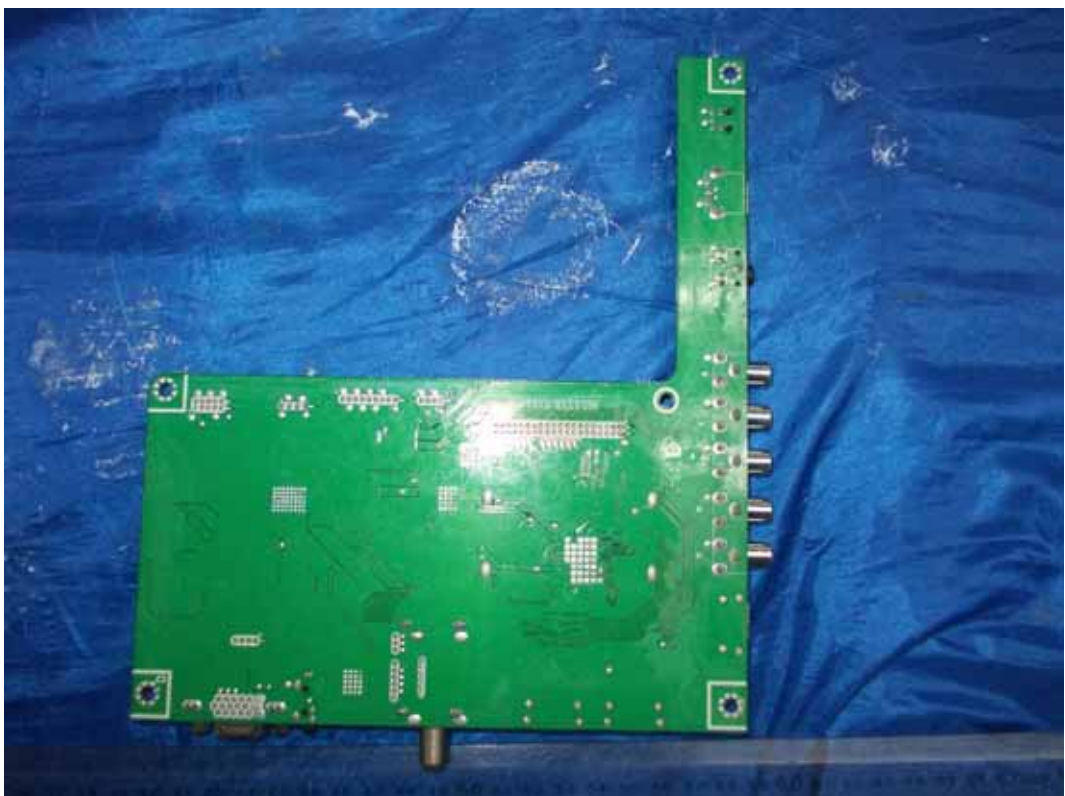
FIGURE 6 LED LCD TV (M/N: 50K362G) MAIN BOARD (SOLDERED SIDE)
