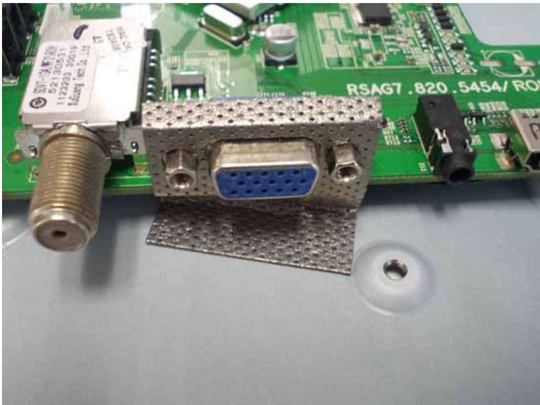
FIGURE 26 LED LCD TV (M/N: 50K366GW) DEBUG #1
