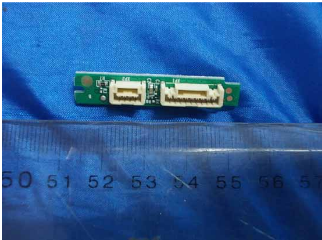
FIGURE 15 LED LCD TV (M/N: 55K610GWN) IR BOARD (SOLDERED SIDE)
