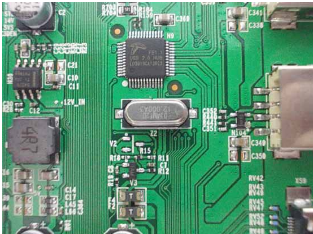
FIGURE 10 LED LCD TV (M/N: 50K610GWN) CHIP #1 & CRYSTAL #2 ON MAIN BOARD
