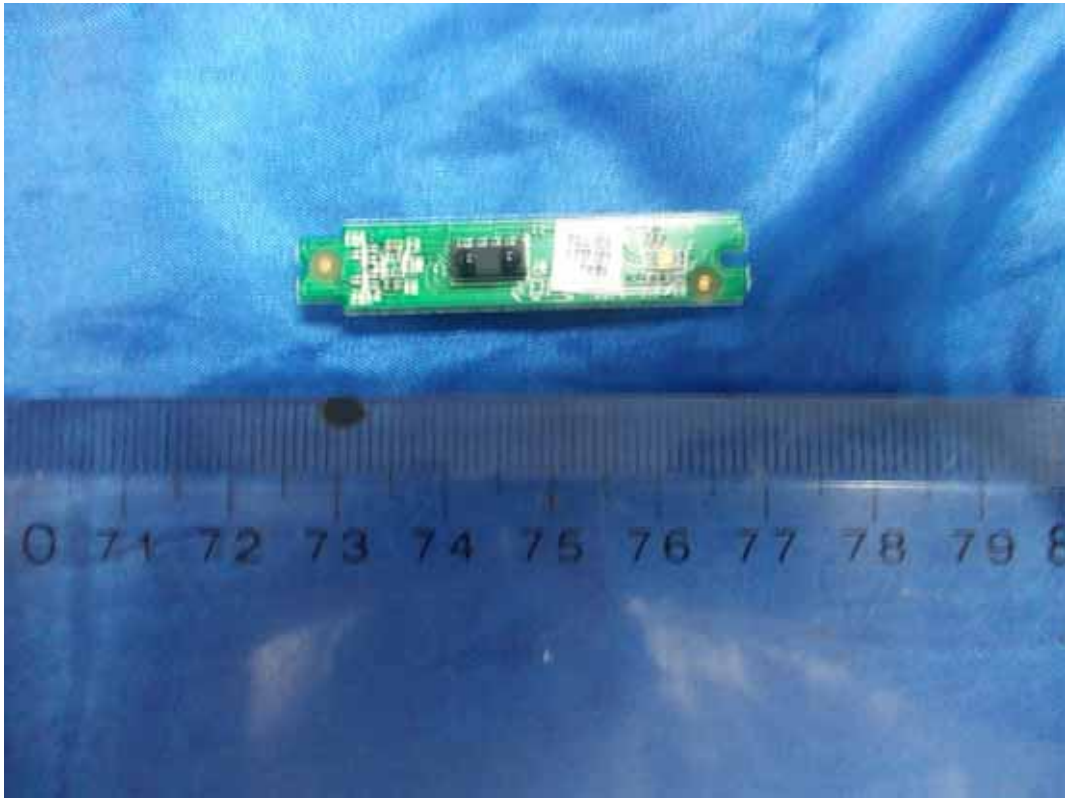
FIGURE 14 LED LCD TV (M/N: 50K610GWN) IR BOARD (COMPONENT SIDE)
