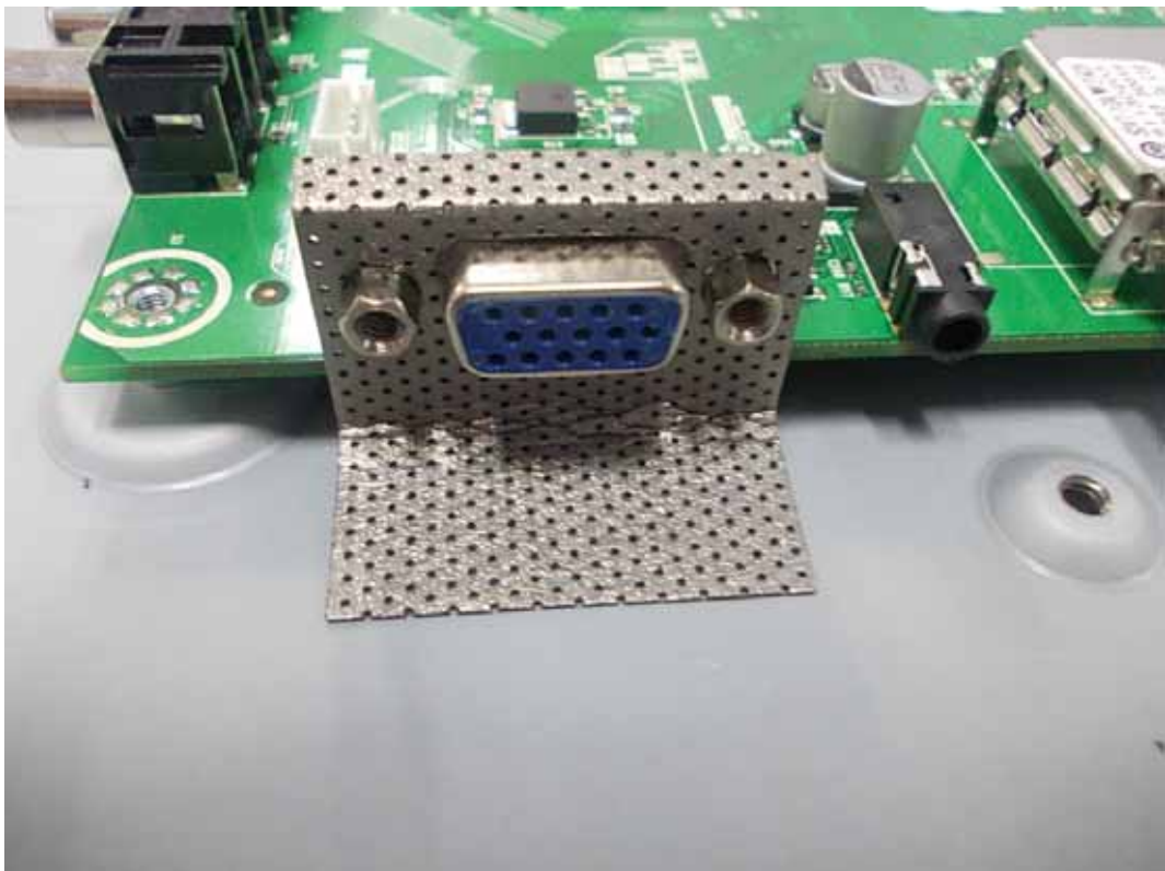
FIGURE 21 LED LCD TV (M/N: 50K610GWN) DEBUG 2
