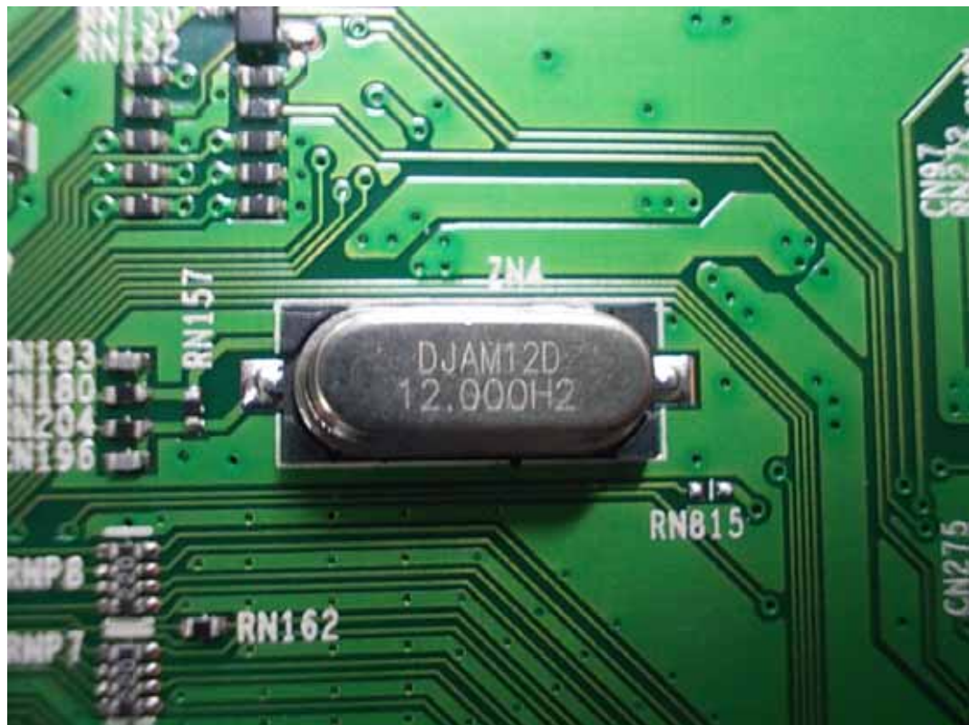
FIGURE 19 LED LCD TV (M/N: LTDN55K610GWUS) CRYSTAL ON LCD PANEL CONTROL BOARD
