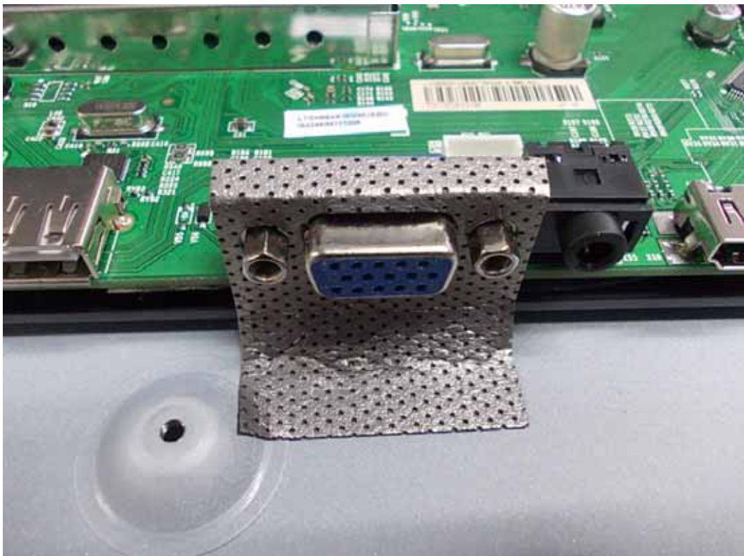
FIGURE 22 LED LCD TV (M/N: LTDN55K610GWUS) DEBUG 2
