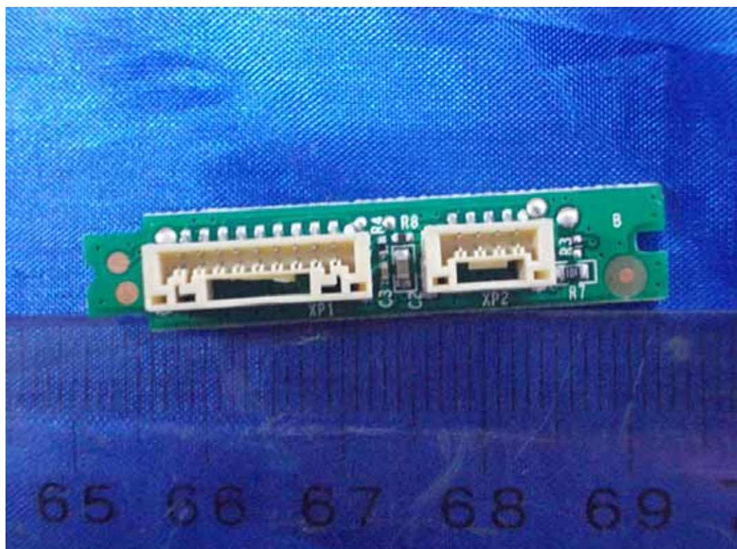
FIGURE 16 LED LCD TV (M/N: LTDN55K610GWUS) IR BOARD (SOLDERED SIDE)
