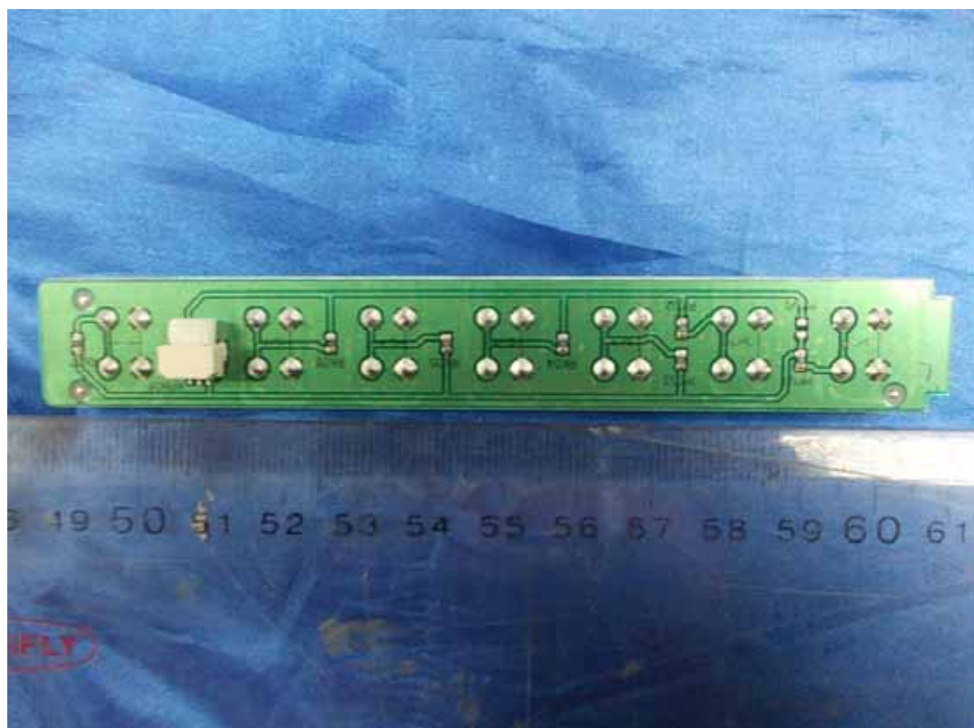
FIGURE 14 LED LCD TV (M/N: LTDN55K610GWUS) KEY BOARD (SOLDERED SIDE)
