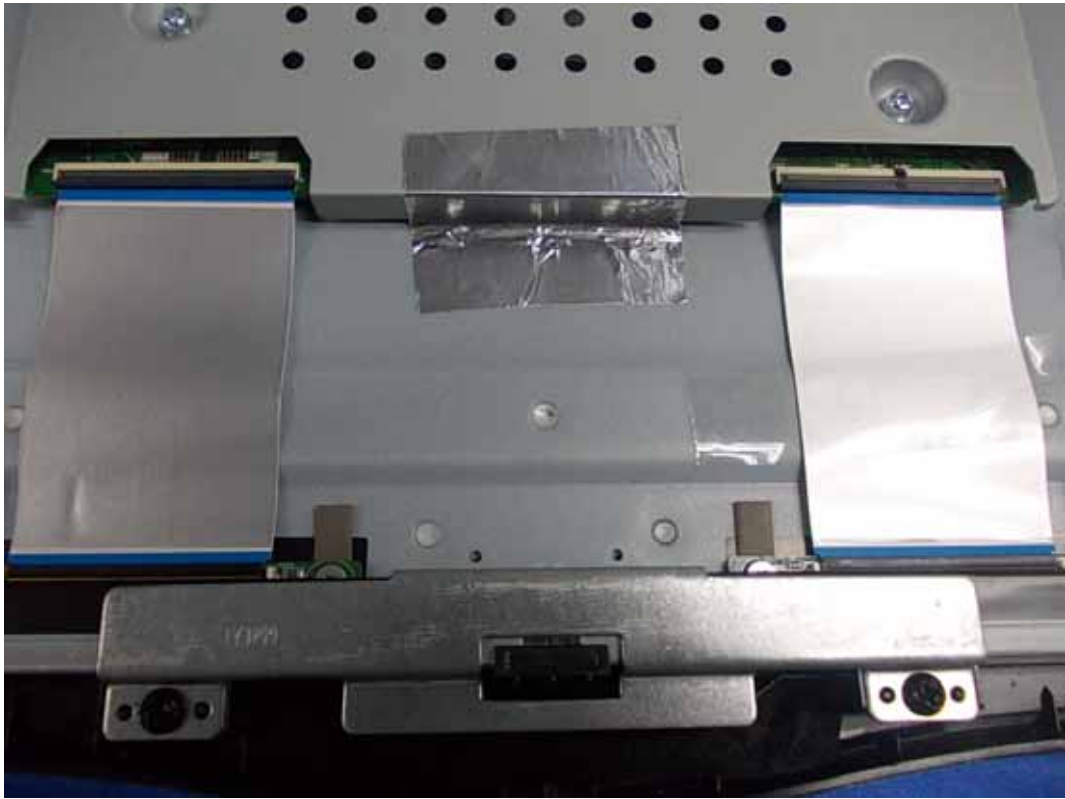
FIGURE 21 LED LCD TV (M/N: LTDN55K610GWUS) DEBUG 1
