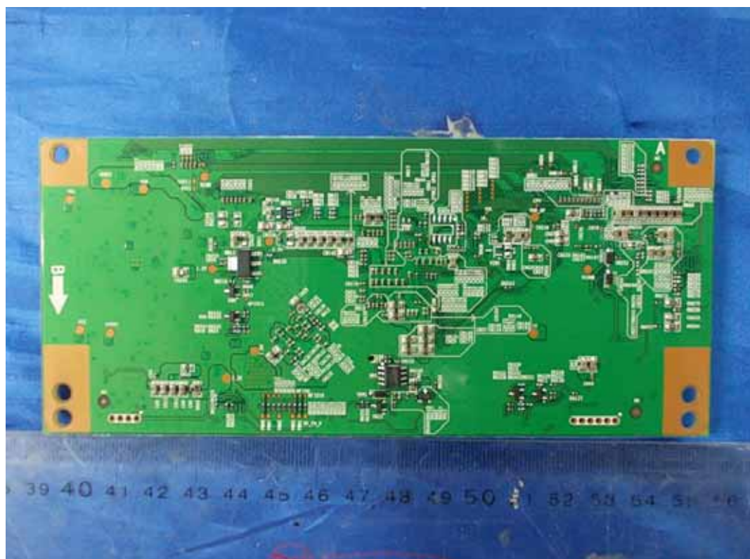
FIGURE 18 LED LCD TV (M/N: LTDN50K610GWUS) LCD PANEL CONTROL BOARD (SOLDERED SIDE)
