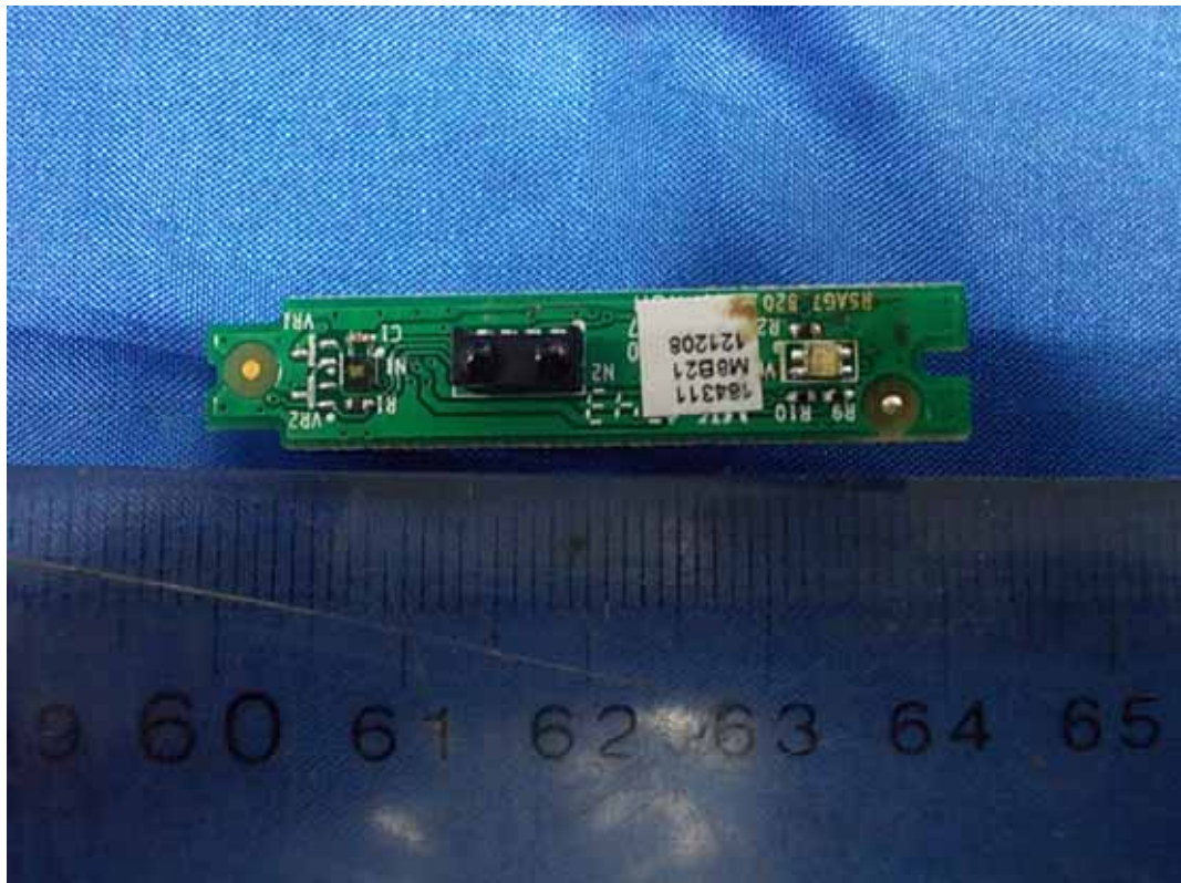
FIGURE 15 LED LCD TV (M/N: LTDN50K610GWUS) IR BOARD (COMPONENT SIDE)
