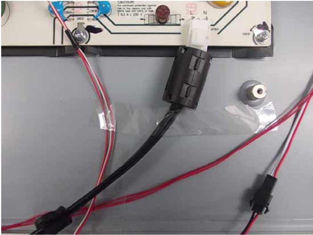
FIGURE 20 LED LCD TV (M/N: LTDN65K560XWUS3D) DEBUG #2
