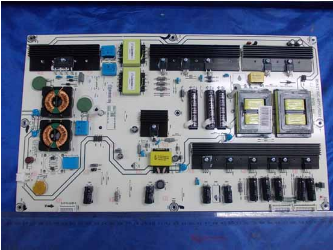
FIGURE 2 LED LCD TV (M/N: LTDN65K560XWUS3D) POWER BOARD (COMPONENT SIDE)
