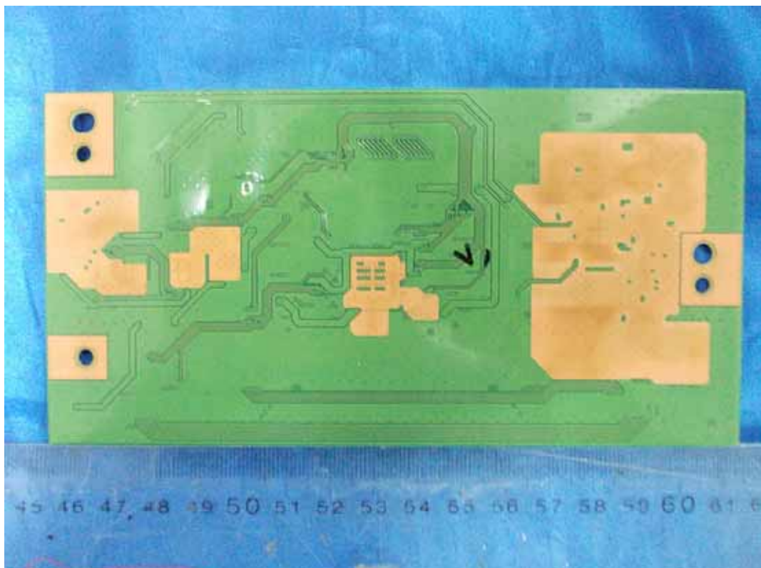
FIGURE 20 LED LCD TV (M/N: LTDN55XT710XWUS3D) LCD PANEL CONTROL BOARD (SOLDERED SIDE)
