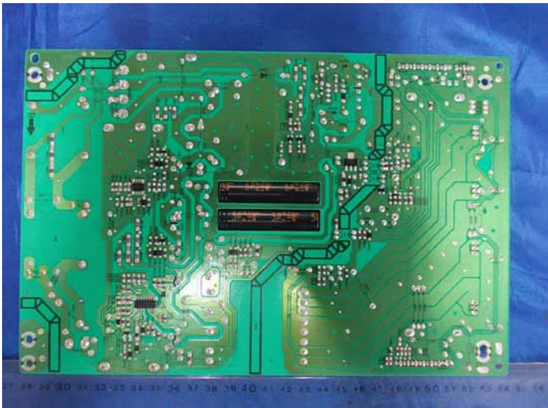
FIGURE 5 LED LCD TV (M/N: LTDN55XT710XWUS3D) POWER BOARD (SOLDERED SIDE)
