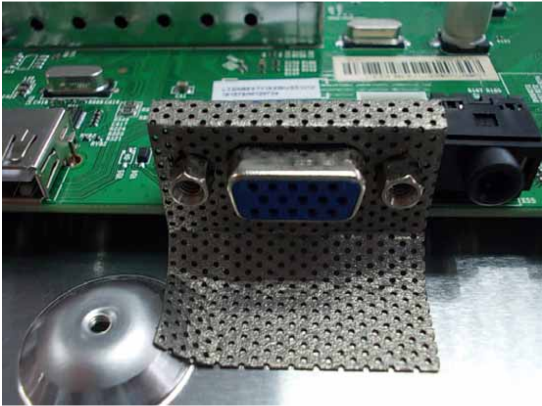
FIGURE 27 LED LCD TV (M/N: LTDN55XT710XWUS3D) DEBUG 5
