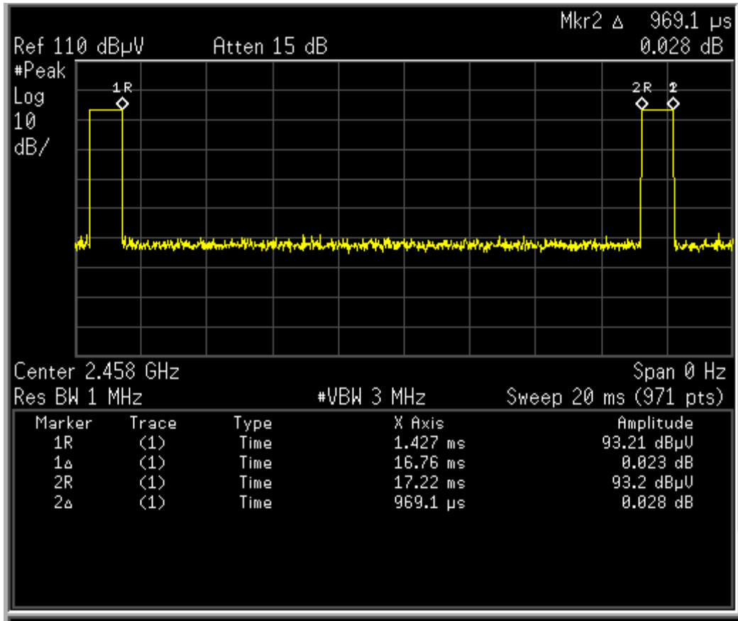
DUTY CYCLE
