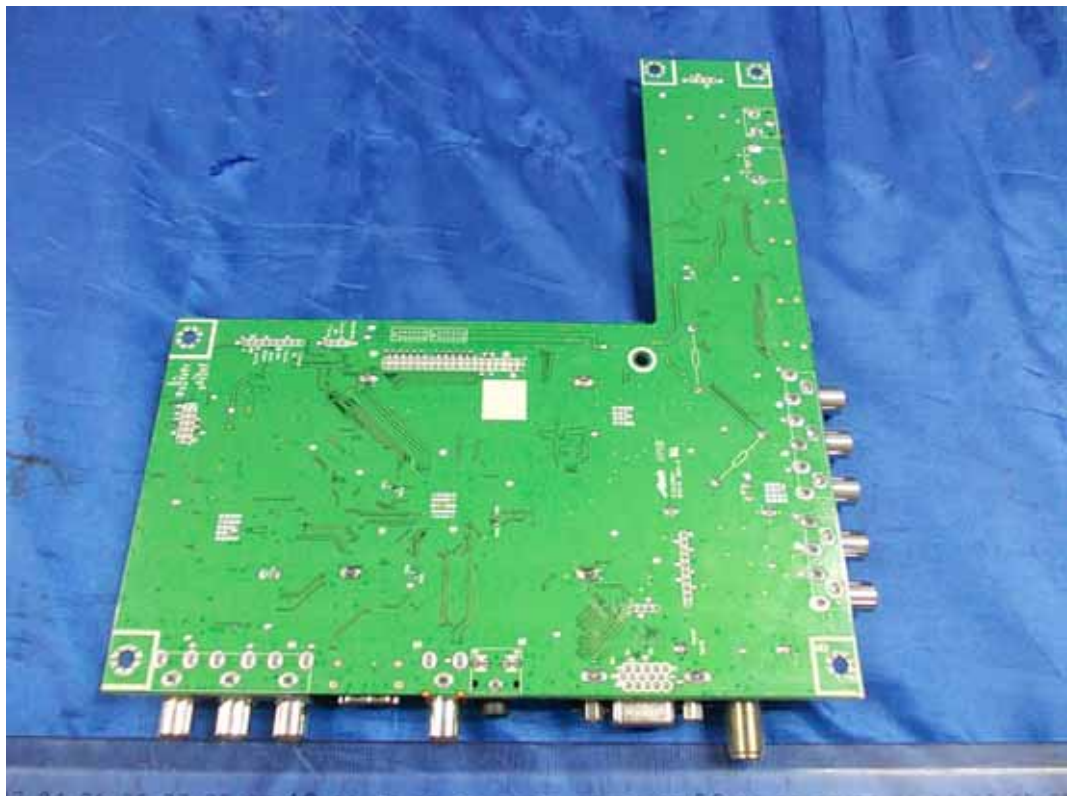
FIGURE 5 LED LCD TV (M/N: LTDN50K360GUS) MAIN BOARD (SOLDERED SIDE)
