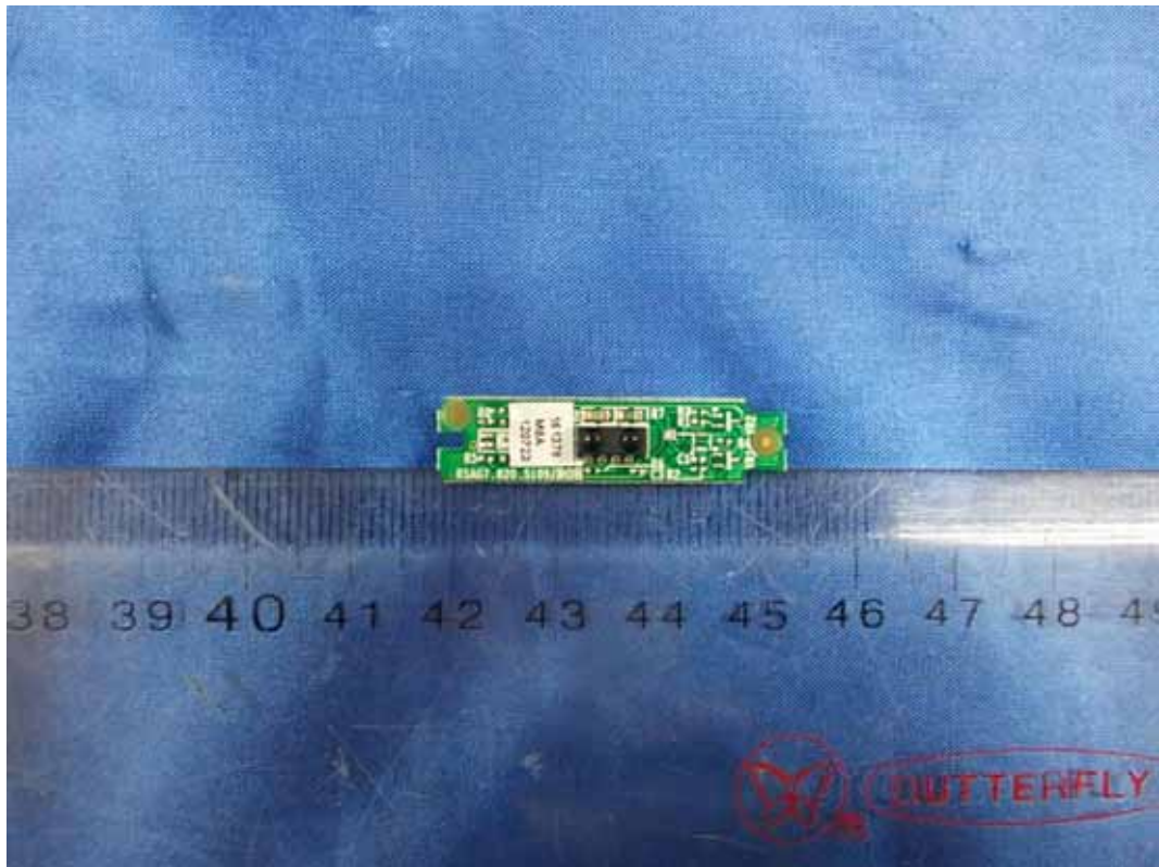
FIGURE 10 LED LCD TV (M/N: LTDN50K360GUS) IR BOARD (COMPONENT SIDE)
