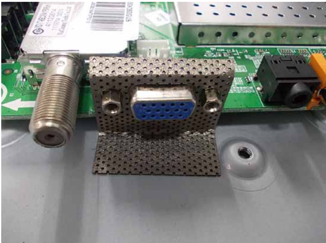
FIGURE 17 LED LCD TV (M/N: LTDN50K360GUS) DEBUG #2
