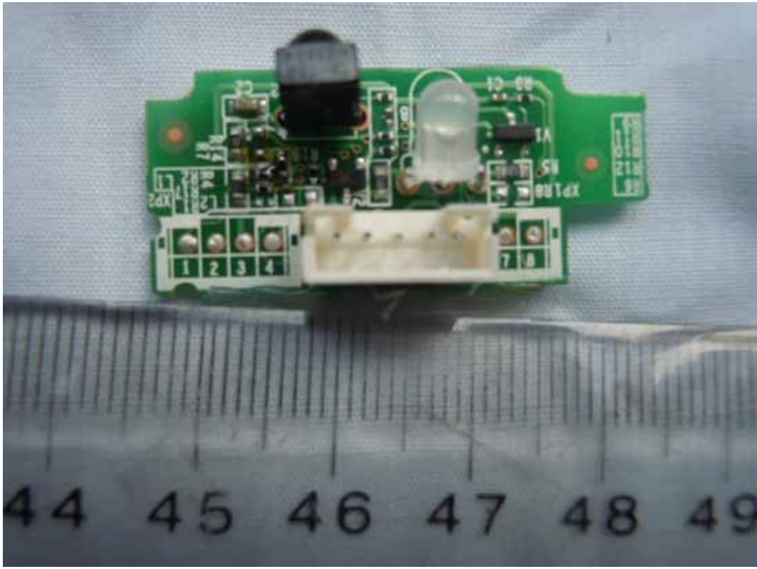
FIGURE 13 LED LCD TV (M/N: LTDN55T39XWUS3D) IR BOARD (COMPONENT SIDE)
