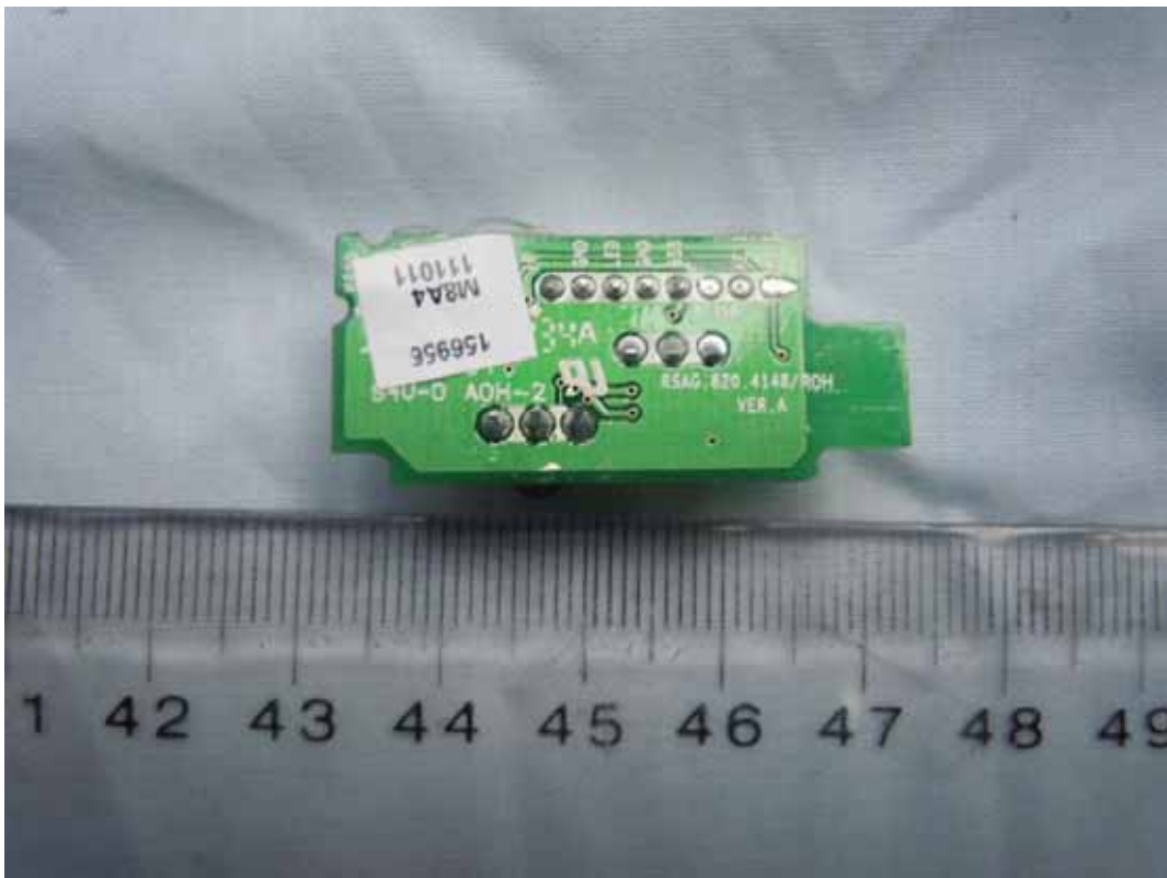
FIGURE 14 LED LCD TV (M/N: LTDN55T39XWUS3D) IR BOARD (SOLDERED SIDE)
