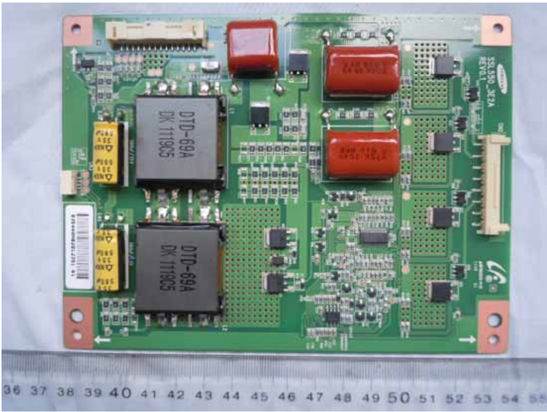
FIGURE 17 LED LCD TV (M/N: LTDN55T39XWUS3D) HIGH VOLTAGE SIGNAL BOARD (COMPONENT SIDE)
