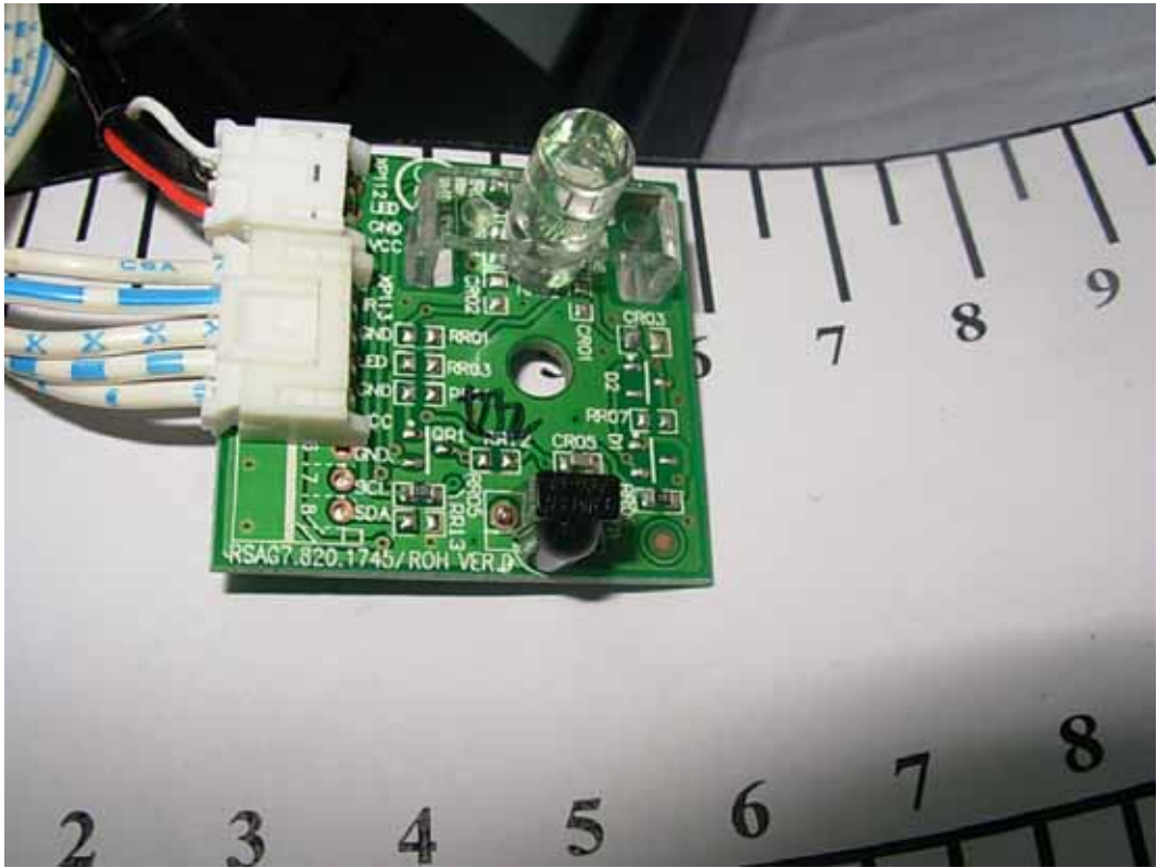
FIGURE 8 LCD TV (M/N: LTDN55T57XUS) LED BOARD (COMPONENT SIDE)
