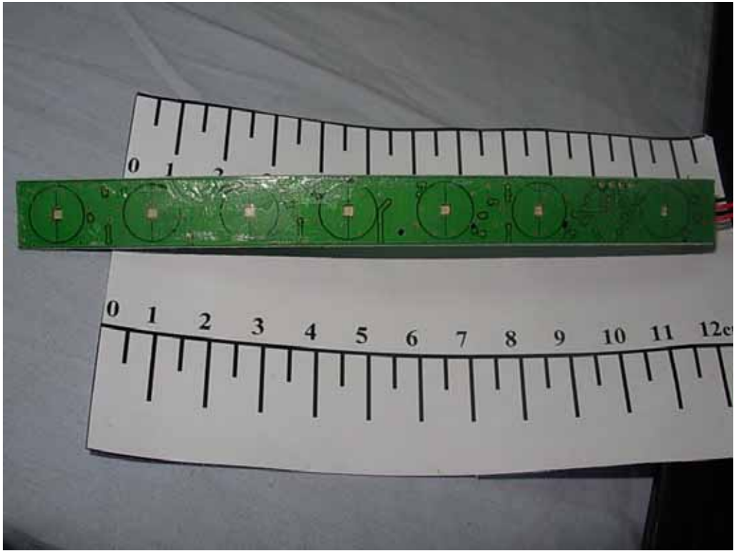
FIGURE 7 LCD TV (M/N: LTDN55T57XUS) KEY BOARD (SOLDERED SIDE)
