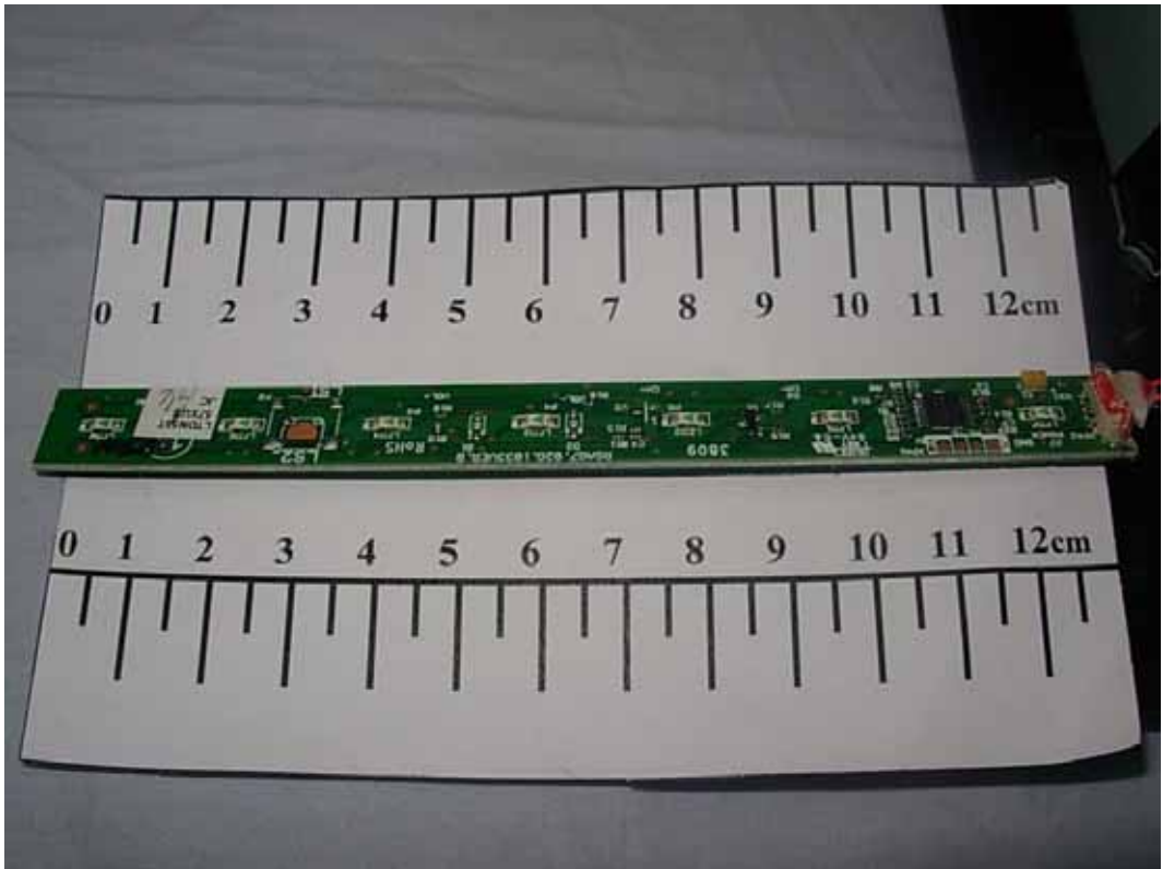
FIGURE 6 LCD TV (M/N: LTDN55T57XUS) KEY BOARD (COMPONENT SIDE)
