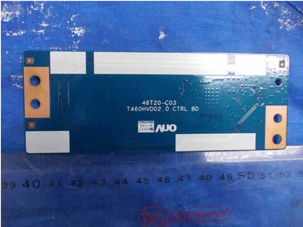
FIGURE 12 LED LCD TV (M/N: 46K360MN) LCD PANEL BOARD (SOLDERED SIDE)
