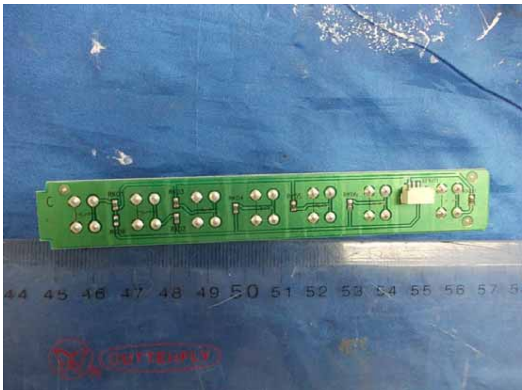
FIGURE 10 LED LCD TV (M/N: 46K360MN) KEY BOARD (SOLDERED SIDE)
