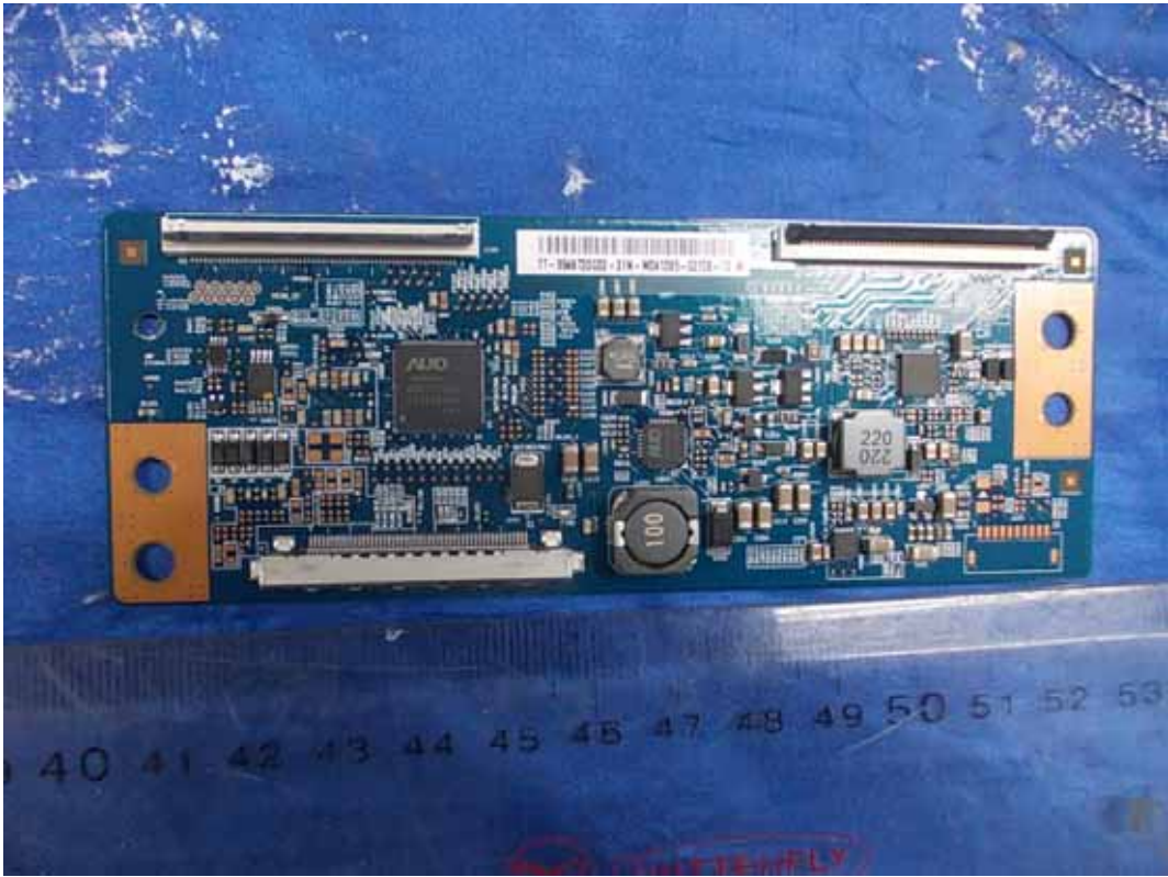
FIGURE 11 LED LCD TV (M/N: 46K360MN) LCD PANEL BOARD (COMPONENT SIDE)
