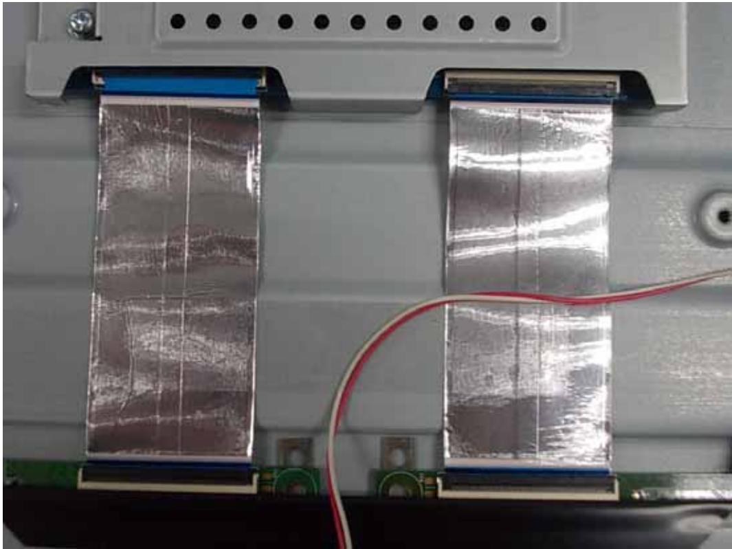
FIGURE 20 LED LCD TV (M/N: 46K366W) DEBUG 3
