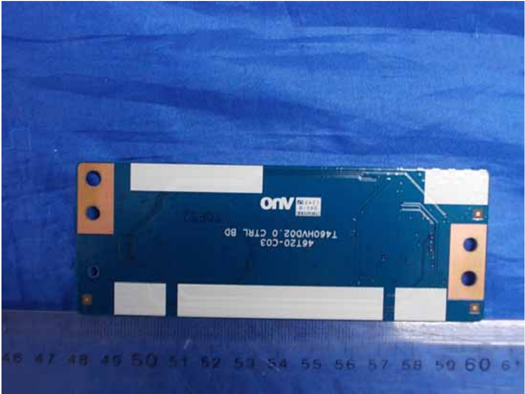
FIGURE 17 LED LCD TV (M/N: 46K366W) SIGNAL BOARD (SOLDERED SIDE)
