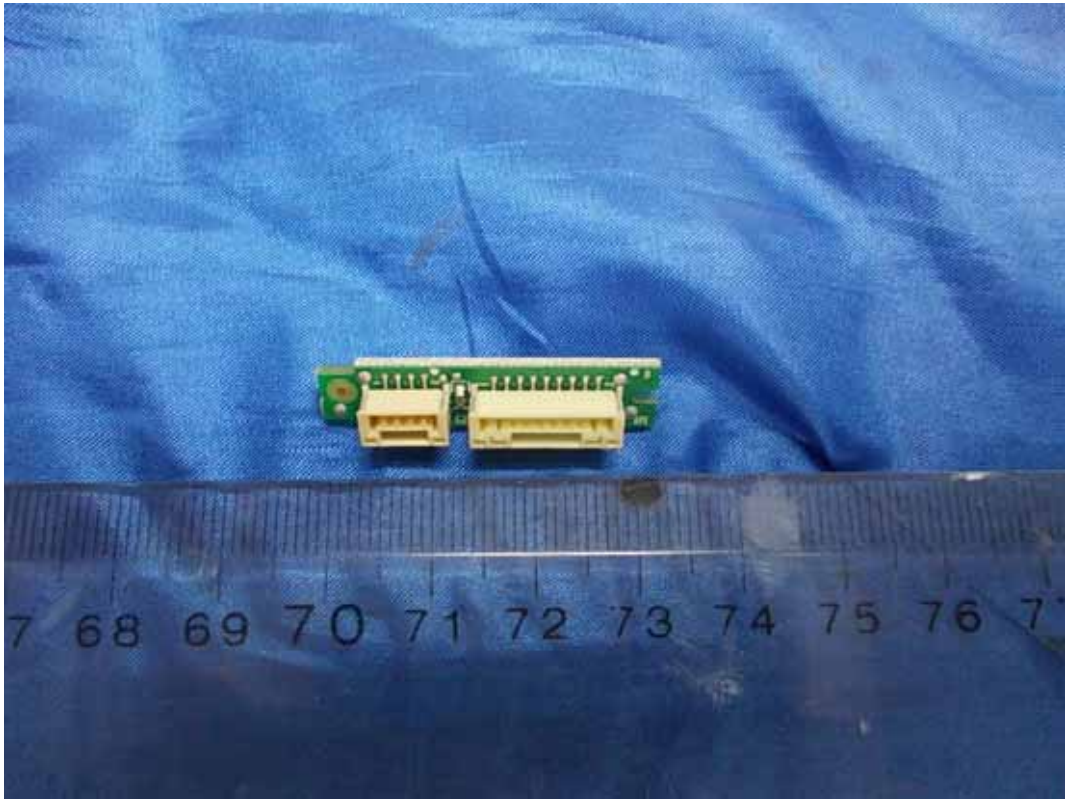
FIGURE 14 LED LCD TV (M/N: 46K366W) IR BOARD (COMPONENT SIDE)
