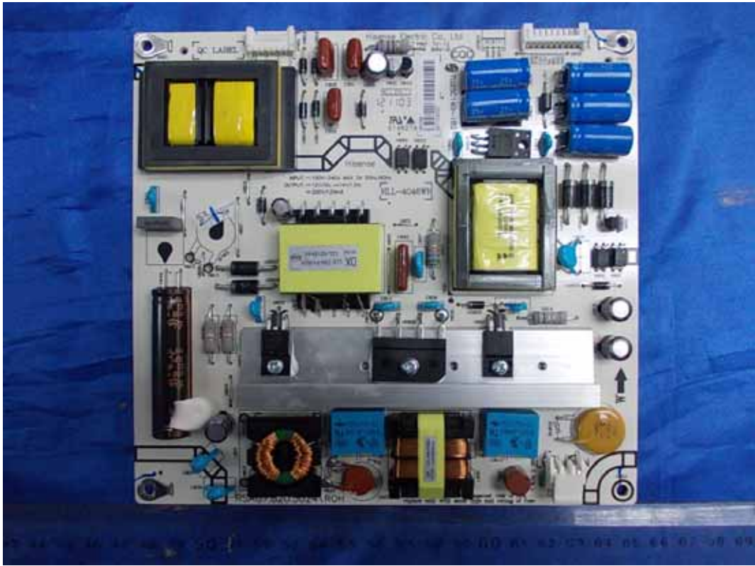
FIGURE 3 LED LCD TV (M/N: LTDN46K360MUS) POWER BOARD (COMPONENT SIDE)
