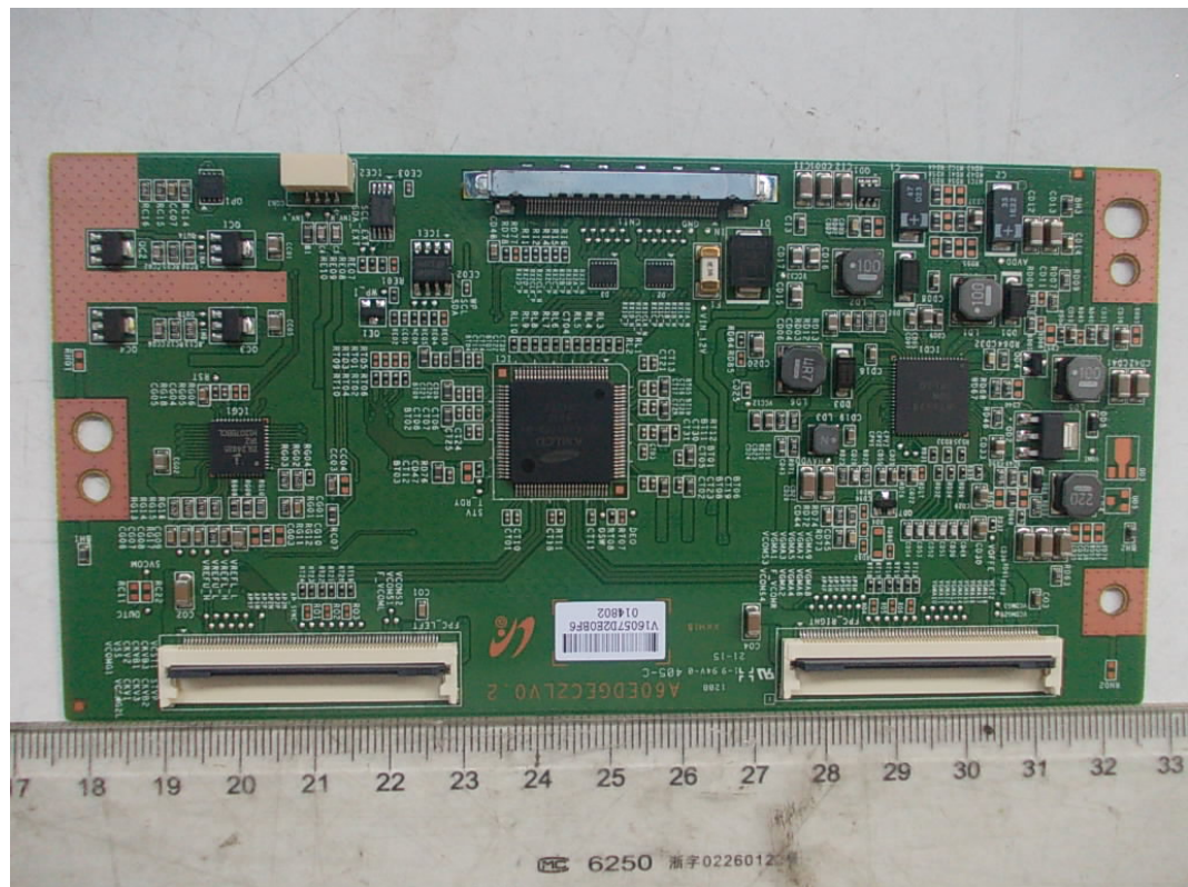
FIGURE 11 LED LCD TV (M/N: LTDN46K20US) LCD PANEL CONTROL BOARD (COMPONENT SIDE)
