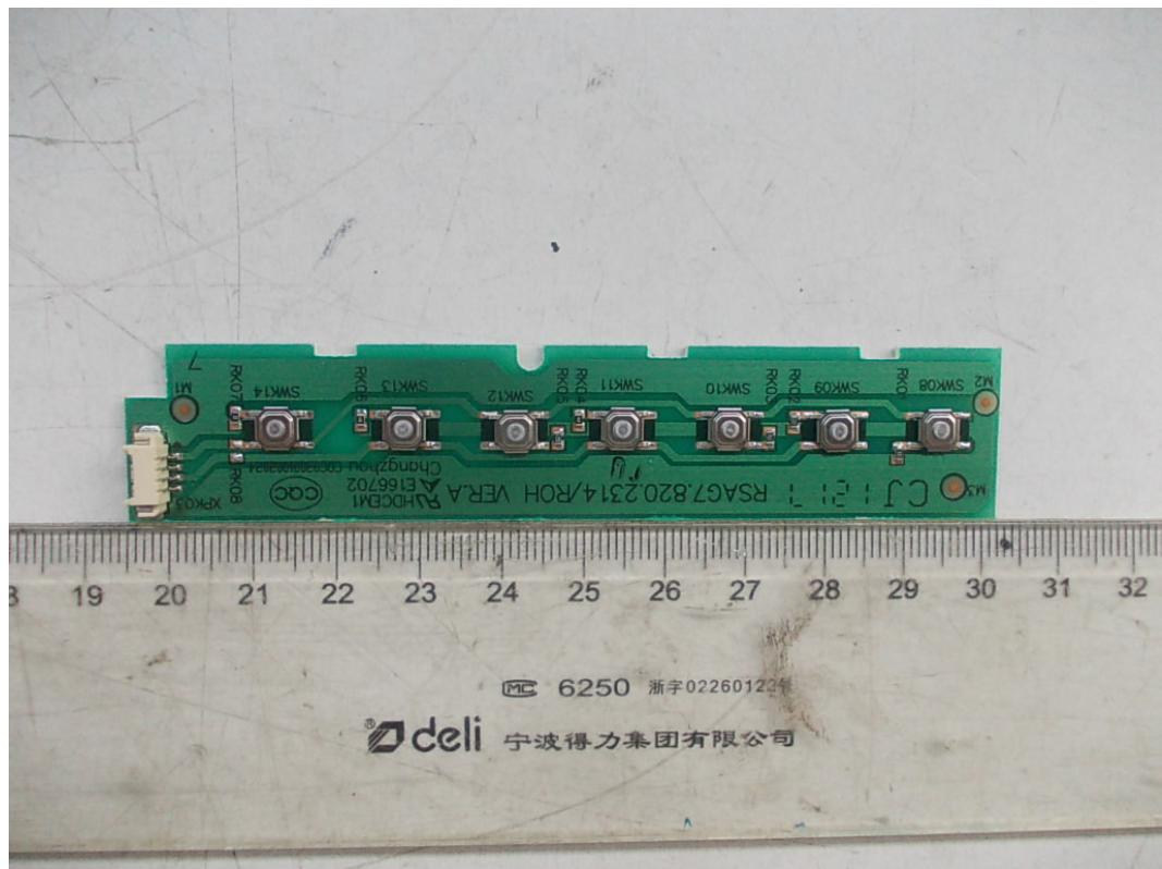
FIGURE 9 LED LCD TV (M/N: LTDN46K20US) KEY BOARD (COMPONENT SIDE)
