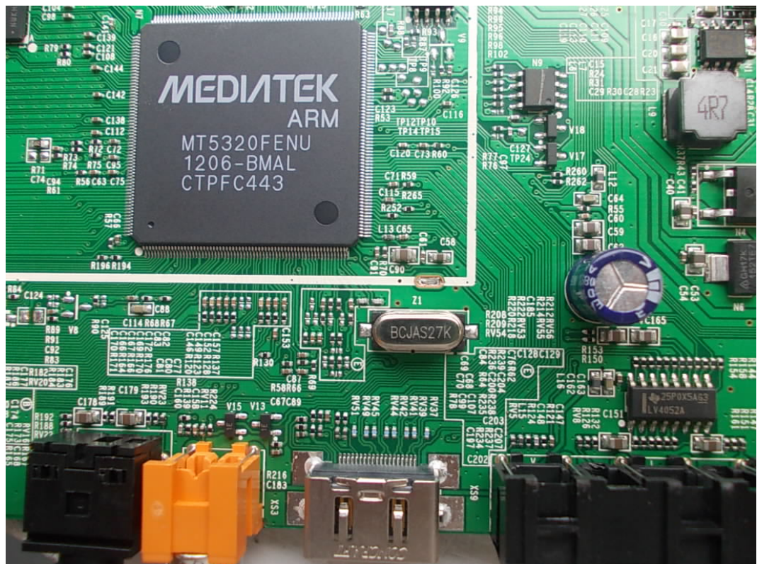
FIGURE 8 LED LCD TV (M/N: LTDN46K20US) CHIP & CRYSTAL ON MAIN BOARD
