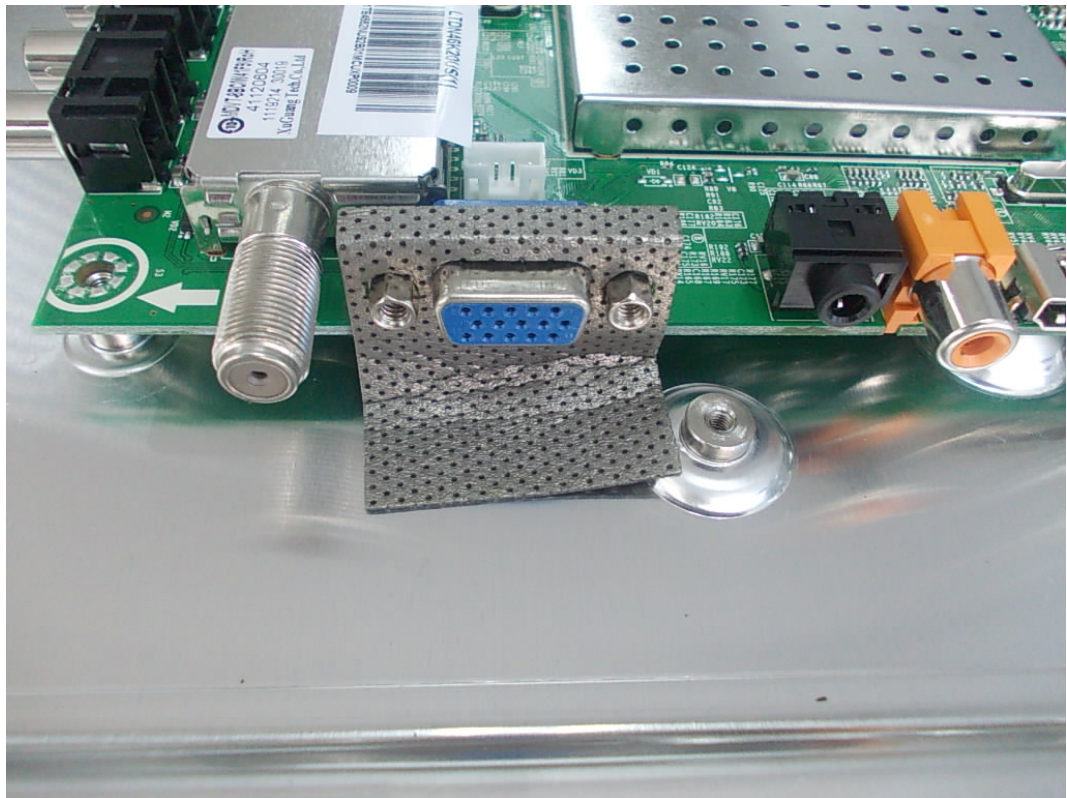
FIGURE 17 LED LCD TV (M/N: LTDN46K20US) DEBUG 3
