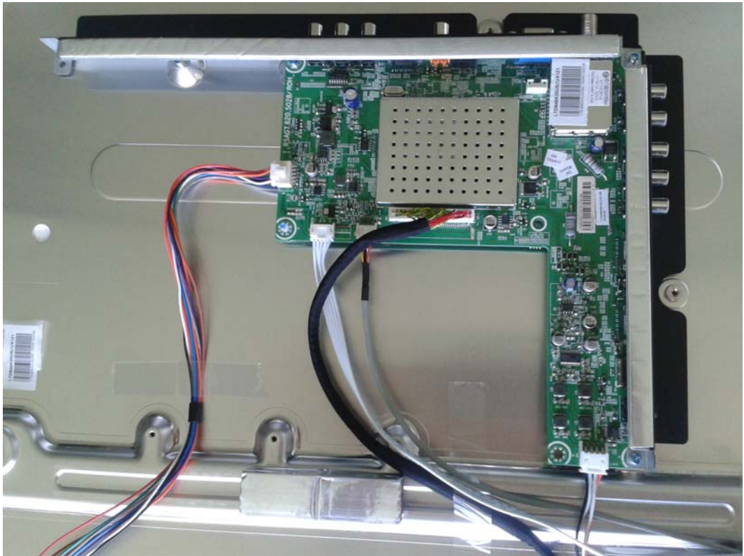
FIGURE 15 LED LCD TV (M/N: LTDN46K20US) DEBUG 1
