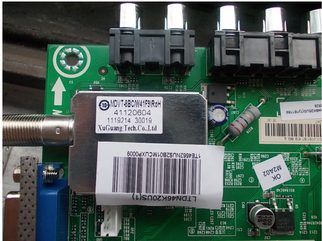
FIGURE 7 LED LCD TV (M/N: LTDN46K20US) TUNER ON MAIN BOARD
