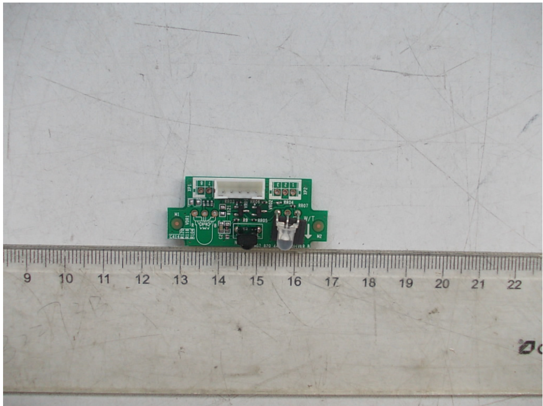
FIGURE 13 LED LCD TV (M/N: LTDN46K20US) IR BOARD (COMPONENT SIDE)
