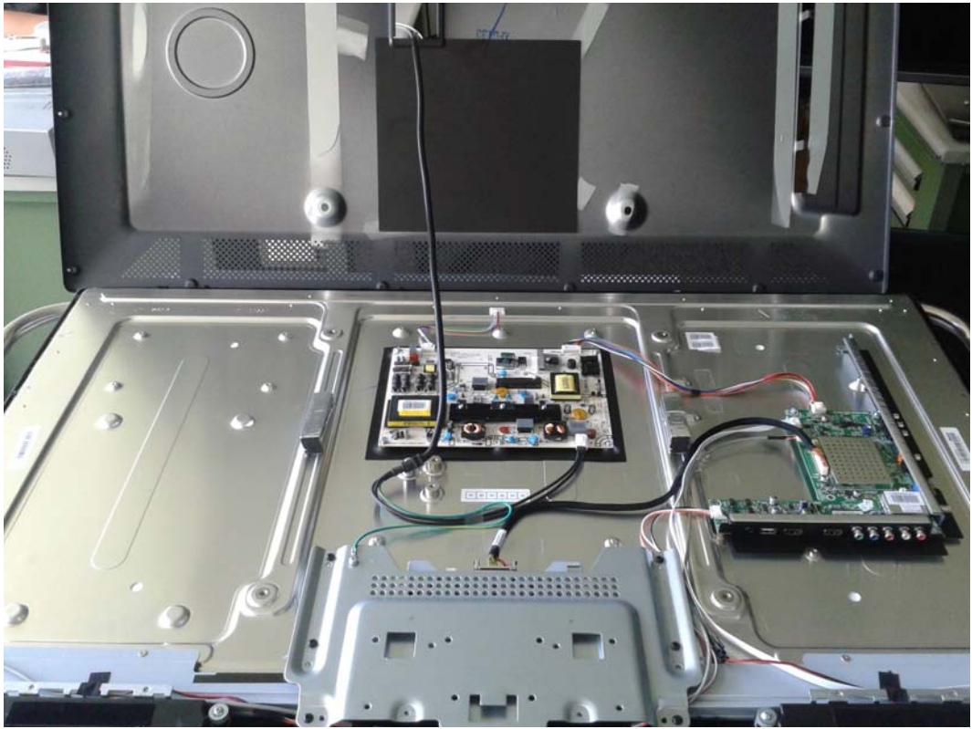
FIGURE 1 LED LCD TV (M/N: LTDN46K20US) COVER REMOVED
