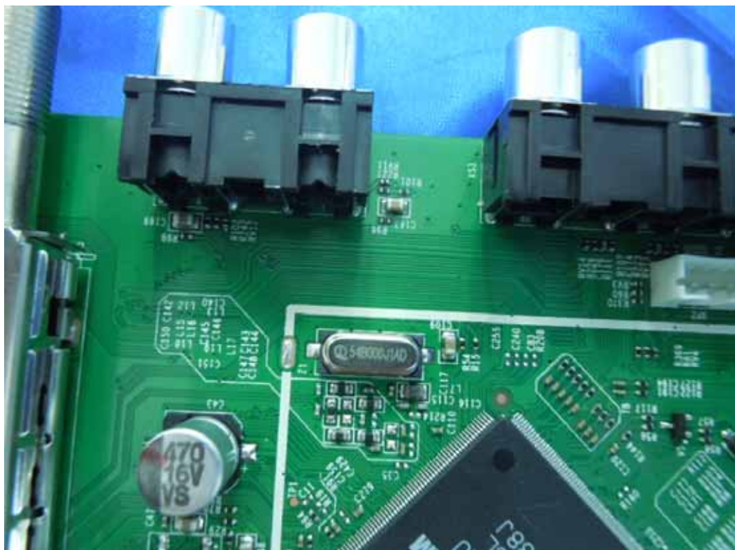
FIGURE 8 LED LCD TV (M/N: LTDN46K20US) CRYSTAL ON MAIN BOARD
