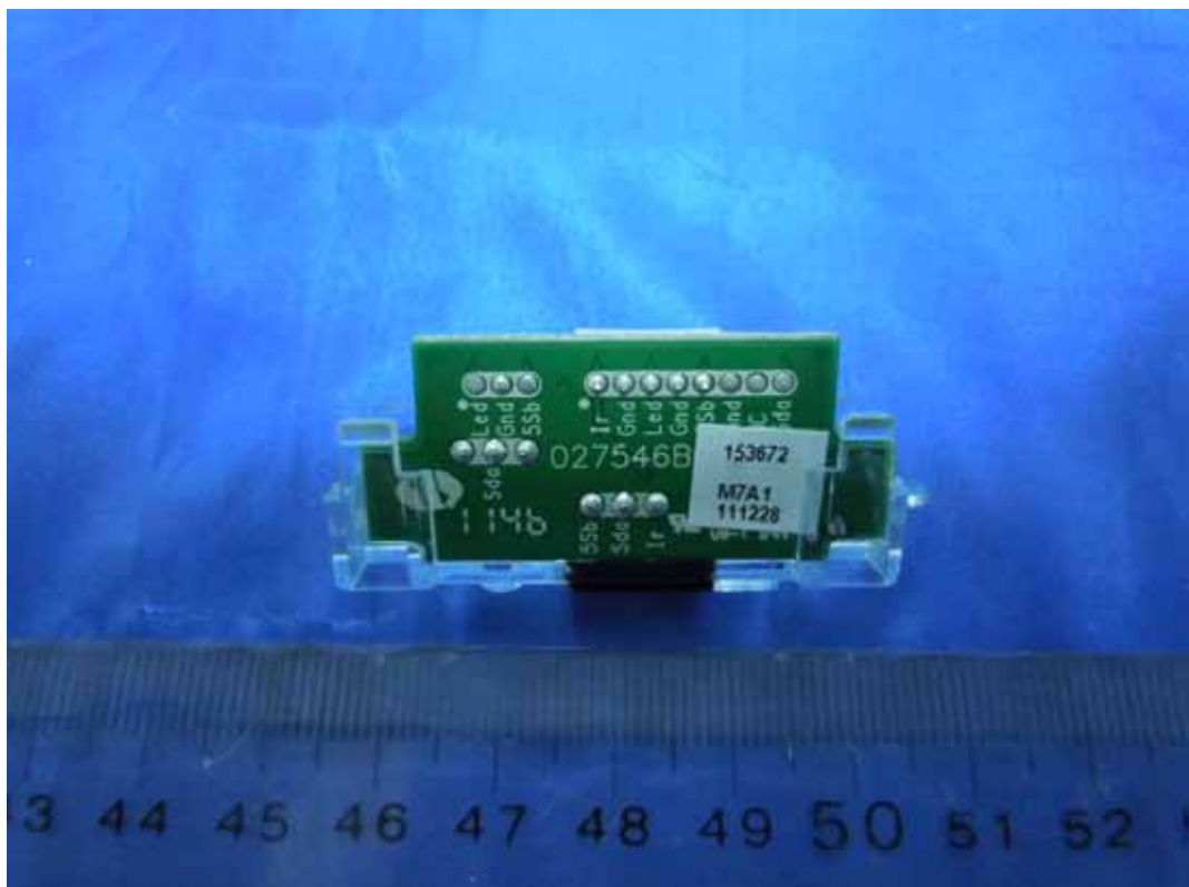
FIGURE 13 LED LCD TV (M/N: LTDN46K20US) IR BOARD (SOLDERED SIDE)
