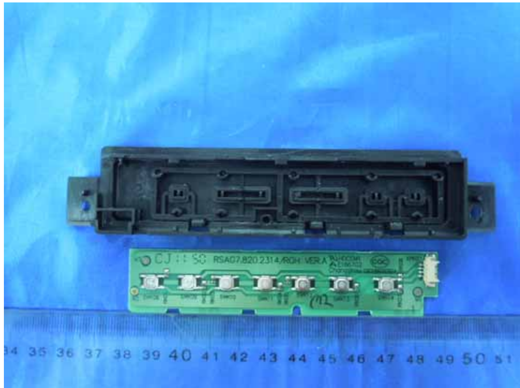
FIGURE 10 LED LCD TV (M/N: LTDN46K20US) KEY BOARD (COMPONENT SIDE)
