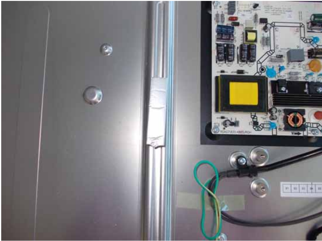
FIGURE 16 LED LCD TV (M/N: LTDN46K20US) DEBUG 1
