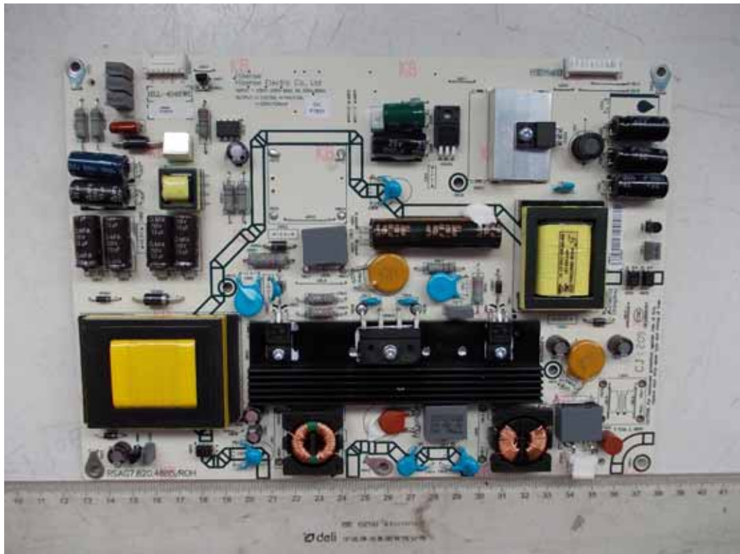
FIGURE 3 LED LCD TV (M/N: LTDN46K20US) POWER BOARD (COMPONENT SIDE)
