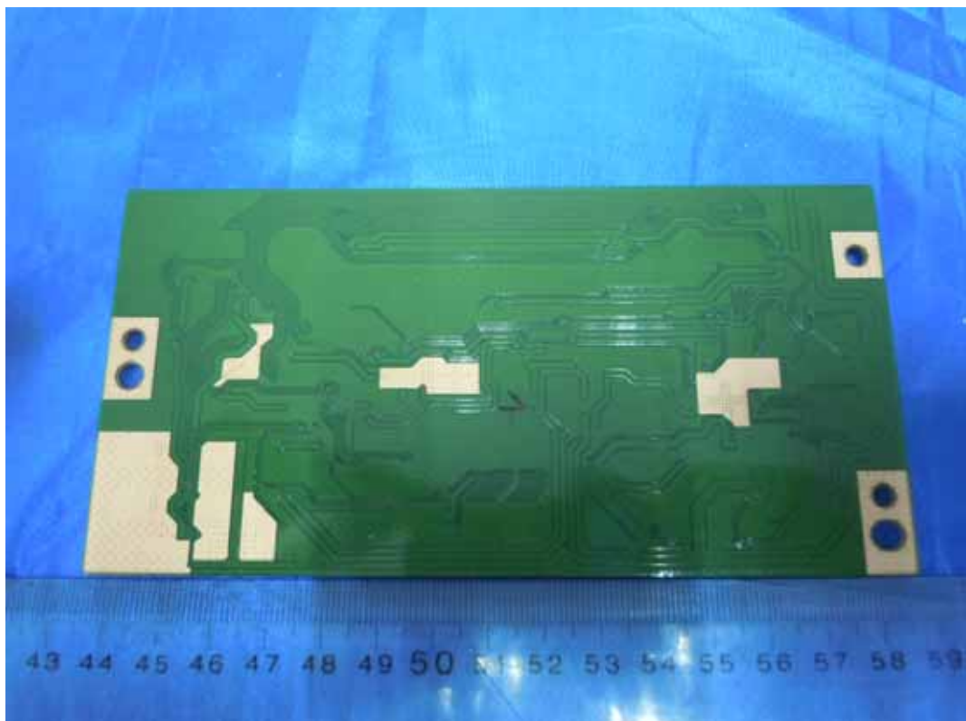
FIGURE 15 LED LCD TV (M/N: LTDN46K20US) PANEL BOARD (SOLDERED SIDE)
