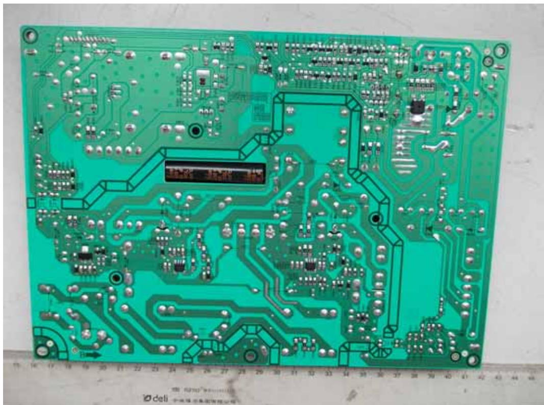
FIGURE 4 LED LCD TV (M/N: LTDN46K20US) POWER BOARD (SOLDERED SIDE)
