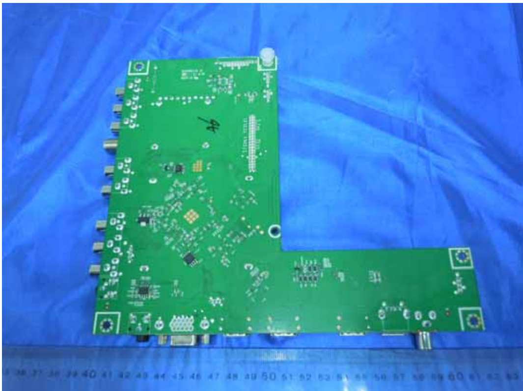
FIGURE 6 LED LCD TV (M/N: LTDN46K20US) MAIN BOARD (SOLDERED SIDE)
