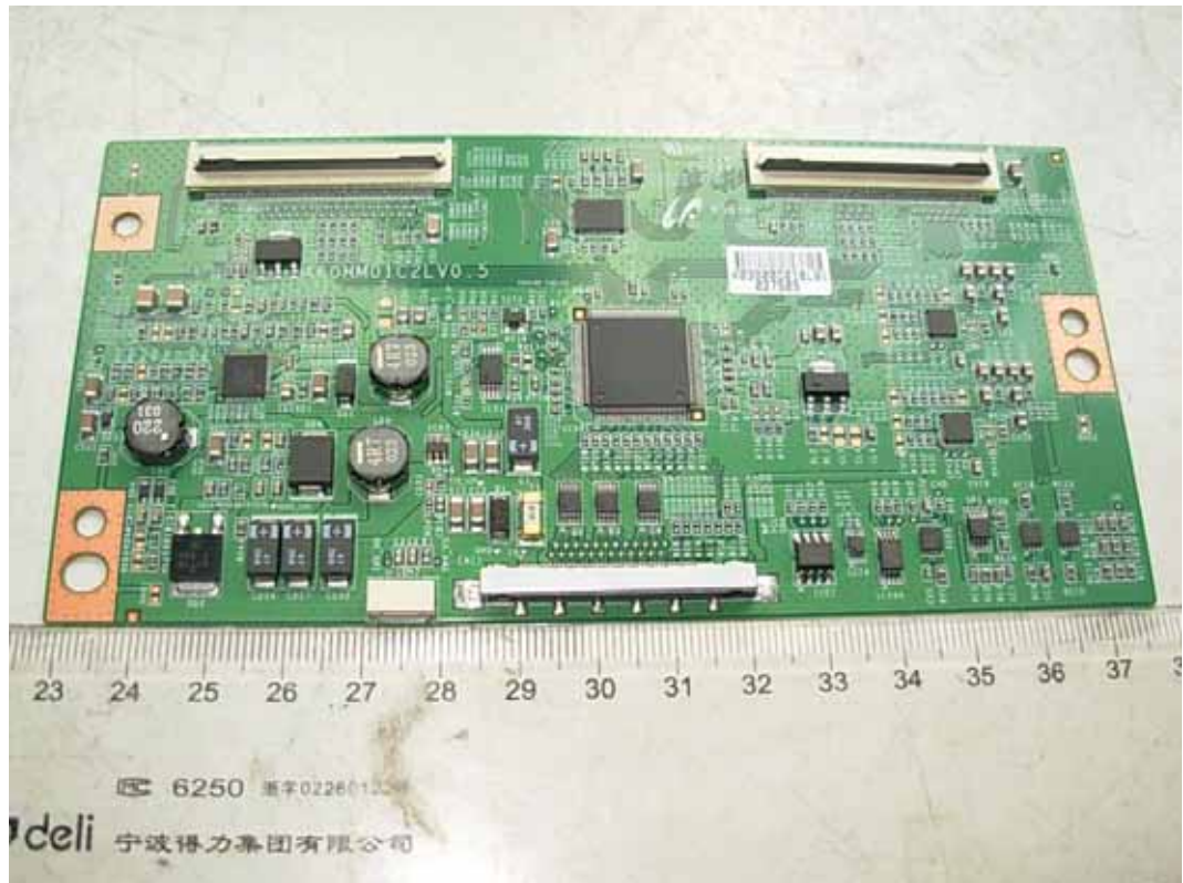
FIGURE 13 LCD TV (M/N: LTDN46K15US) DISPLAY BOARD (COMPONENT SIDE)
