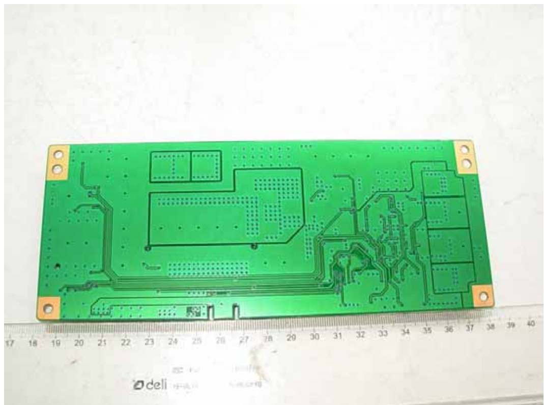
FIGURE 16 LCD TV (M/N: LTDN46K15US) HIGH VOLTAGE SIGNAL BOARD (SOLDERED SIDE)
