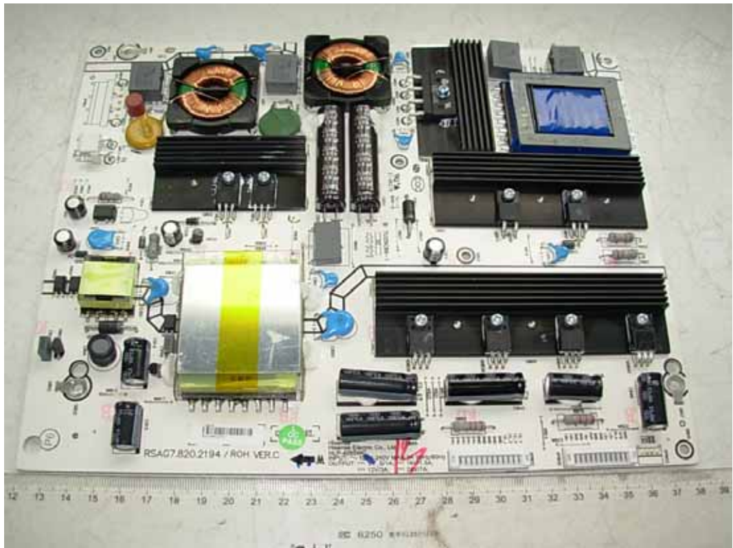
FIGURE 3 LCD TV (M/N: LTDN46K15US) POWER BOARD (COMPONENT SIDE)
