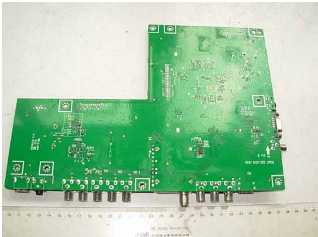
FIGURE 6 LCD TV (M/N: LTDN46K15US) MAIN BOARD (SOLDERED SIDE)
